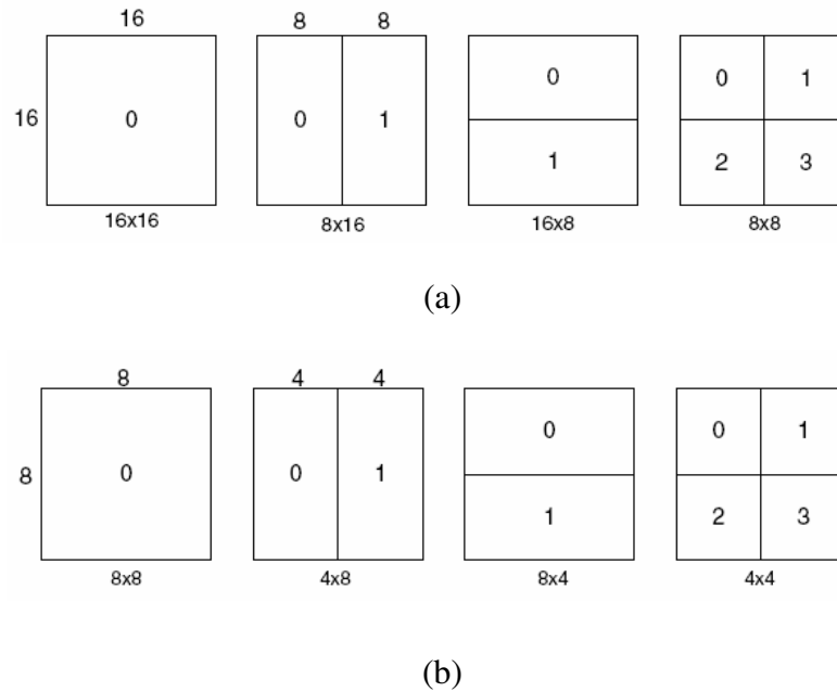
Figure 2.3: (a) Macroblock partitions: 16x16, 8x16, 16x8, 8x8, (b) Sub-macroblock partitions: 8x8, 4x8, 8x4, 4x4
