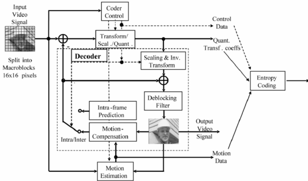
Figure 2.5: Block Diagram of encoding process in the VCL of H.264/AVC [1]
