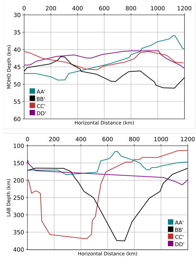
Figure 3.26 : MOHO and LAB depth vs. horizontal distance (cross sections taken from MOHO and LAB maps).
