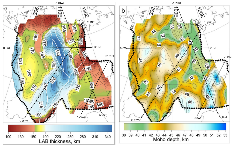
Figure 3.25 : MOHO and LAB depths (modified after Cherepanova & Artemieva, 2015).
