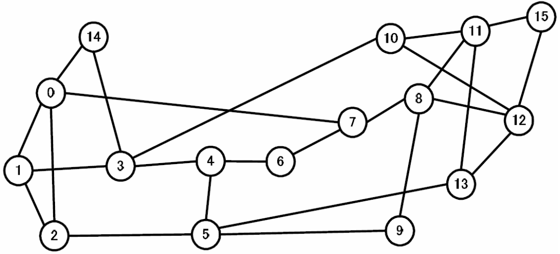
Figure 5.2: NSFNET Topology Used in Simulations
