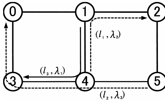
Figure 4.3: New Lightpaths on the Physical Network
