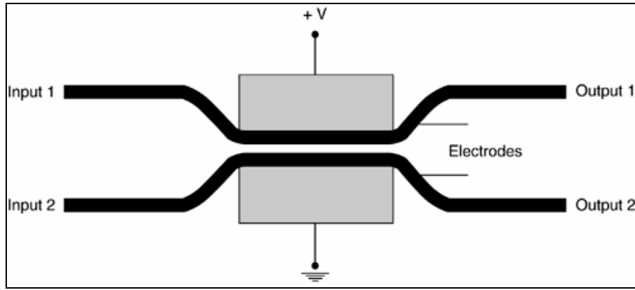
Figure 2.4: A Simple 2 \times 2 Switch (Coupler)
