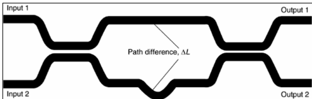
Figure 2.7: Mach-Zehnder Interferometer
