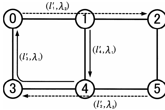
Figure 4.2: Old Lightpaths on the Physical Network
