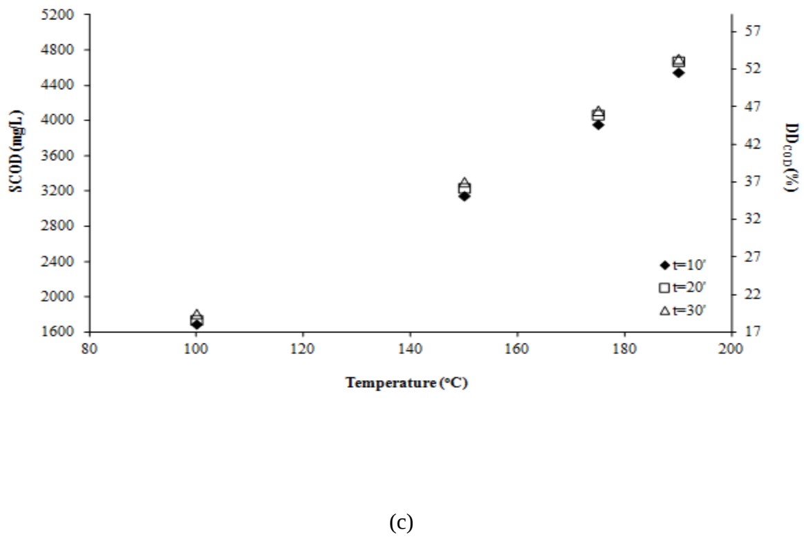
Figure 4.2 (continuity): Effect of microwave pretreatment on sludge solubilization – Sample 1: (b) 1.13% and (c) 2.26% TS concentration.
