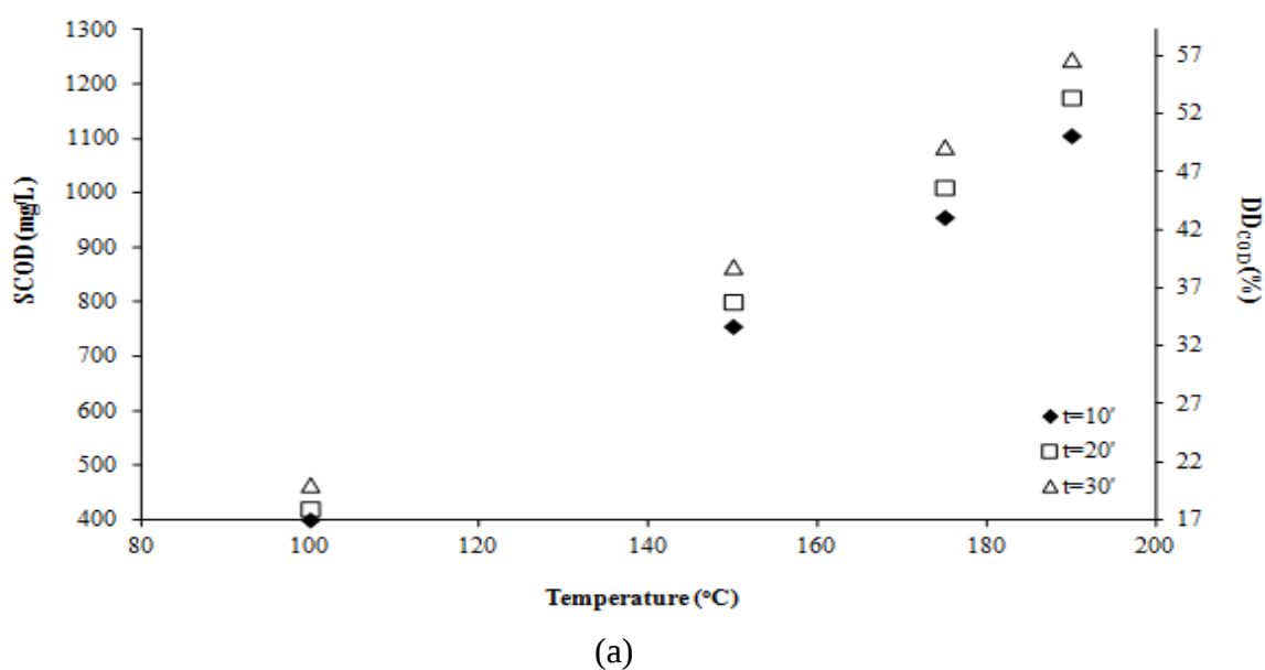
Figure 4.2: Effect of microwave pretreatment on sludge solubilization – Sample 1:(a) 0.57%
