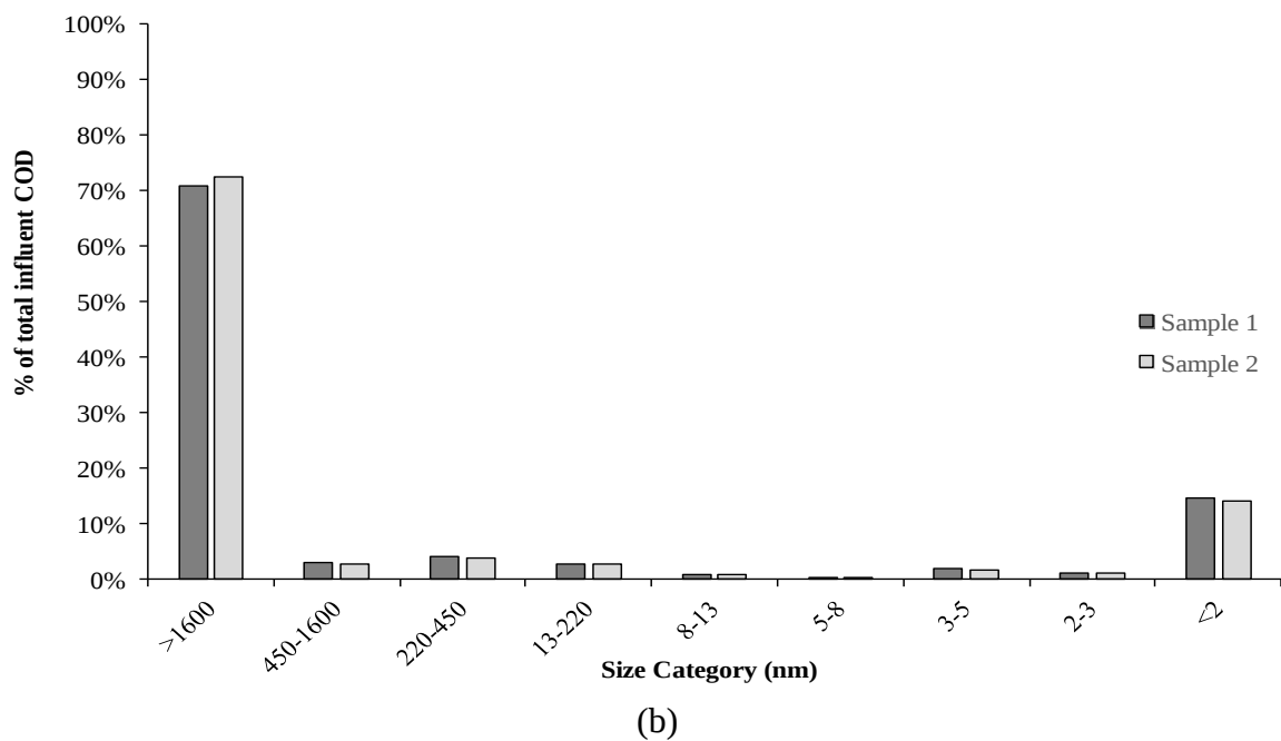
Figure 4.3: Impact of sludge disintegration on the PSD-based COD fractionation: (a) sonication E_s=5000 kJ/kg TS, (b) sonication E_s=30000 kJ/kg TS.
