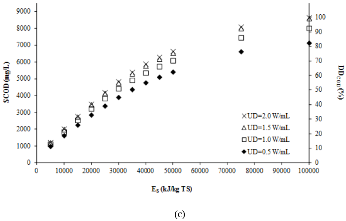
Figure 4.1 (contunity): Effect of ultrasonic pretreatment on sludge solubilization – Sample 1: (c) 2.26% TS concentration.
