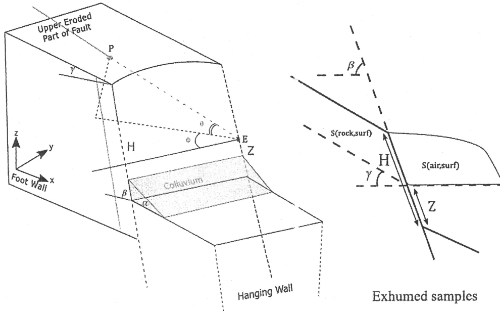
Figure 3.7: Exhumed samples receive cosmic rays going through the both air and through the rock (Modified after Scalaginhauf et.al, 2010).
