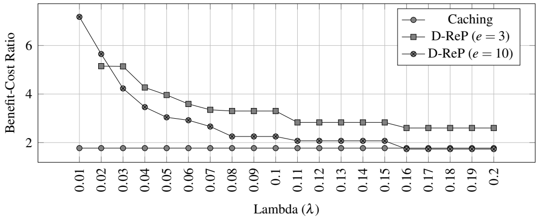
Figure 5.9 : Benefit-cost ratio with variable \lambda .
