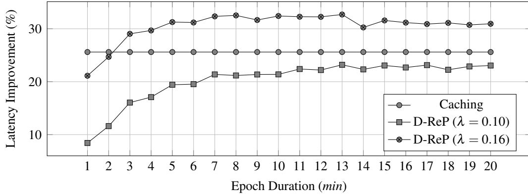
Figure 5.6 : Latency improvement rate with variable epoch duration.
