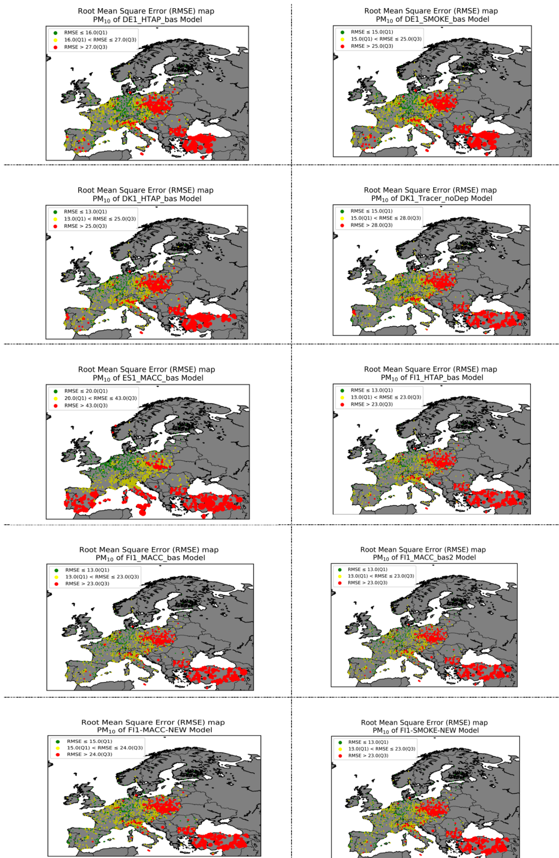
Figure B.10: RMSE maps.
