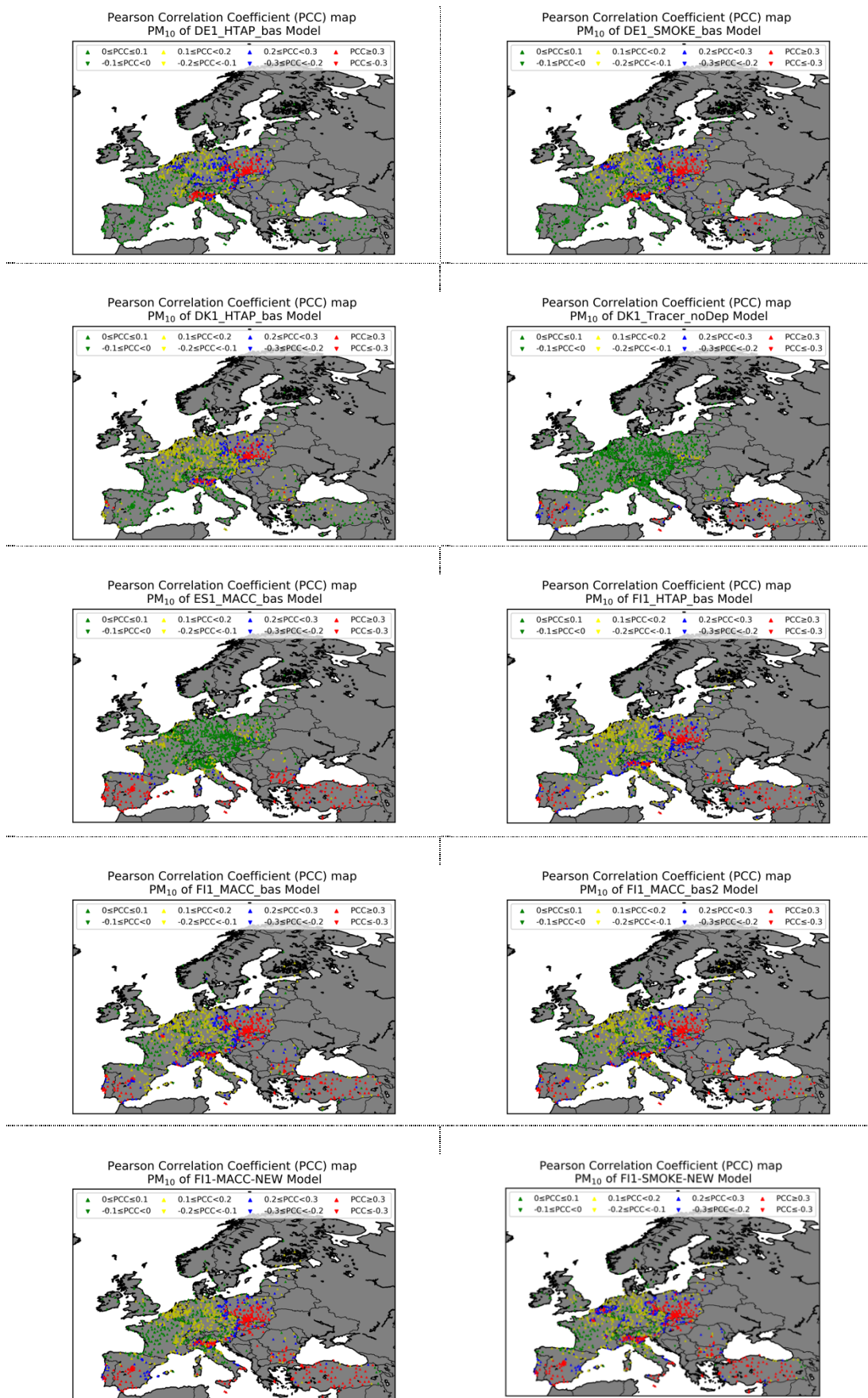
Figure B.8 : PCC maps.
