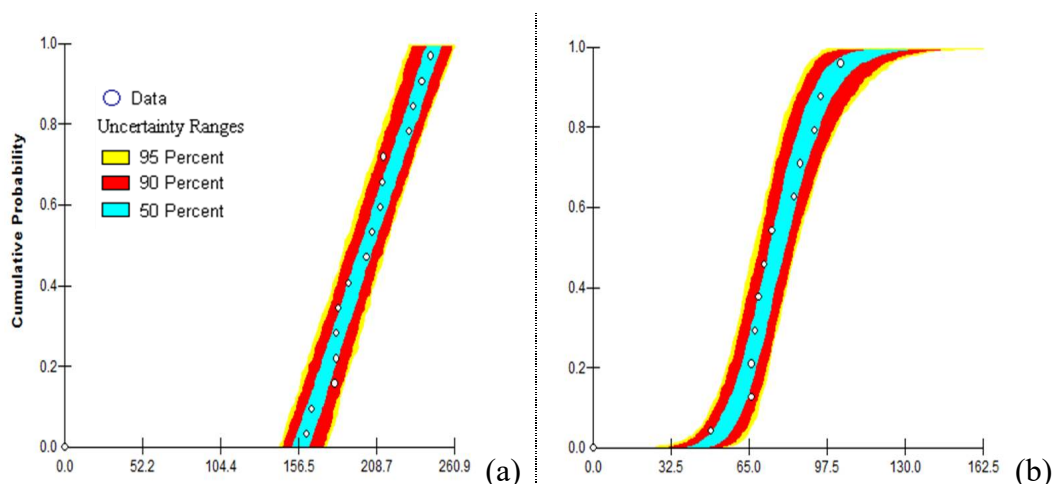
Figure 3.18 : Probability band of NO 2 EFs for “1A1a-10101-3.10” as cumulative distribution of (a)Uniform distribution fitted to NO 2 EFs derived from in-situ measurements (b)Gamma distribution fitted to NO 2 EFs derived from EMRs.
