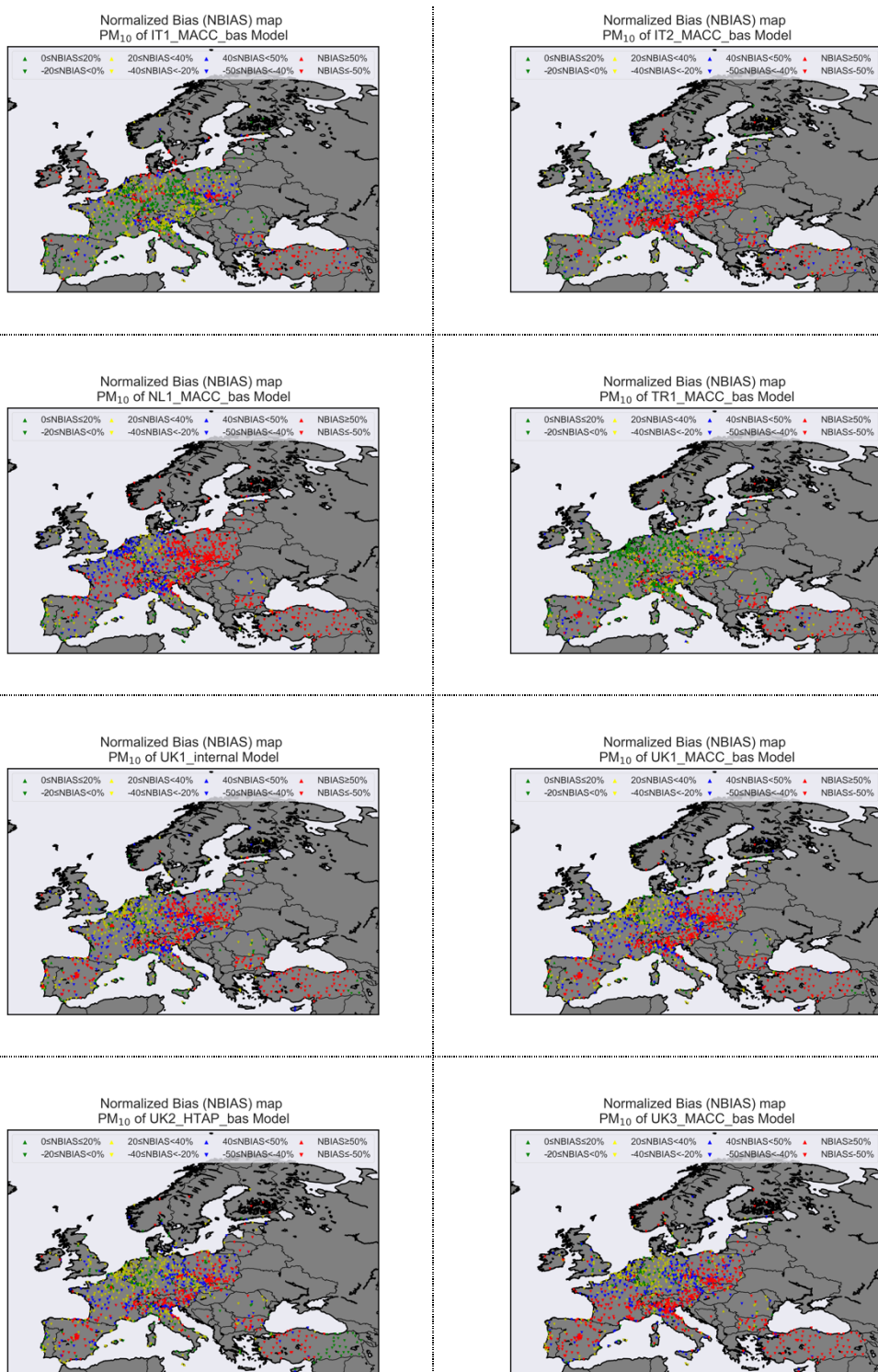
Figure B.6 (continued) : NBIAS maps.
