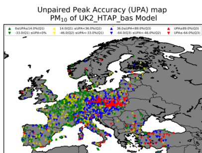
Figure B.11 (continued) : UPA maps.
