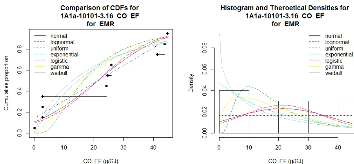
Figure 3.21 : Distribution fitting comparisons of CO EFs on CDF and Histogram for EFs derived from EMRs of “1.A.1.a – 10101 – 3.16”.
