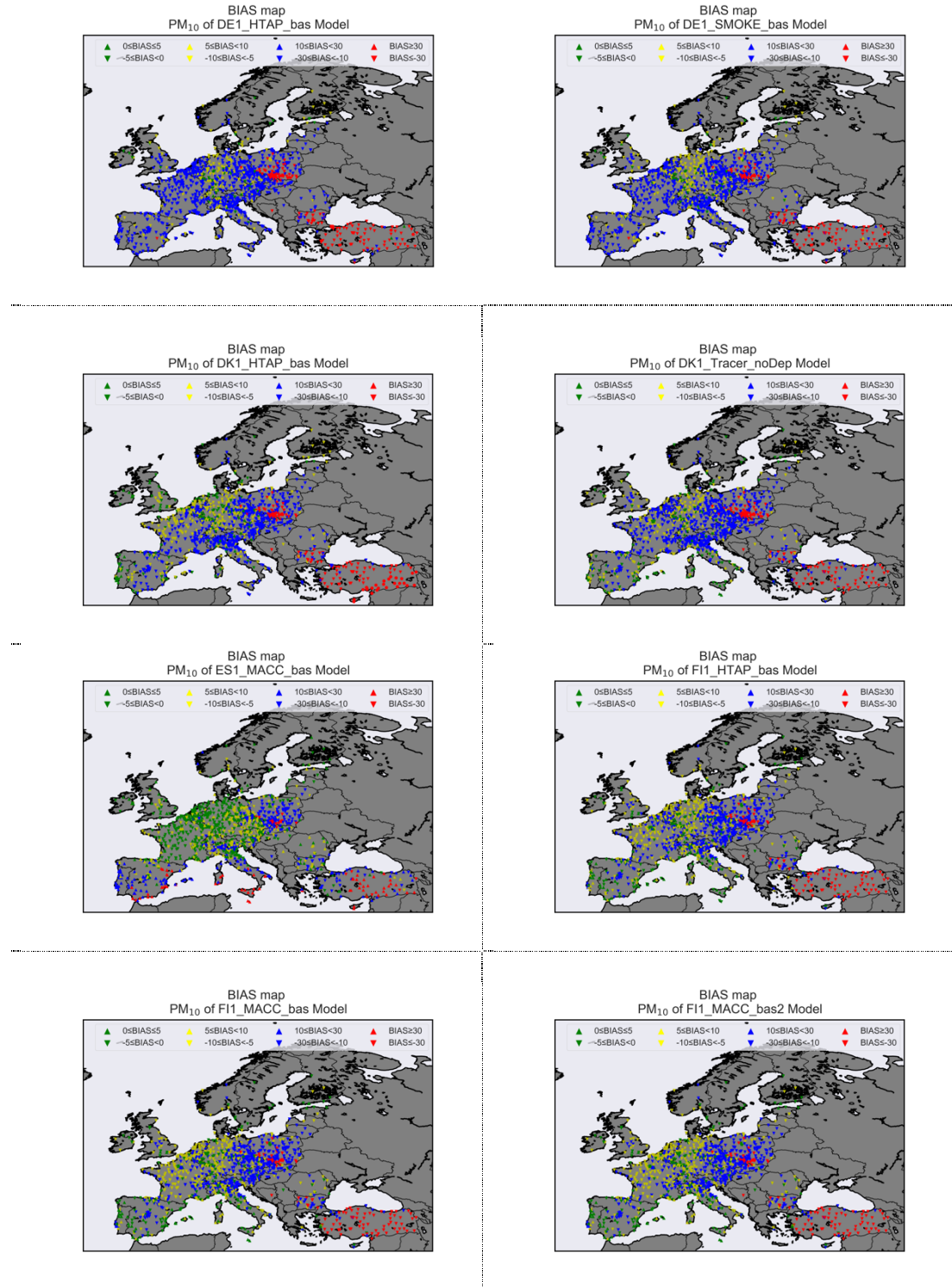
Figure B.1 : BIAS maps.
