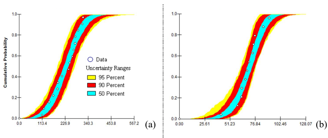
Figure 3.14 : Probability band of SO 2 EFs for “1A1a-10101-3.10” as cumulative distribution of Weibull distribution fitted to SO 2 EFs derived from (a) in-situ measurements (b) EMRs.
