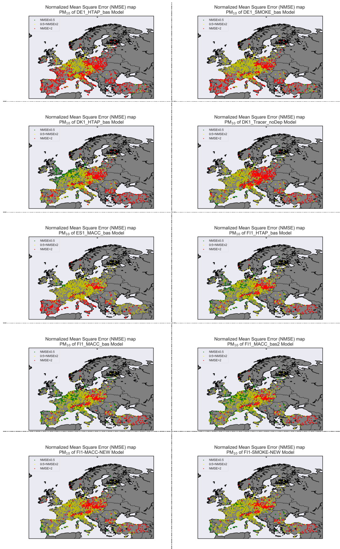
Figure B.7 : NMSE maps.
