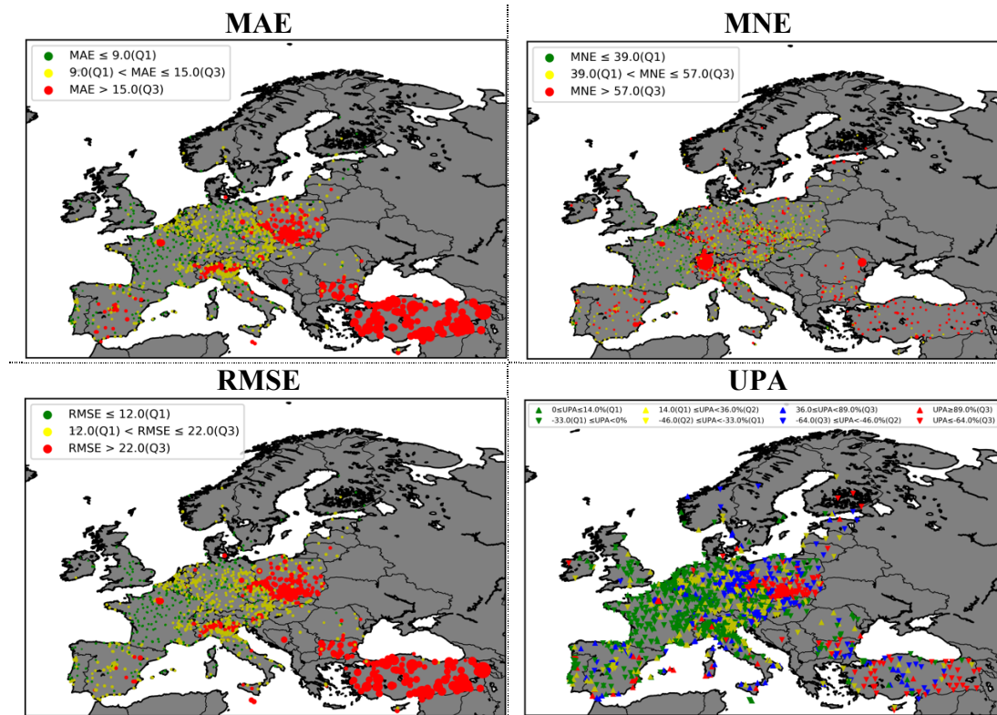
Figure 3.3 : Map of some performance metrics calculated by our group (TR1 model) for \text{PM}_{10} in observation stations throughout Europe for 2010.
