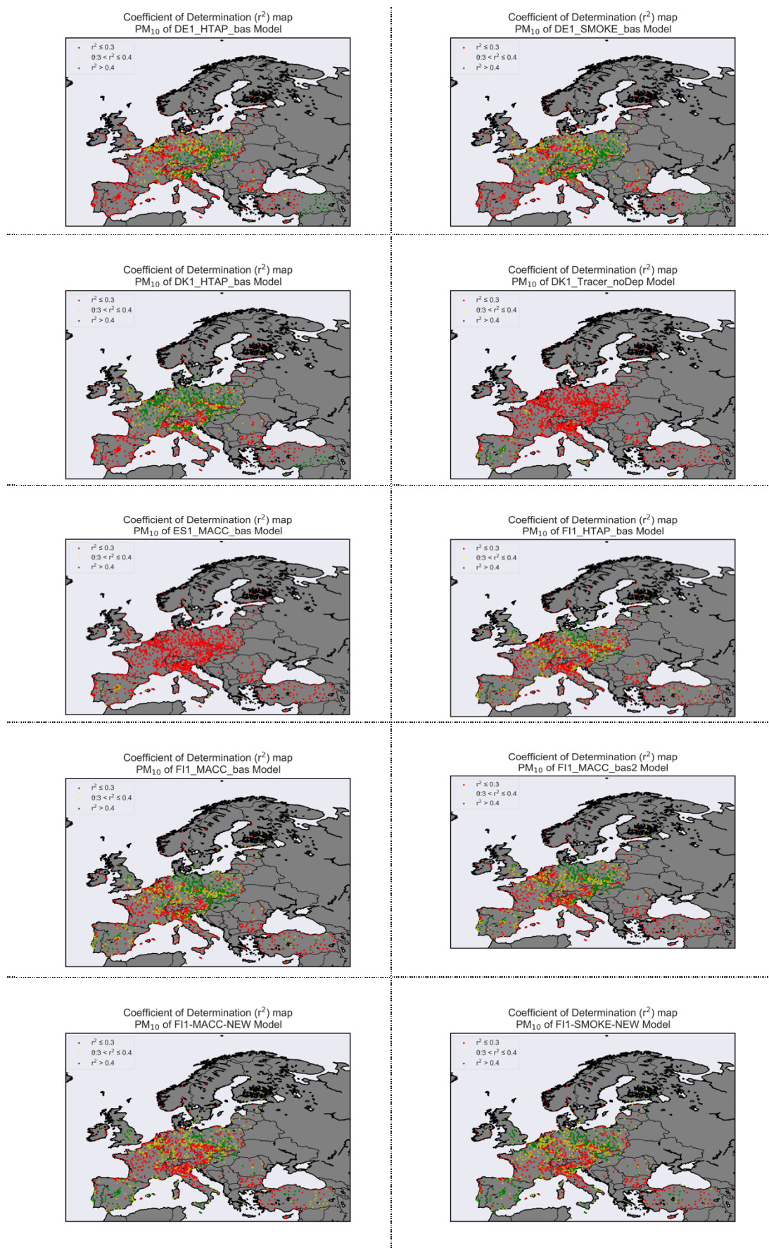
Figure B.9 : r^2 (coefficient of determination) maps.
