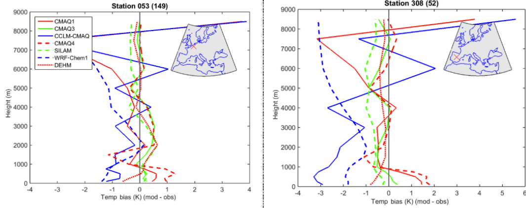
Figure 3.1 : Mean bias (model–observations) for the vertical profiles of temperature measured by ozonesondes launched from indicated locations on the upper right map of each panel.
