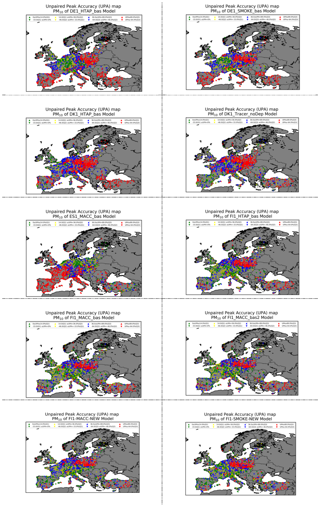
Figure B.11 : UPA maps.
