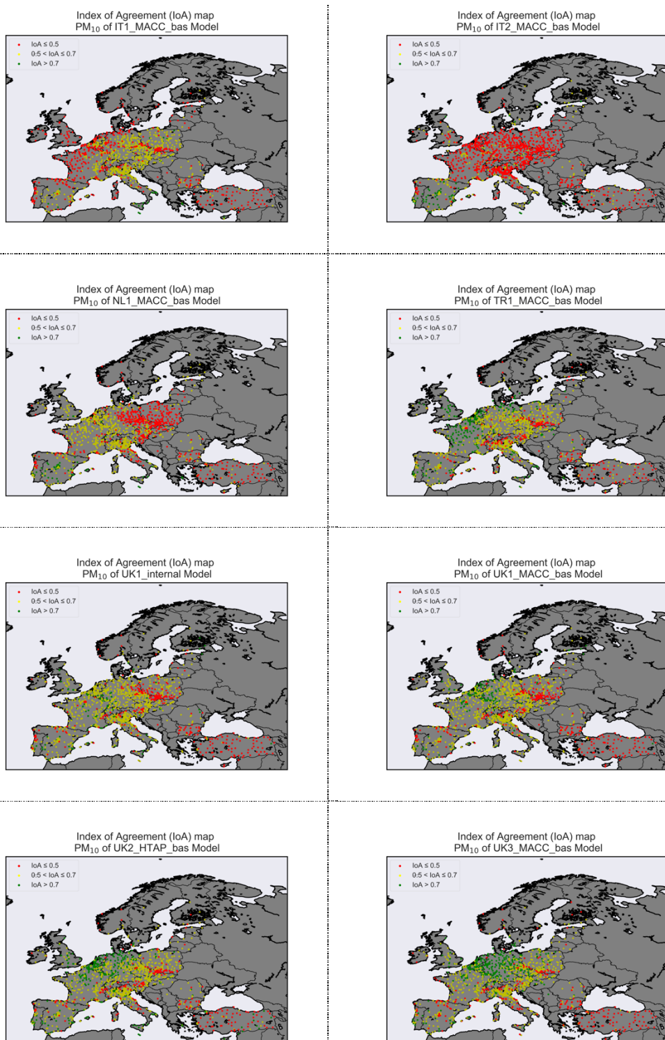
Figure B.2 (continued) : IoA maps.
