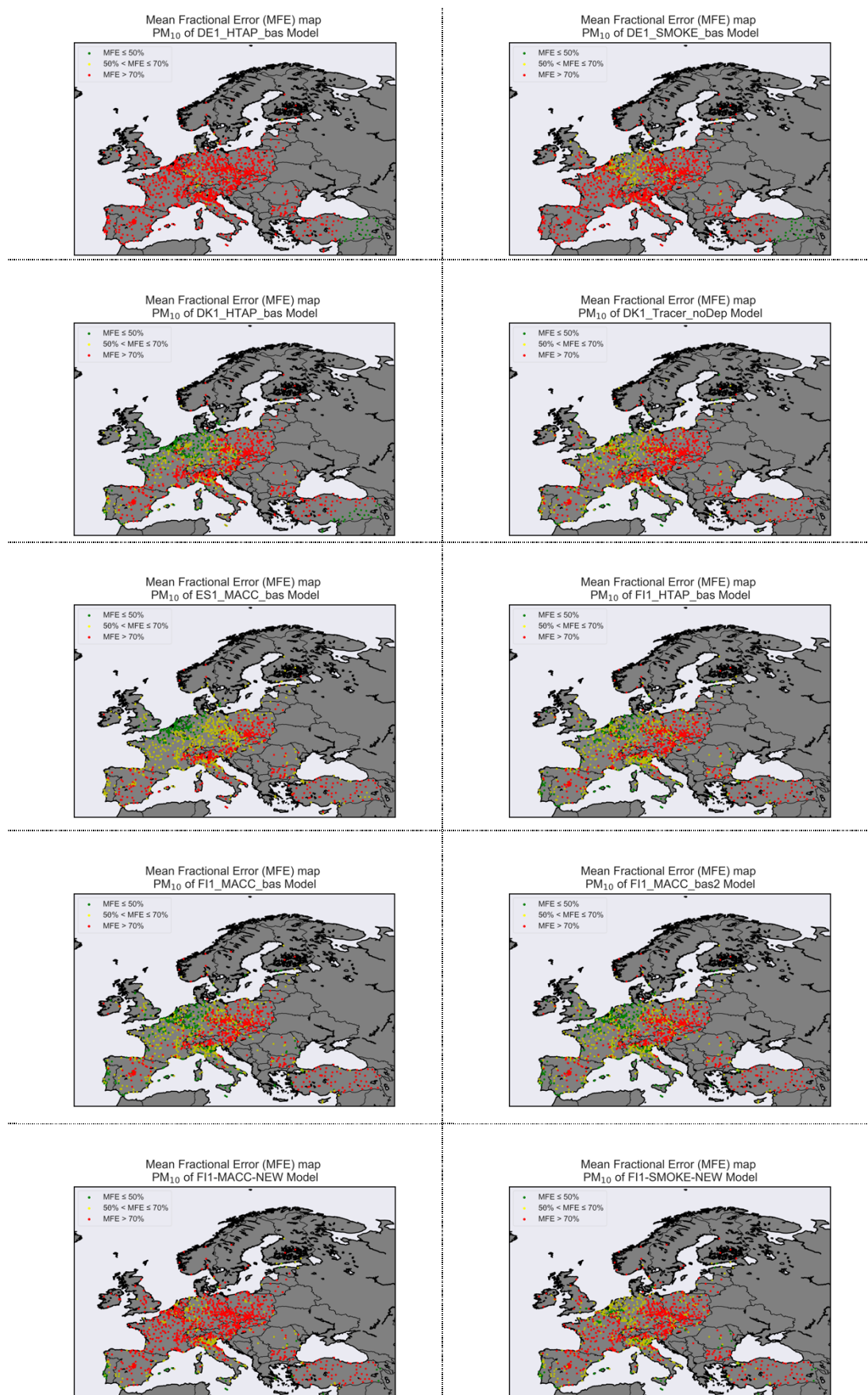
Figure B.4 : MFE maps.
