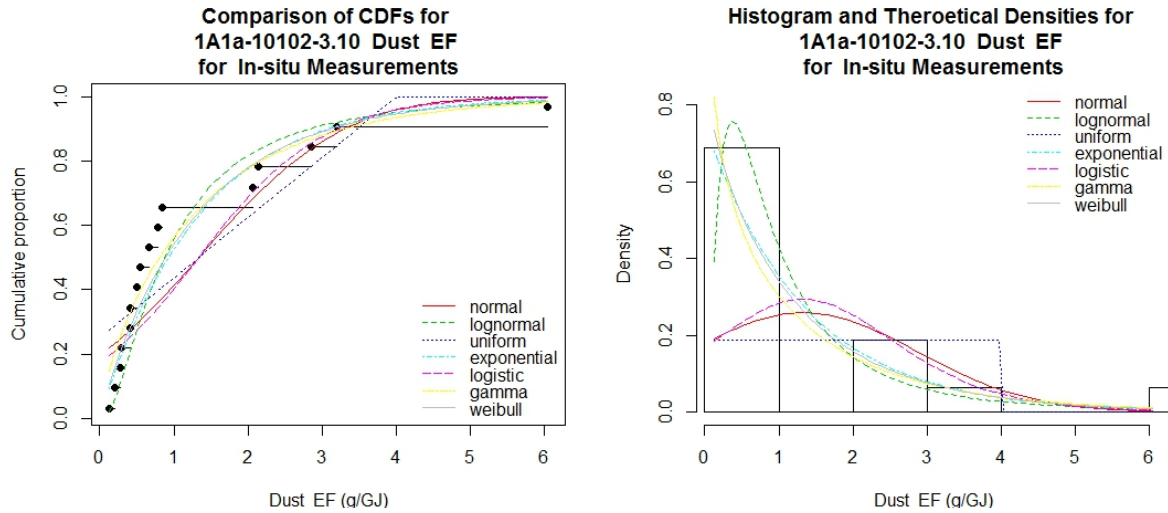
Figure 3.29 : Distribution fitting comparisons of dust EF on CDF and Histogram for in-situ measurements of “1.A.1.a–10102–3.10”.
