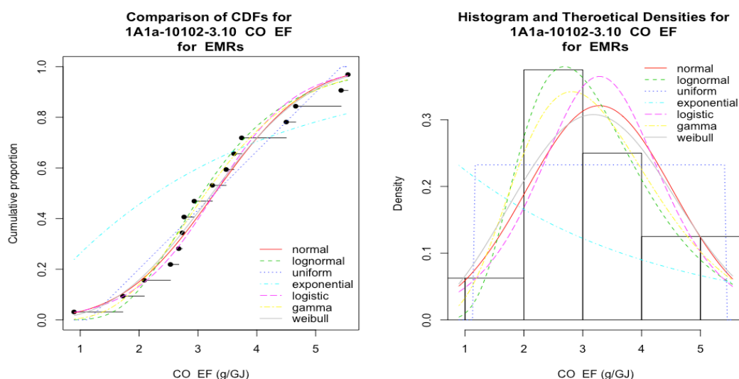
Figure 3.31 : Distribution fitting comparisons of CO EF on CDF and Histogram for in-situ measurements of “1.A.1.a–10102–3.10”.
