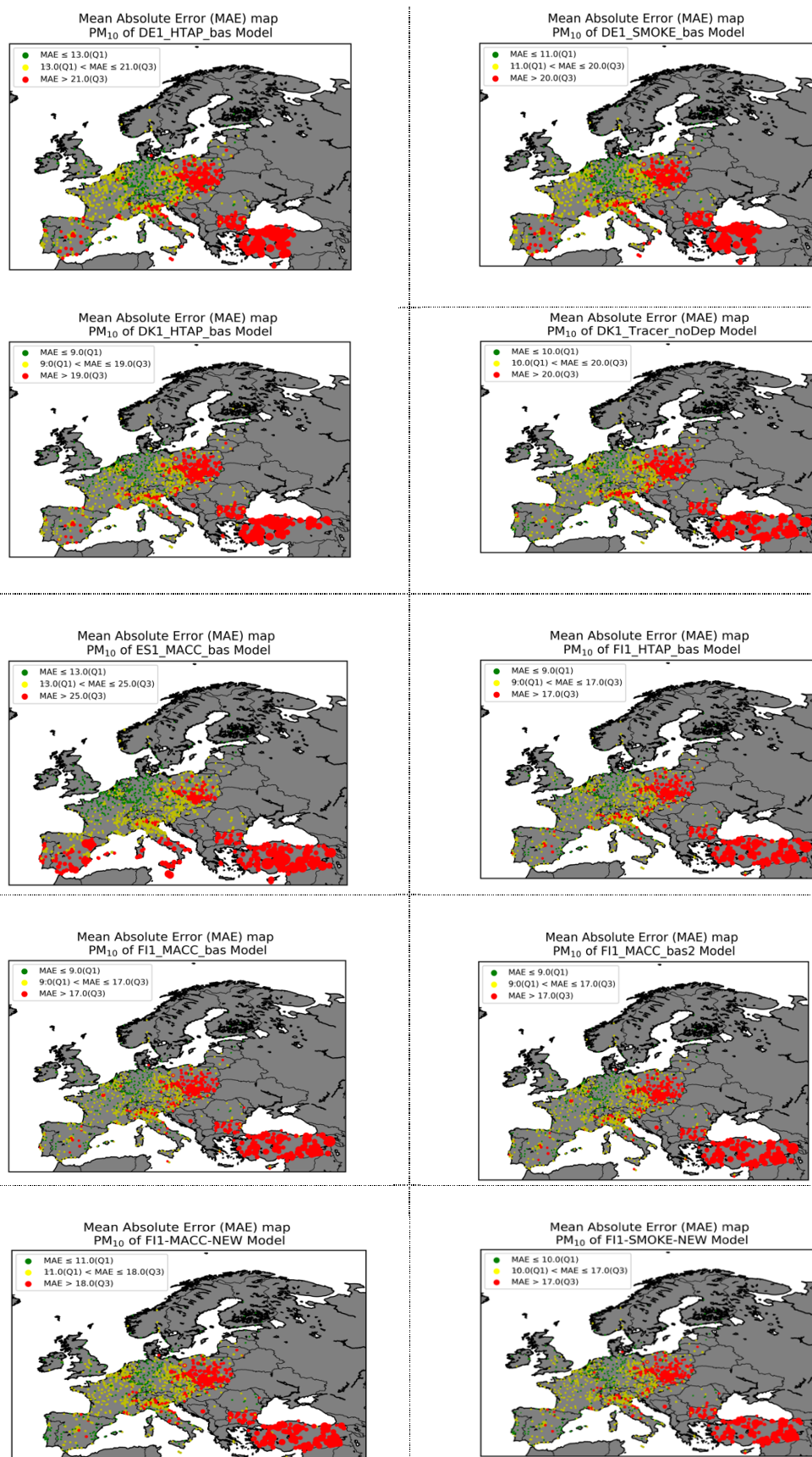
Figure B.3 : MAE maps.
