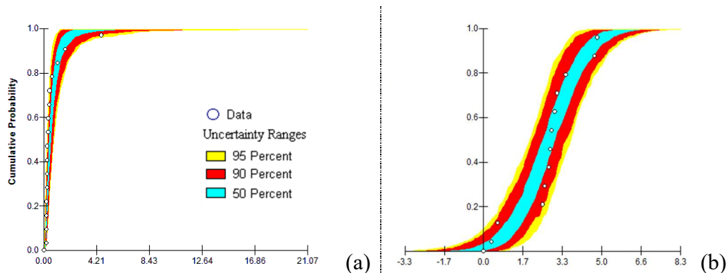
Figure 3.10 : Probability band of dust EFs for “1A1a-10101-3.10” as cumulative distribution of (a)lognormal distribution fitted to dust EFs derived from in-situ measurements (b)normal distribution fitted to dust EFs derived from EMRs.
