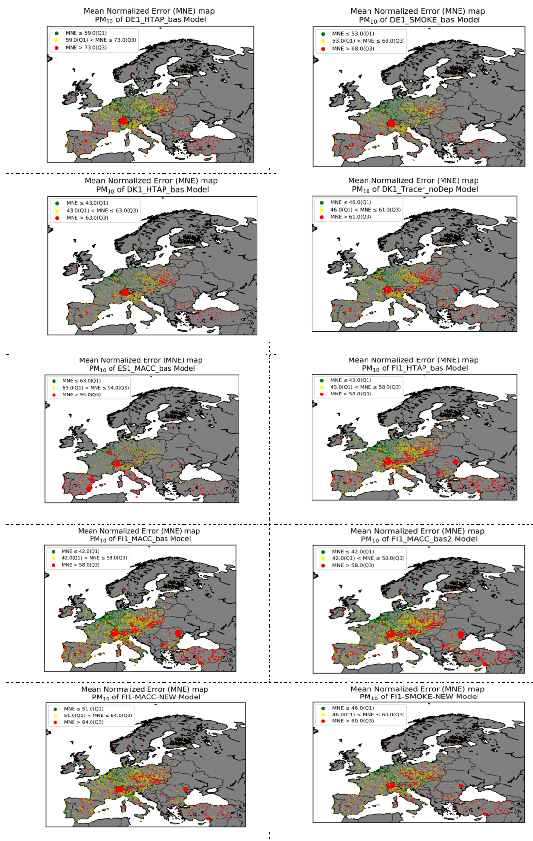
Figure B.5 : MNE maps.
