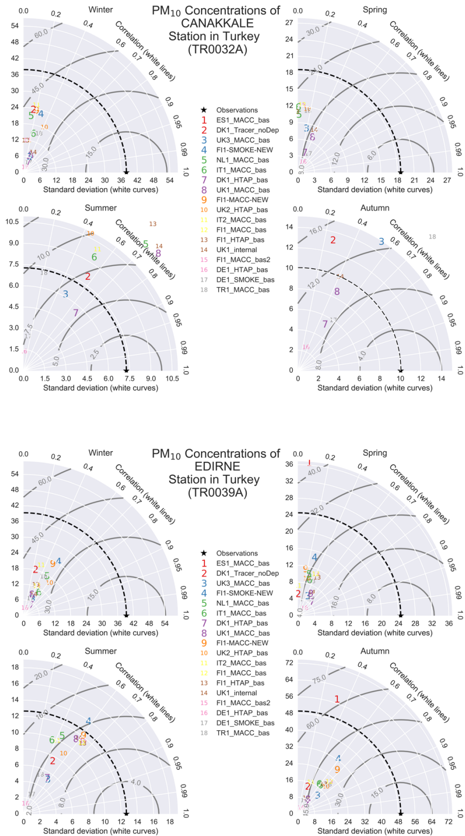
Figure E.1 (continued) : Taylor Diagrams for stations in Marmara region.
