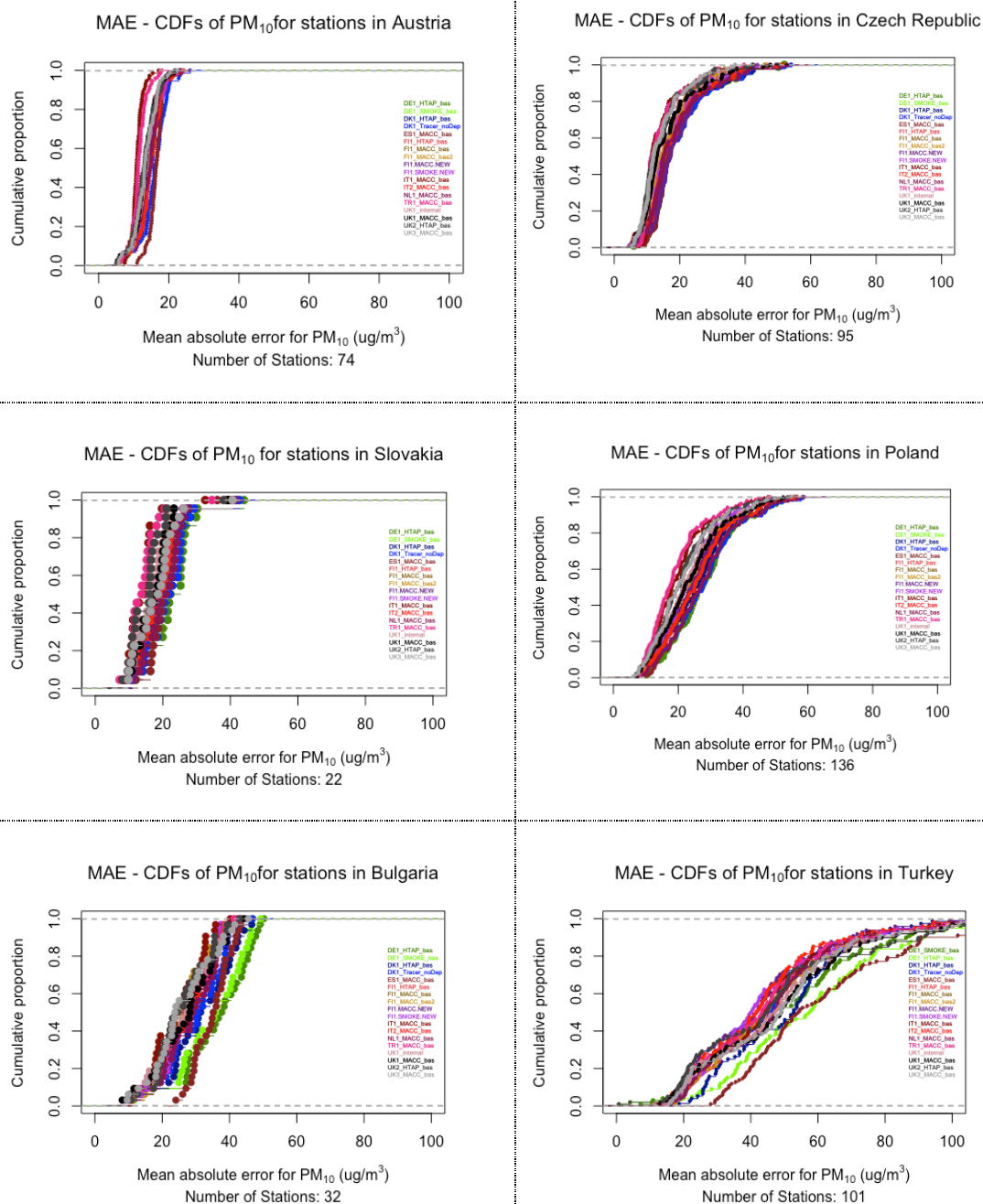
Figure C.1 : MAE CDFs of stations for \text{PM}_{10} , for the countries with more than 10 stations
