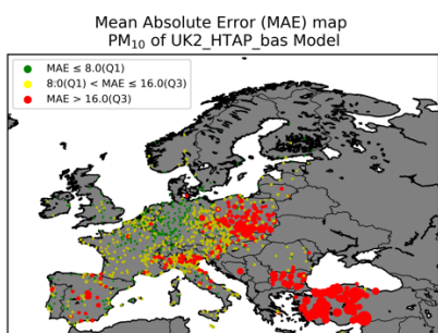
Figure B.3 (continued) : MAE maps.
