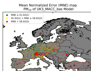
Figure B.5 (continued) : MNE maps.
