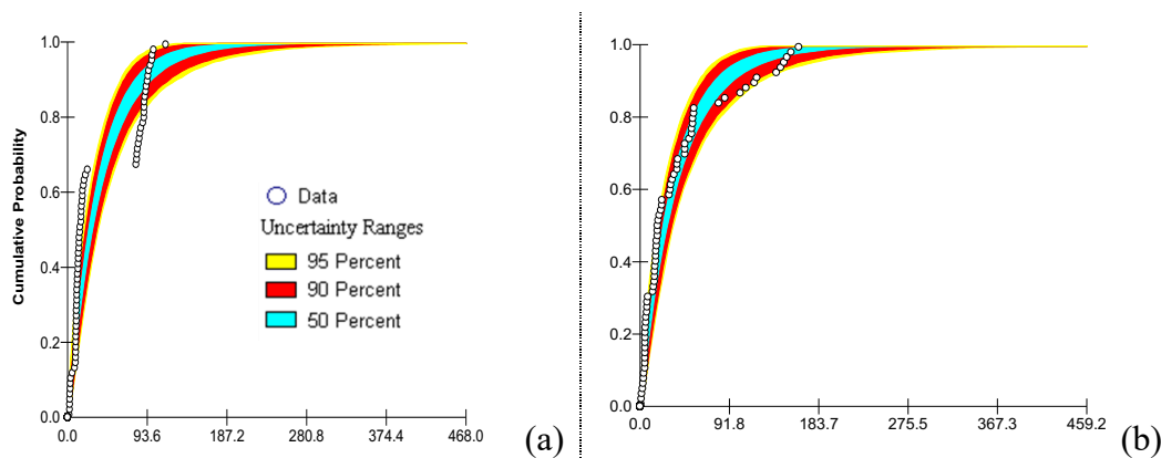
Figure 3.57 : Probability band of NO 2 EFs for “1A1a-10104-3.17” as cumulative distribution of Weibull distribution fitted to NO 2 EFs derived from (a) in-situ measurements (b) EMRs.
