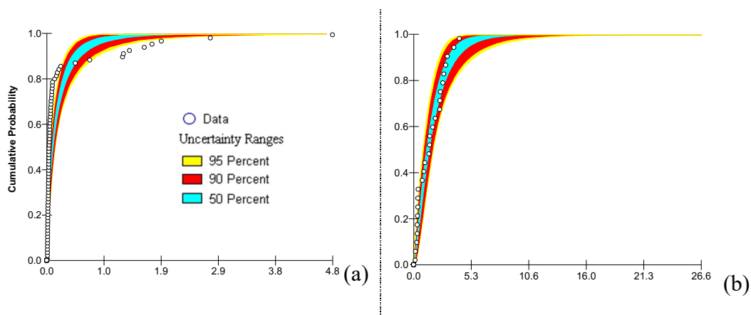
Figure 3.49 : Probability band of dust EFs for “1A1a-10104-3.17” as cumulative distribution of Weibull distribution fitted to dust EFs derived from (a) in-situ measurements (b) EMRs.
