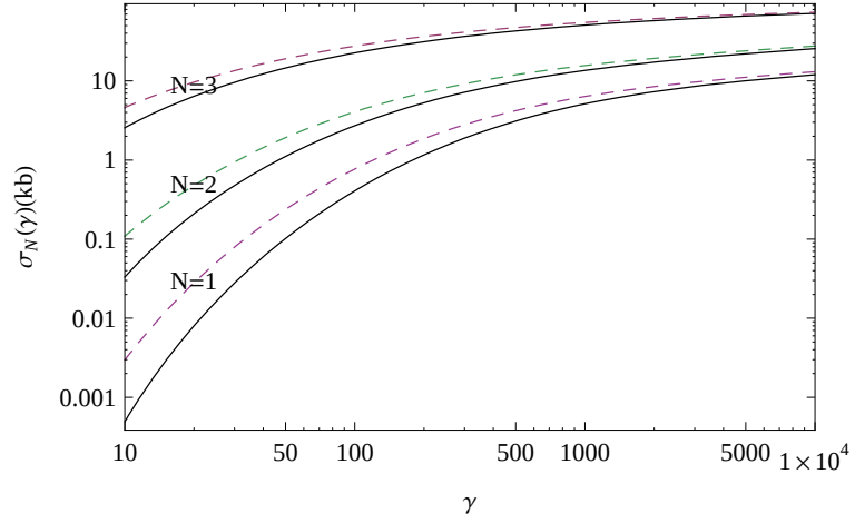
Figure 7.6: Total cross section for the N -pair production in Au-Au collisions versus \gamma with two photon Monte Carlo model for a = 1.8\lambda_c . Solid lines are the corrected calculations, and the dashed are the calculations without corrections
