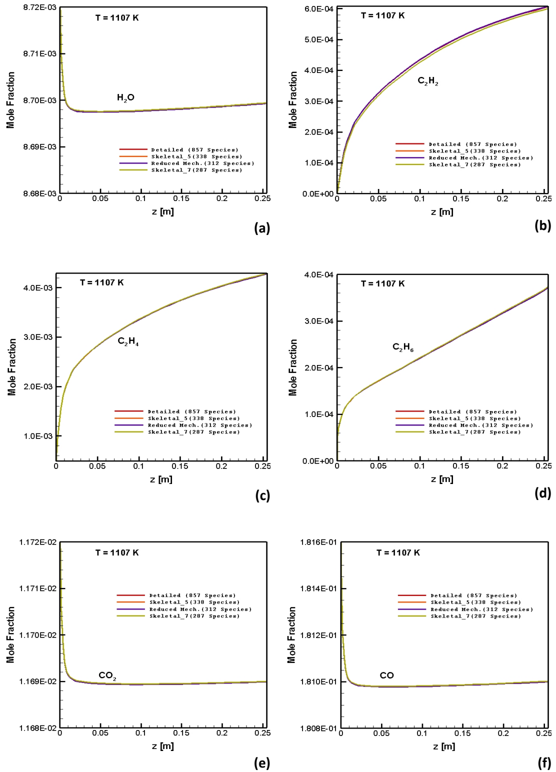
Figure A.12 : Numerically predicted species distribution as a function of axial position along the reactor: C/O=1.3 , 1107\text{ K} : (a) H_2O . (b) C_2H_2 . (c) C_2H_4 . (d) C_2H_6 . (e) CO_2 . (f) CO
