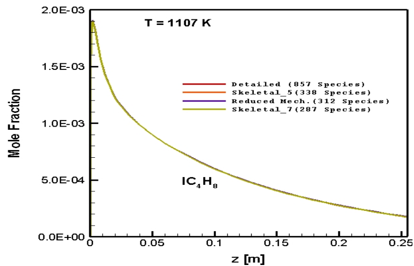
Figure 5.63 : Numerically predicted \text{IC}_4\text{H}_8 distribution as a function of axial position along the reactor: \text{C/O}=1.3 , 1107 K
