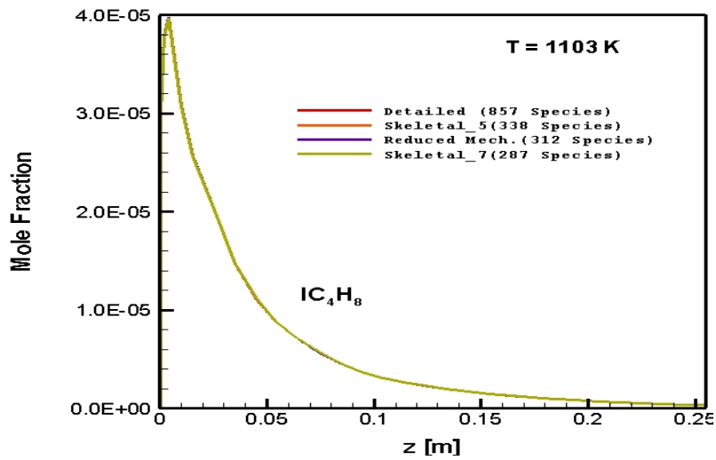
Figure 5.68 : Numerically predicted \text{IC}_4\text{H}_8 distribution as a function of axial position along the reactor: \text{C/O}=1.0 , 1103 K
