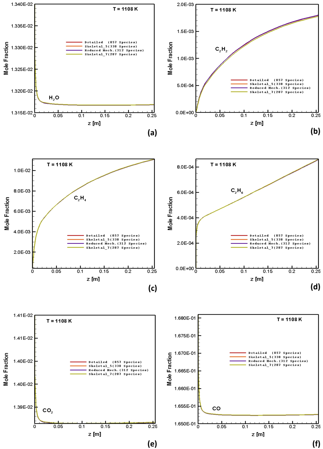
Figure A.10 : Numerically predicted species distribution as a function of axial position along the reactor: C/O=1.6 , 1108 K: (a) H_2O . (b) C_2H_2 . (c) C_2H_4 . (d) C_2H_6 . (e) CO_2 . (f) CO
