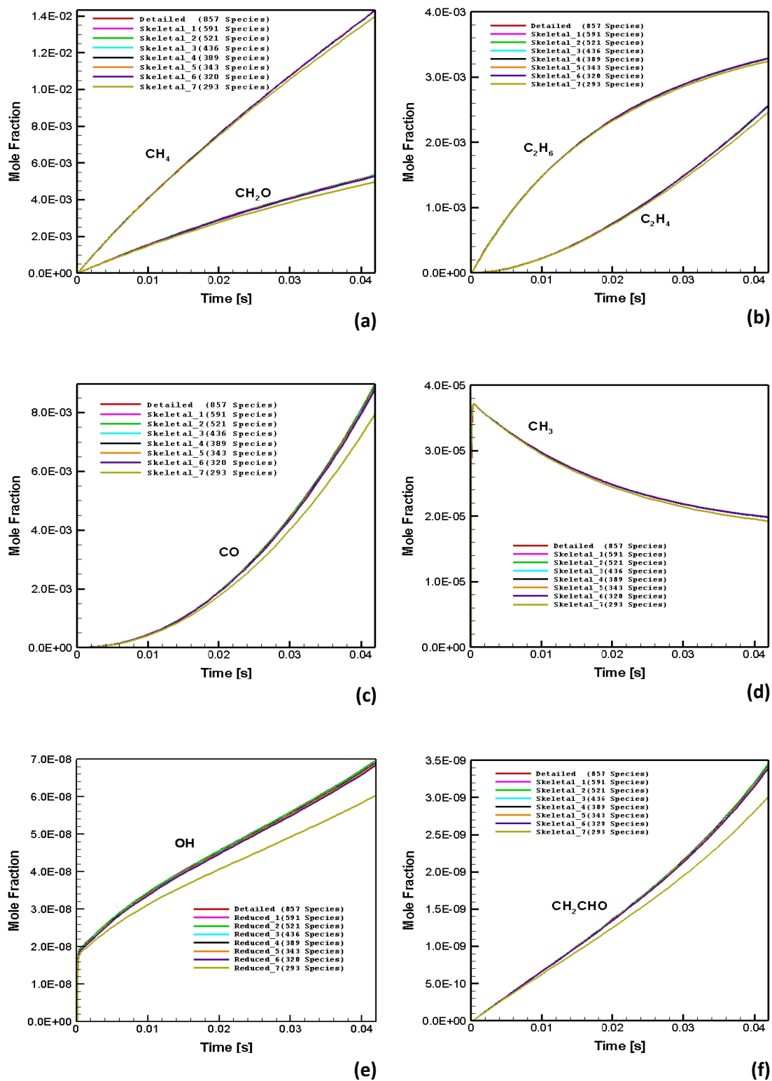
Figure A.3 : Numerically predicted species distribution in CPOX of i-octane as a function of time in the batch reactor: C/O=1.2, 1017.86 K: (a) CH 4 and CH 2 O. (b) C 2 H 6 and C 2 H 4 . (c) CO. (d) CH 3 . (e) OH. (f) CH 2 CHO
