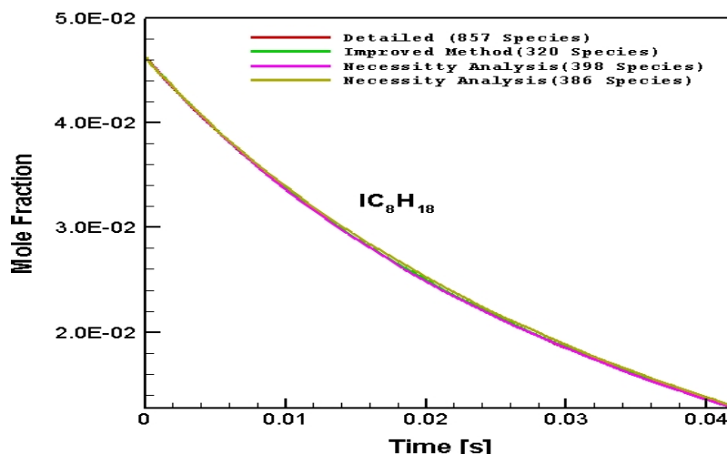
Figure 5.49 : Comparison of the necessity analysis method and improved method for numerically predicted \text{IC}_8\text{H}_{18} distribution in CPOX of i-octane as a function of time in the batch reactor: C/O=1.2, 1017.86)
