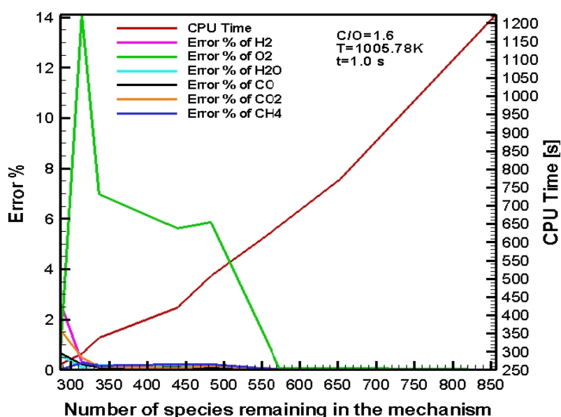
Figure 5.40 : CPU Time – Remaining Species – Error % graph of important species in CPOX of i-octane: C/O=1.6, 1005.78 K, t=1.0 s - 1
