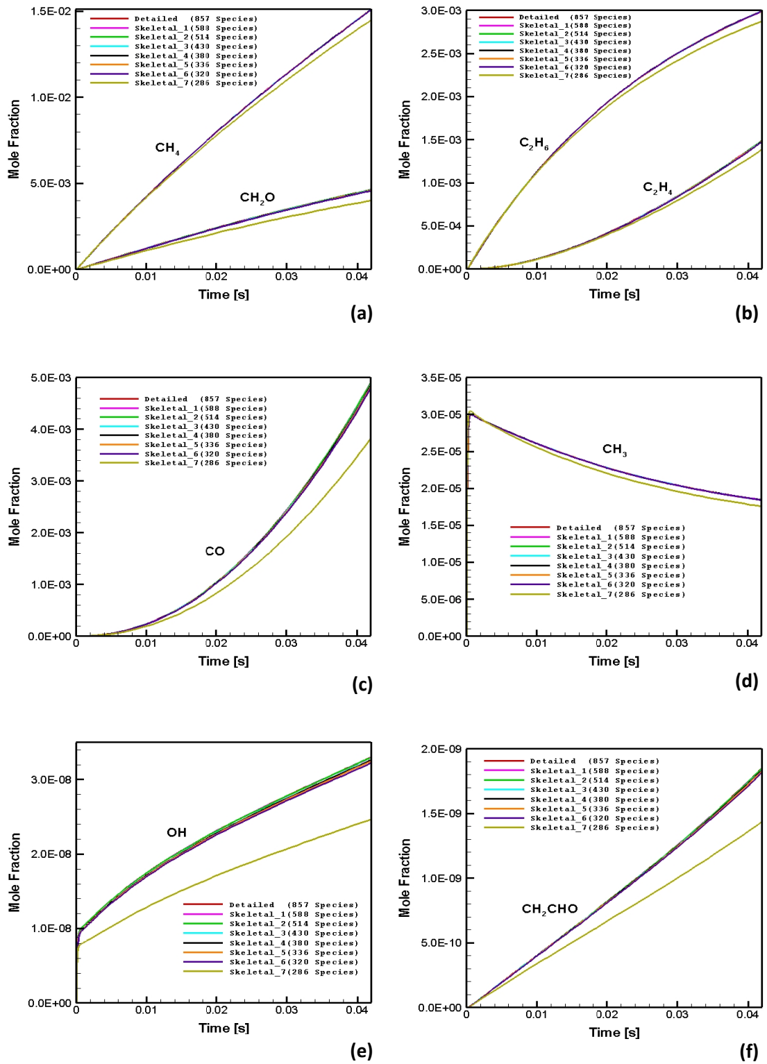
Figure A.2 : Numerically predicted species distribution in CPOX of i-octane as a function of time in the batch reactor: C/O=2.0, 998.26 K: (a) \text{CH}_4 and \text{CH}_2\text{O} . (b) \text{C}_2\text{H}_6 and \text{C}_2\text{H}_4 . (c) \text{CO} . (d) \text{CH}_3 . (e) \text{OH} . (f) \text{CH}_2\text{CHO}
