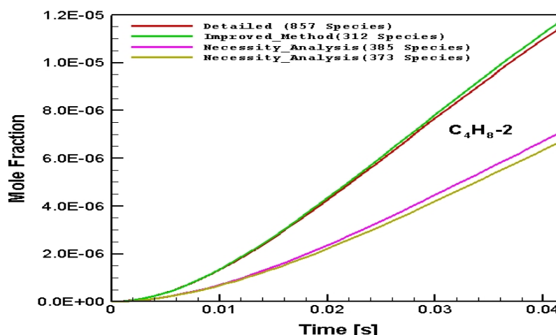
Figure 5.46 : Comparison of the necessity analysis method and improved method for numerically predicted \text{C}_4\text{H}_8\text{-2} distribution in CPOX of i-octane as a function of time in the batch reactor: C/O=1.6, 1005.78 K
