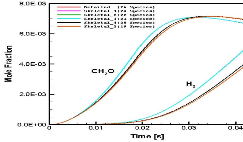
Figure 5.2 : Numerically predicted \text{CH}_2\text{O} and \text{H}_2 distribution in CPOX of methane as a function of time in the batch reactor: \text{C/O}=1.0 , 1005.78 K
