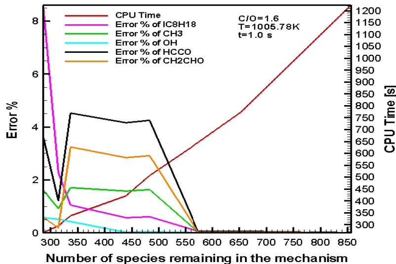
Figure 5.42 : CPU Time – Remaining Species – Error % graph of important species in CPOX of i-octane: C/O=1.6, 1005.78 K, t=1.0 s - 3
