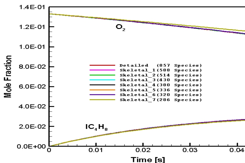
Figure 5.17 : Numerical prediction of O 2 and IC 4 H 8 distribution in CPOX of i-octane as a function of time in the batch reactor: C/O=2.0, 998.26 K
