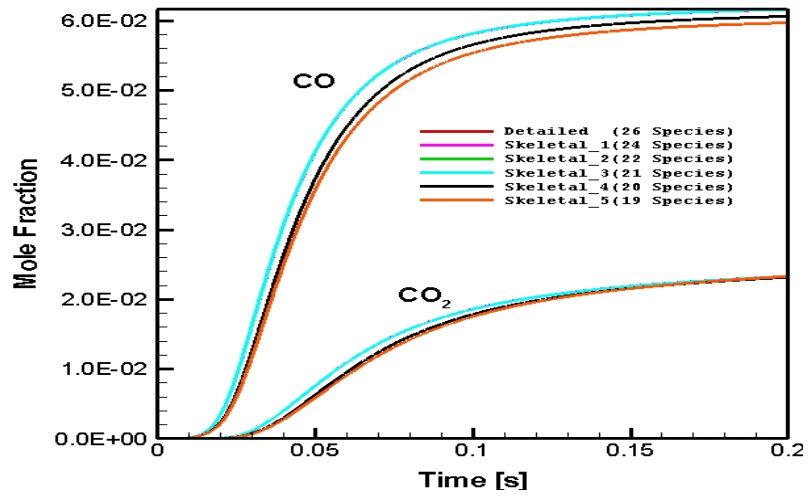
Figure 5.7 : Numerically predicted \text{CO}_2 and \text{CO} distribution in CPOX of methane as a function of time in the batch reactor: \text{C/O}=1.0 , 1005.78 K, t=0.2\text{s}
