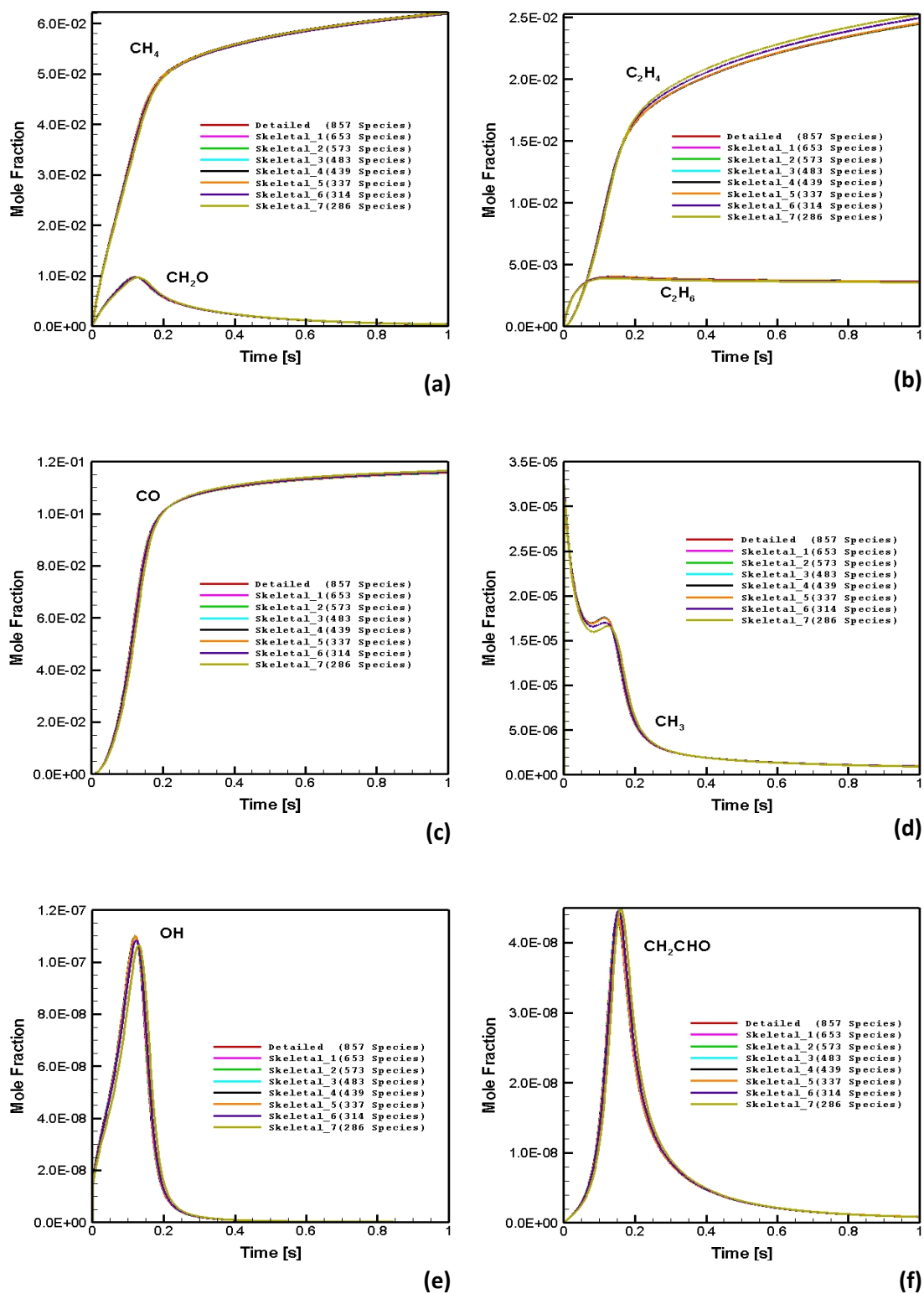
Figure A.5 : Numerically predicted species distribution in CPOX of i-octane as a function of time in the batch reactor: \text{C/O}=1.6 , 1005.78 K, t=1.0\text{s} : (a) \text{CH}_4 and \text{CH}_2\text{O} . (b) \text{C}_2\text{H}_6 and \text{C}_2\text{H}_4 . (c) \text{CO} . (d) \text{CH}_3 . (e) \text{OH} . (f) \text{CH}_2\text{CHO}
