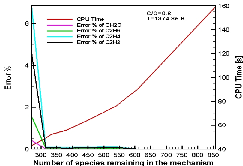
Figure 5.35 : CPU Time – Remaining Species – Error % graph of important species in CPOX of i-octane: C/O=0.8, 1374.85 K – 3
