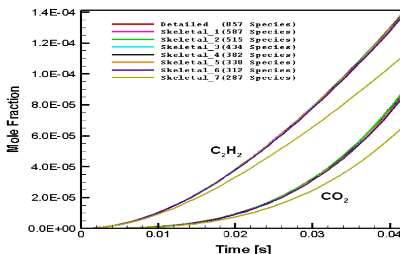
Figure 5.11 : Numerically predicted C_2H_2 and CO_2 distribution in CPOX of i-octane as a function of time in the batch reactor: C/O=1.6 , 1005.78 K
