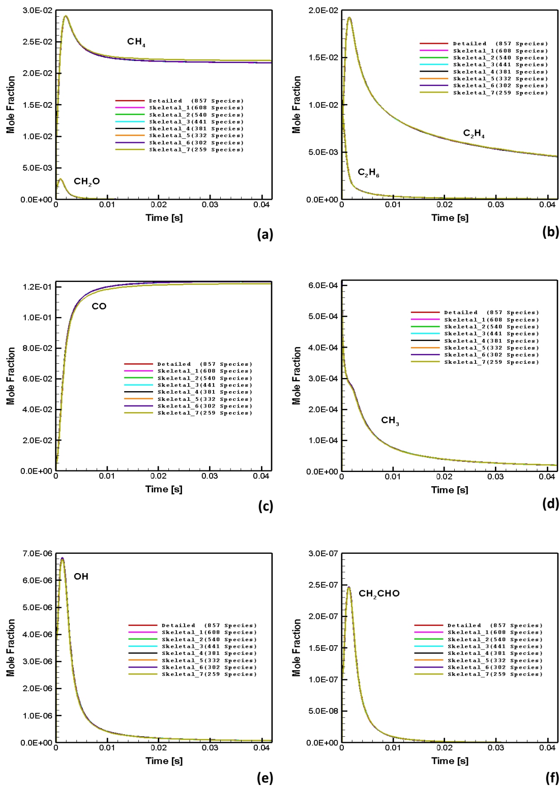
Figure A.4 : Numerically predicted species distribution in CPOX of i-octane as a function of time in the batch reactor: C/O=0.8 , 1374.85\text{ K} : (a) CH_4 and CH_2O . (b) C_2H_6 and C_2H_4 . (c) CO . (d) CH_3 . (e) OH . (f) CH_2CHO
