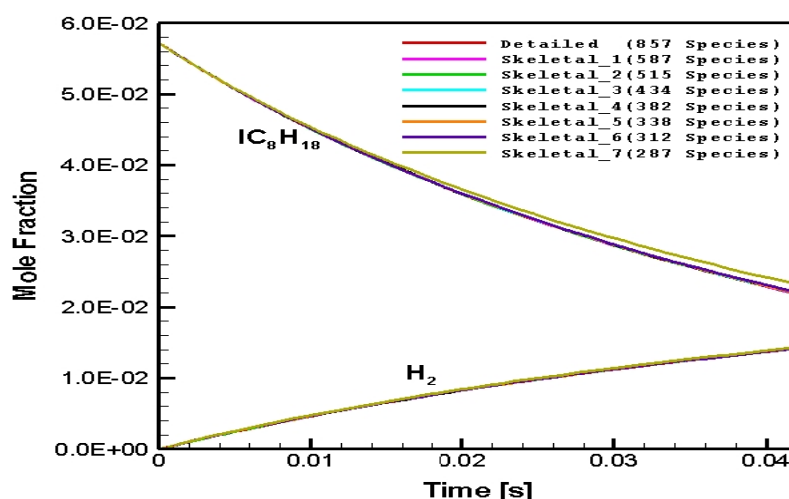
Figure 5.8 : Numerically predicted H_2 and IC_8H_{18} distribution in CPOX of i-octane as a function of time in the batch reactor: C/O=1.6, 1005.78 K
