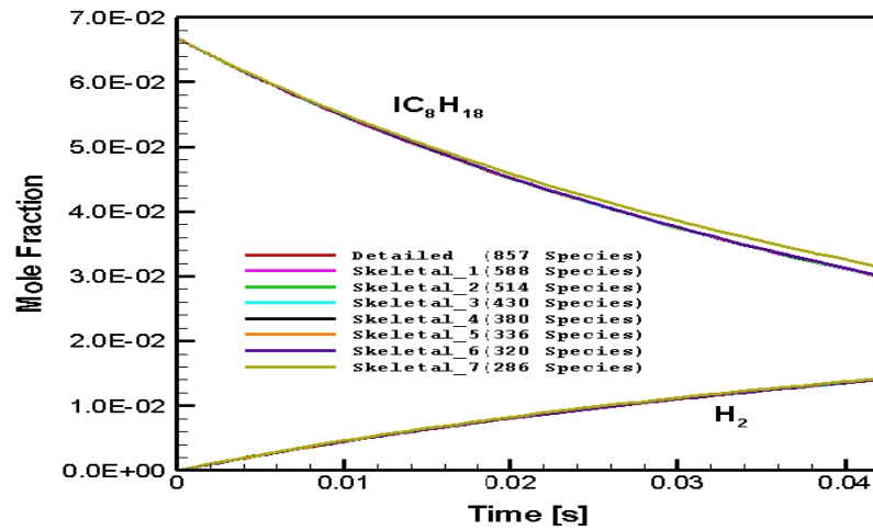
Figure 5.15 : Numerical prediction of H_2 and IC_8H_{18} distribution in CPOX of i-octane as a function of time in the batch reactor: C/O=2.0, 998.26 K
