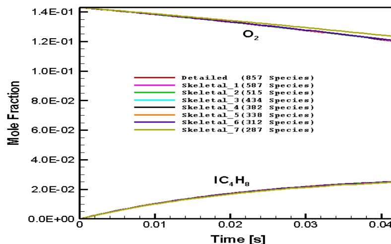
Figure 5.10 : Numerically predicted O_2 and IC_4H_8 distribution in CPOX of i-octane as a function of time in the batch reactor: C/O=1.6 , 1005.78 K
