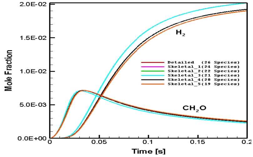
Figure 5.5 : Numerically predicted \text{CH}_2\text{O} and \text{H}_2 distribution in CPOX of methane as a function of time in the batch reactor: \text{C/O}=1.0 , 1005.78 K, t=0.2\text{s}
