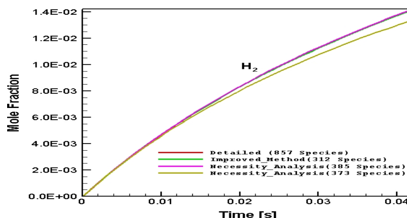
Figure 5.43 : Comparison of the necessity analysis method and improved method for numerically predicted H_2 distribution in CPOX of i-octane as a function of time in the batch reactor: C/O=1.6, 1005.78 K
