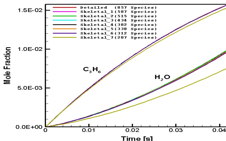
Figure 5.9 : Numerically predicted H_2O and C_3H_6 distribution in CPOX of i-octane as a function of time in the batch reactor: C/O=1.6, 1005.78 K
