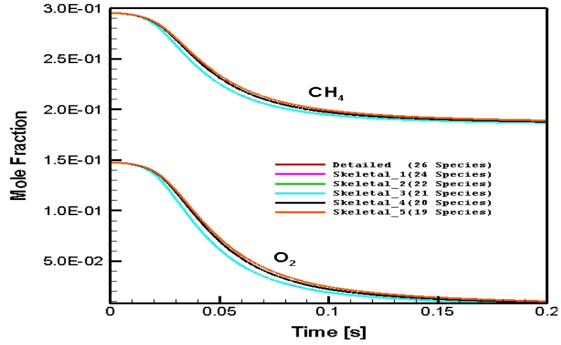
Figure 5.6 : Numerically predicted \text{CH}_4 and \text{O}_2 distribution in CPOX of methane as a function of time in the batch reactor: \text{C/O}=1.0 , 1005.78 K, t=0.2\text{s}
