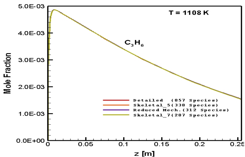
Figure 5.55 : Numerically predicted \text{C}_3\text{H}_6 distribution as a function of axial position along the reactor: \text{C}/\text{O}=1.6 , 1108 K
