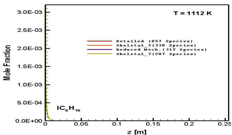
Figure 5.57 : Numerically predicted IC_8H_{18} distribution as a function of axial position along the reactor: C/O=2.0, 1112 K
