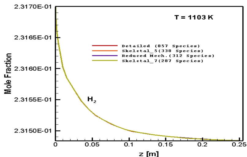
Figure 5.66 : Numerically predicted H 2 distribution as a function of axial position along the reactor: C/O=1.0, 1103 K
