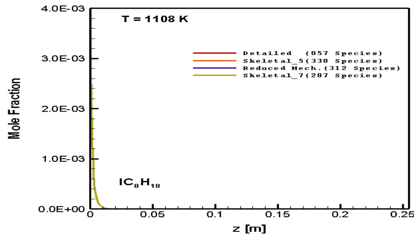
Figure 5.52 : Numerically predicted IC 8 H 18 distribution as a function of axial position along the reactor: C/O=1.6, 1108 K
