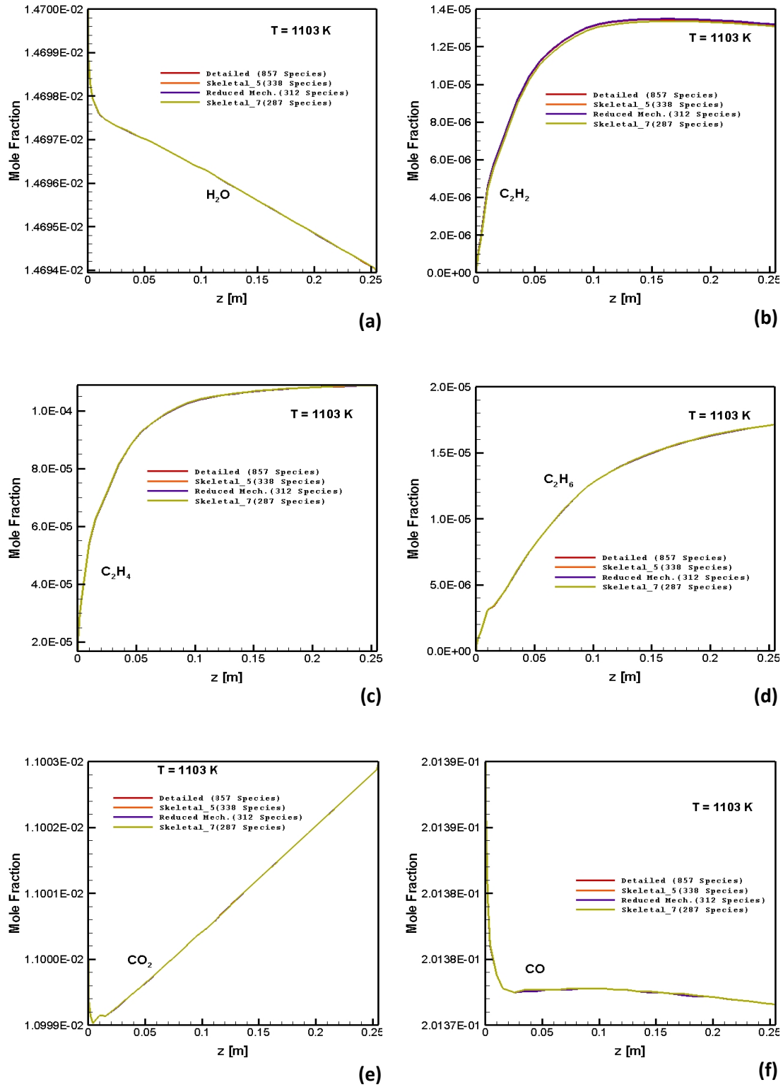
Figure A.13 : Numerically predicted species distribution as a function of axial position along the reactor: C/O=1.0 , 1103\text{ K} : (a) H_2O . (b) C_2H_2 . (c) C_2H_4 . (d) C_2H_6 . (e) CO_2 . (f) CO
