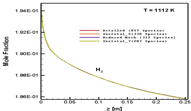
Figure 5.56 : Numerically predicted H_2 distribution as a function of axial position along the reactor: C/O=2.0, 1112 K
