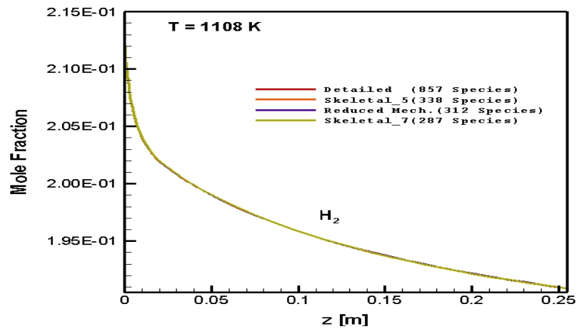
Figure 5.51 : Numerically predicted H 2 distribution as a function of axial position along the reactor: C/O=1.6, 1108 K
