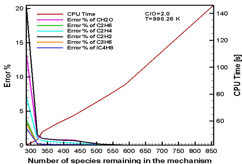
Figure 5.20 : CPU Time – Remaining Species – Error % graph of important species in CPOX of i-octane: C/O=2.0 , 998.26 K - 2
