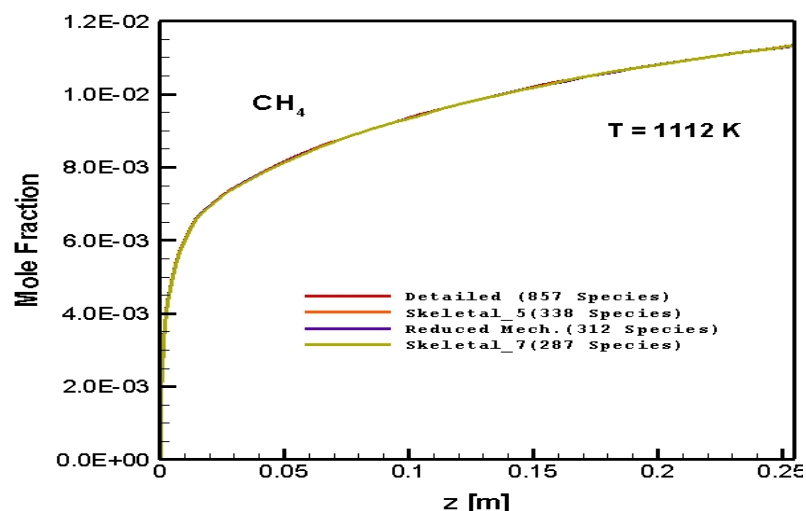
Figure 5.59 : Numerically predicted \text{CH}_4 distribution as a function of axial position along the reactor: \text{C/O}=2.0 , 1112 K
