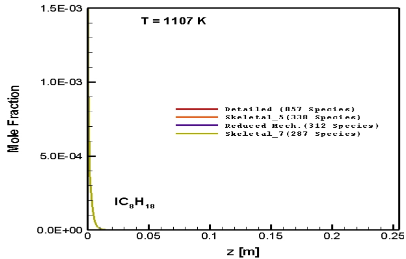
Figure 5.62 : Numerically predicted \text{IC}_8\text{H}_{18} distribution as a function of axial position along the reactor: \text{C/O}=1.3 , 1107 K
