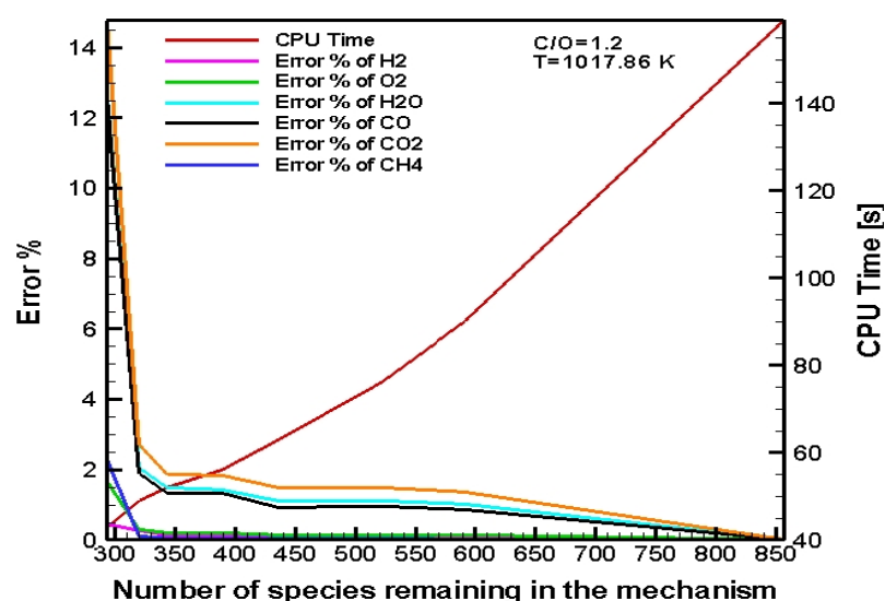
Figure 5.26 : CPU Time – Remaining Species – Error % graph of important species in CPOX of i-octane: C/O=1.2, 1017.86 K - 1
