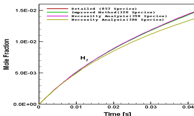
Figure 5.47 : Comparison of the necessity analysis method and improved method for numerically predicted H_2 distribution in CPOX of i-octane as a function of time in the batch reactor: C/O=1.2 , 1017.86
