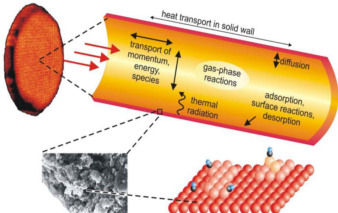
Figure 1.1 : Catalytic combustion monolith and physical and chemical process occurring in the single monolith channel [14]
