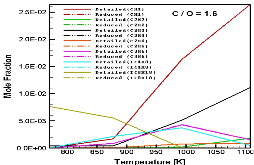
Figure 5.71 : Numerically predicted distribution of some important species as a function of gas temperature at one exact position in the channel (20 mm): C/O=1.6
