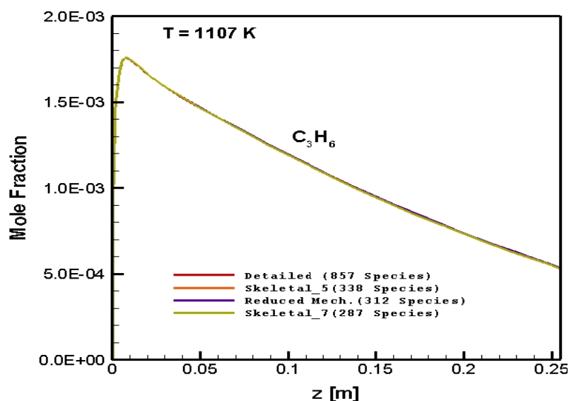
Figure 5.65 : Numerically predicted C_3H_6 distribution as a function of axial position along the reactor: C/O=1.3, 1107 K
