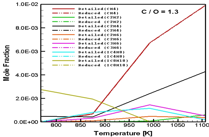
Figure 5.73 : Numerically predicted distribution of some important species as a function of gas temperature at one exact position in the channel (20 mm); C/O=1.3
