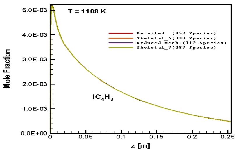
Figure 5.53 : Numerically predicted \text{IC}_4\text{H}_8 distribution as a function of axial position along the reactor: \text{C}/\text{O}=1.6 , 1108 K
