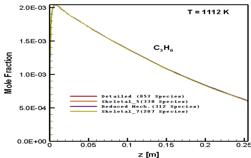
Figure 5.60 : Numerically predicted \text{C}_3\text{H}_6 distribution as a function of axial position along the reactor: \text{C/O}=2.0 , 1112 K
