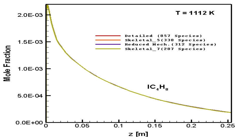
Figure 5.58 : Numerically predicted IC_4H_8 distribution as a function of axial position along the reactor: C/O=2.0, 1112 K
