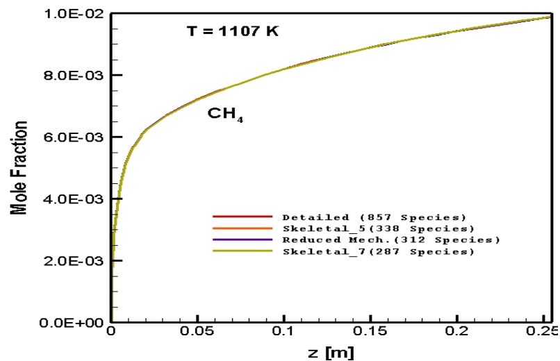
Figure 5.64 : Numerically predicted \text{CH}_4 distribution as a function of axial position along the reactor: \text{C/O}=1.3 , 1107 K
