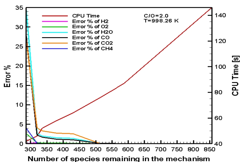
Figure 5.19 : CPU Time – Remaining Species – Error % graph of important species in CPOX of i-octane: C/O=2.0 , 998.26 K - 1
