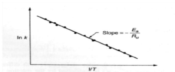
Figure 2.1 : Temperature dependence of reaction rate constant k [22]
