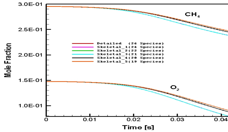
Figure 5.3 : Numerically predicted \text{CH}_4 and \text{O}_2 distribution in CPOX of methane as a function of time in the batch reactor: \text{C/O}=1.0 , 1005.78 K
