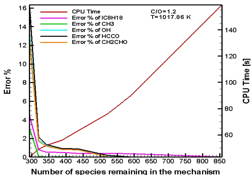
Figure 5.28 : Remaining Species –Error % of \text{IC}_4\text{H}_8 in CPOX of i-octane: \text{C/O}=1.2 , 1017.86 K
