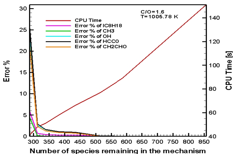
Figure 5.14 : CPU Time – Remaining Species – Error % graph of important species in CPOX of i-octane: C/O=1.6, 1005.78 K - 3
