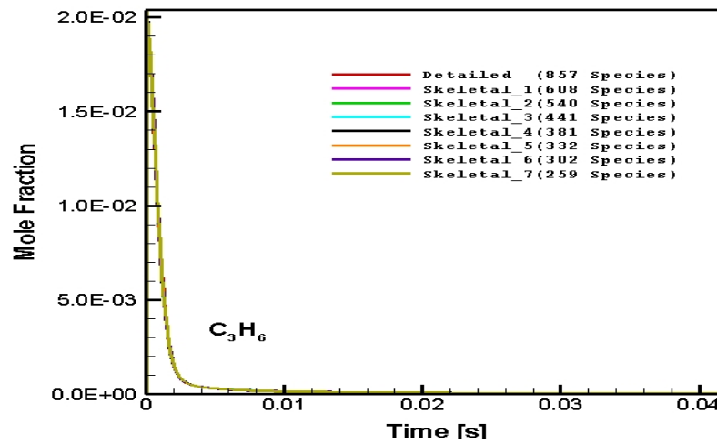
Figure 5.30 : Numerically predicted C_3H_6 distribution in CPOX of i-octane as a function of time in the batch reactor: C/O=0.8, 1374.85 K
