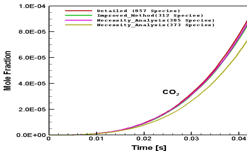
Figure 5.44 : Comparison of the necessity analysis method and improved method for numerically predicted \text{CO}_2 distribution in CPOX of i-octane as a function of time in the batch reactor: C/O=1.6, 1005.78 K
