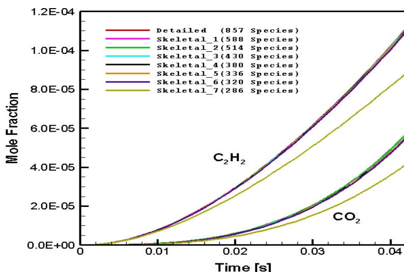
Figure 5.18 : Numerical prediction of C 2 H 2 and CO 2 distribution in CPOX of i-octane as a function of time in the batch reactor: C/O=2.0, 998.26 K
