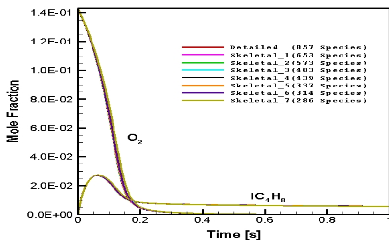
Figure 5.38 : Numerically predicted \text{O}_2 and \text{IC}_4\text{H}_8 distribution in CPOX of i-octane as a function of time in the batch reactor: \text{C}/\text{O}=1.6 , 1005.78 K, t=1.0\text{s}
