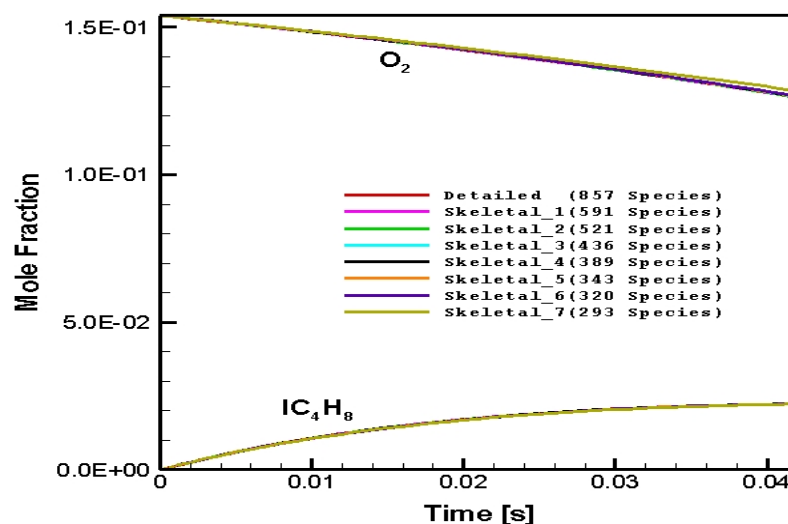
Figure 5.24 : Numerically predicted O_2 and IC_4H_8 distribution in CPOX of i-octane as a function of time in the batch reactor: C/O=1.2 , 1017.86 K
