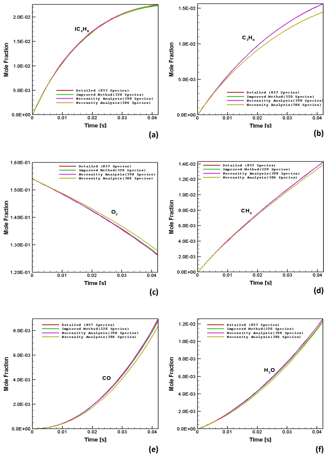
Figure A.8 : Comparison of the necessity analysis method and improved method for numerically predicted species distribution in CPOX of i-octane as a function of time in the batch reactor: C/O=1.2, 1017.86: (a) \text{IC}_4\text{H}_8 . (b) \text{C}_3\text{H}_6 . (c) \text{O}_2 . (d) \text{CH}_4 . (e) \text{CO} . (f) \text{H}_2\text{O}
