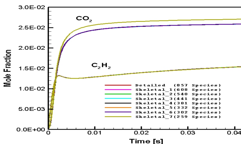
Figure 5.32 : Numerically predicted C 2 H 2 and CO 2 distribution in CPOX of i-octane as a function of time in the batch reactor: C/O=0.8, 1374.85 K
