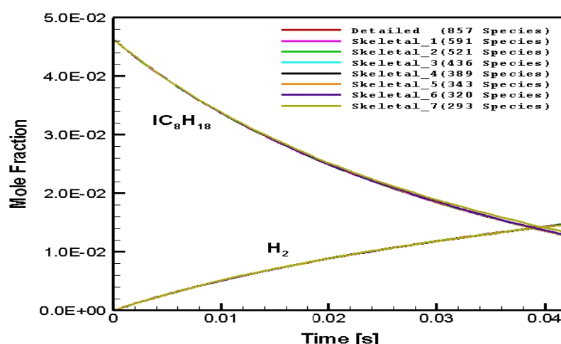
Figure 5.22 : Numerically predicted H_2 and IC_8H_{18} distribution in CPOX of i-octane as a function of time in the batch reactor: C/O=1.2, 1017.86 K
