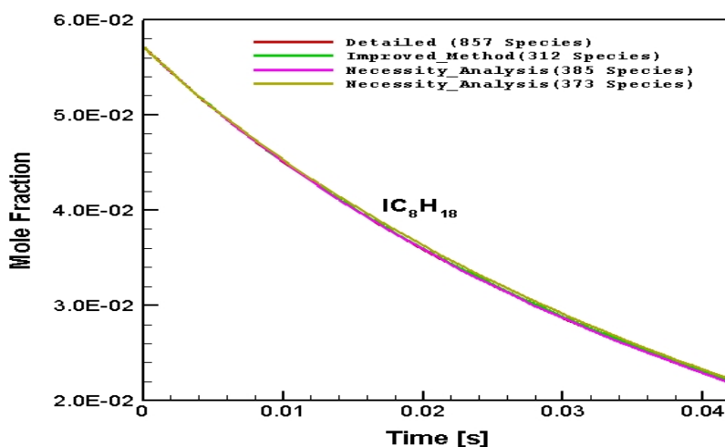
Figure 5.45 : Comparison of the necessity analysis method and improved method for numerically predicted \text{IC}_8\text{H}_{18} distribution in CPOX of i-octane as a function of time in the batch reactor: C/O=1.6, 1005.78 K
