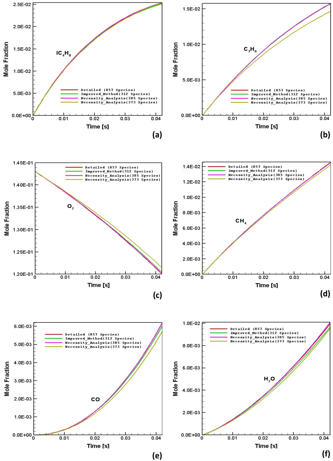
Figure A.6 : Comparison of the necessity analysis method and improved method for numerically predicted species distribution in CPOX of i-octane as a function of time in the batch reactor: C/O=1.6, 1005.78 K: (a) \text{IC}_4\text{H}_8 . (b) \text{C}_3\text{H}_6 . (c) \text{O}_2 . (d) \text{CH}_4 . (e) \text{CO} . (f) \text{H}_2\text{O}
