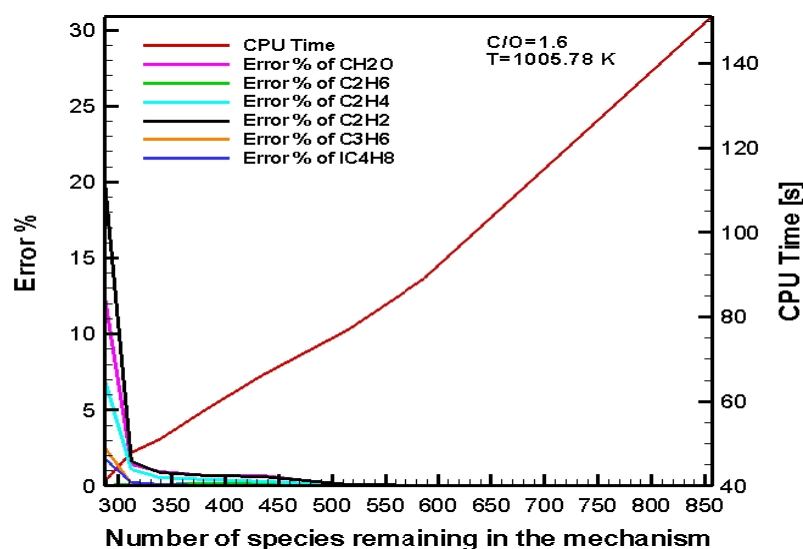
Figure 5.13 : CPU Time – Remaining Species – Error % graph of important species in CPOX of i-octane: C/O=1.6 , 1005.78 K - 2
