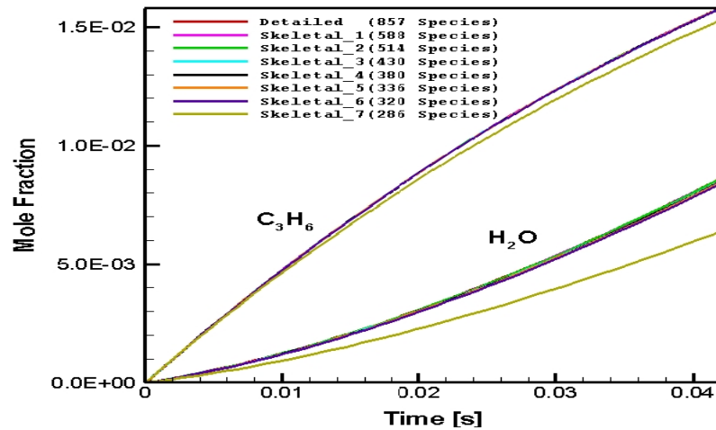
Figure 5.16 : Numerical prediction of H_2O and C_3H_6 distribution in CPOX of i-octane as a function of time in the batch reactor: C/O=2.0, 998.26 K
