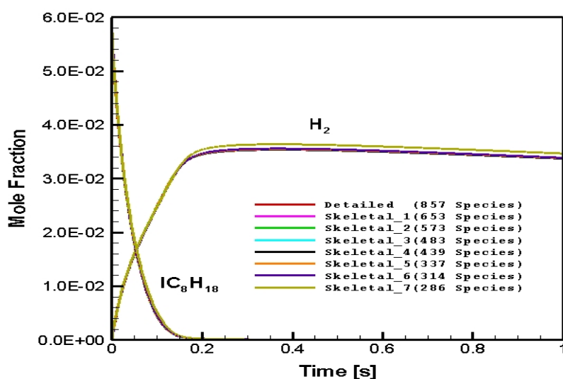
Figure 5.36 : Numerically predicted H 2 and IC 8 H 18 distribution in CPOX of i-octane as a function of time in the batch reactor: C/O=1.6, 1005.78 K, t=1.0s
