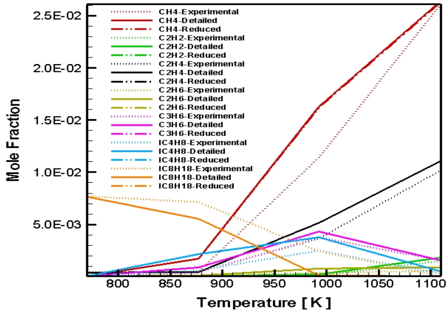
Figure 5.75 : Numerically predicted and experimentally measured distribution of some important species as a function of gas temperature at one exact position in the channel (20 mm): C/O=1.6
