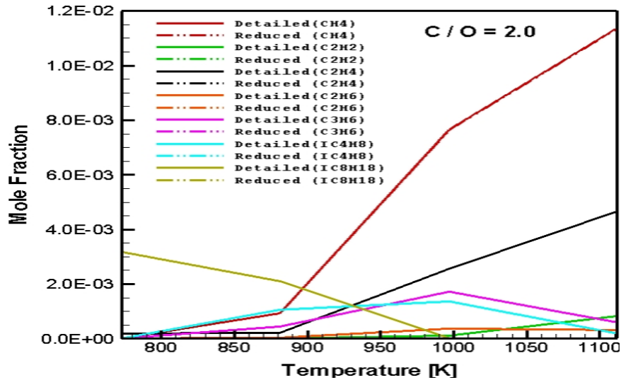
Figure 5.72 : Numerically predicted distribution of some important species as a function of gas temperature at one exact position in the channel (20 mm): C/O=2.0
