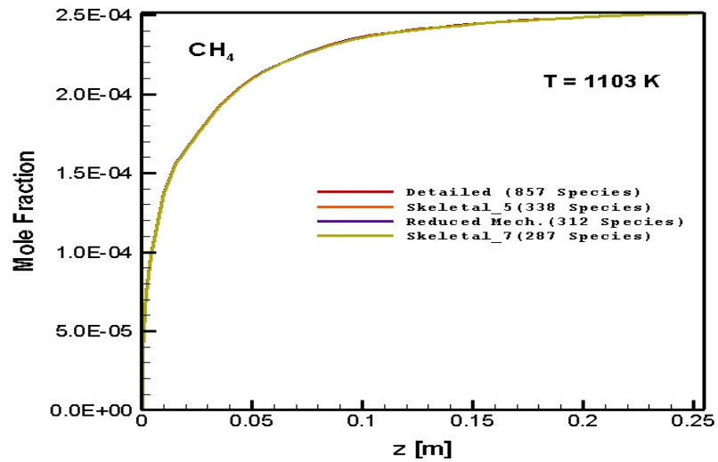
Figure 5.69 : Numerically predicted \text{CH}_4 distribution as a function of axial position along the reactor: \text{C/O}=1.0 , 1103 K
