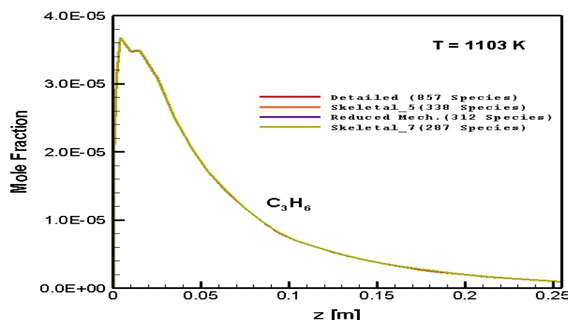
Figure 5.70 : Numerically predicted C_3H_6 distribution as a function of axial position along the reactor: C/O=1.0, 1103 K
