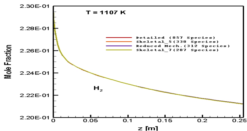
Figure 5.61 : Numerically predicted H 2 distribution as a function of axial position along the reactor: C/O=1.3, 1107 K
