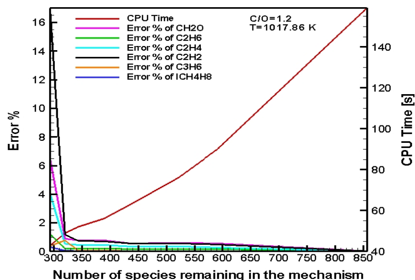
Figure 5.27 : CPU Time – Remaining Species – Error % graph of important species in CPOX of i-octane: C/O=1.2, 1017.86 K – 1
