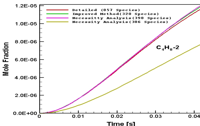
Figure 5.50 : Comparison of the necessity analysis method and improved method for numerically predicted \text{C}_4\text{H}_8\text{-2} distribution in CPOX of i-octane as a function of time in the batch reactor: C/O=1.2, 1017.86)
