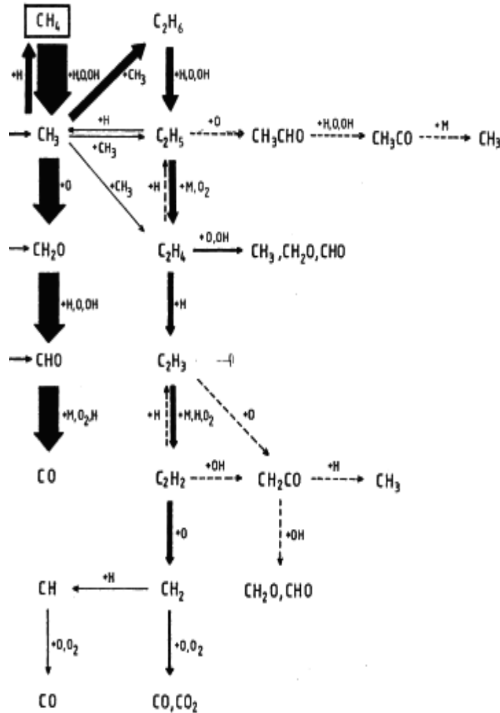
Figure 3.3 : Integral reaction flow analysis in a premixed stoichiometric CH 4 /air flame at p=1 bar and T u =298 K [30]
