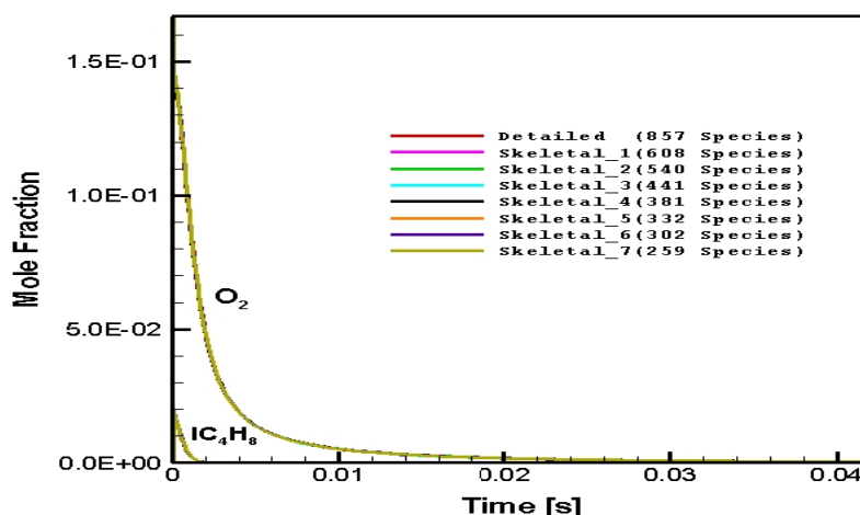
Figure 5.31 : Numerically predicted O 2 and IC 4 H 8 distribution in CPOX of i-octane as a function of time in the batch reactor: C/O=0.8, 1374.85 K
