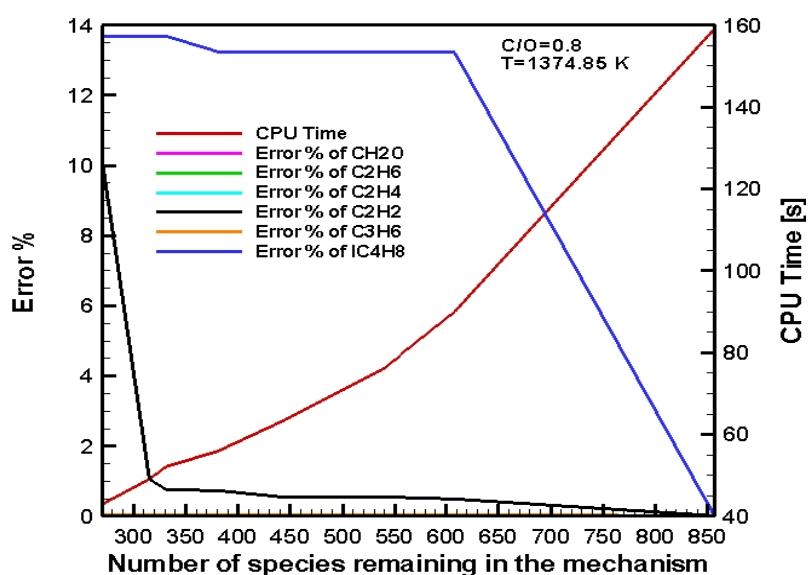
Figure 5.34 : CPU Time – Remaining Species – Error % graph of important species in CPOX of i-octane: C/O=0.8, 1374.85 K – 2
