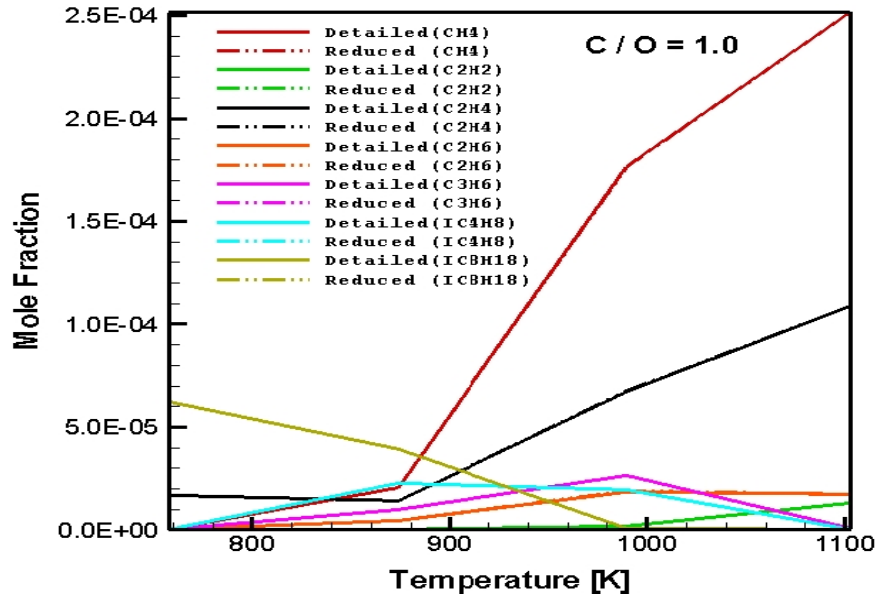
Figure 5.74 : Numerically predicted distribution of some important species as a function of gas temperature at one exact position in the channel (20 mm); C/O=1.0
