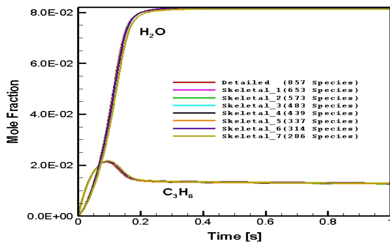
Figure 5.37 : Numerically predicted \text{H}_2\text{O} and \text{C}_3\text{H}_6 distribution in CPOX of i-octane as a function of time in the batch reactor: \text{C}/\text{O}=1.6 , 1005.78 K, t=1.0\text{s}
