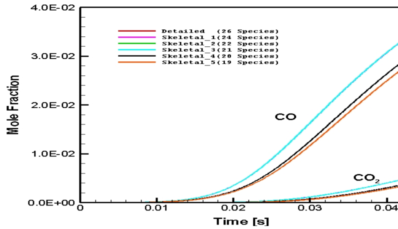
Figure 5.4 : Numerically predicted \text{CO}_2 and \text{CO} distribution in CPOX of methane as a function of time in the batch reactor: \text{C/O}=1.0 , 1005.78 K
