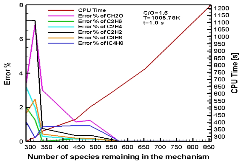
Figure 5.41 : CPU Time – Remaining Species – Error % graph of important species in CPOX of i-octane: C/O=1.6, 1005.78 K, t=1.0 s - 2
