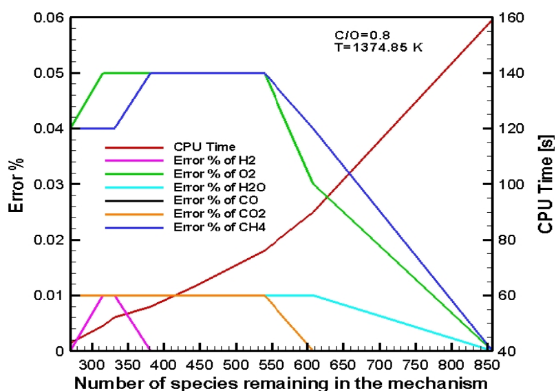
Figure 5.33 : CPU Time – Remaining Species – Error % graph of important species in CPOX of i-octane: C/O=0.8, 1374.85 K – 1
