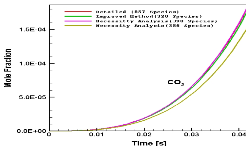
Figure 5.48 : Comparison of the necessity analysis method and improved method for numerically predicted CO_2 distribution in CPOX of i-octane as a function of time in the batch reactor: C/O=1.2 , 1017.86)
