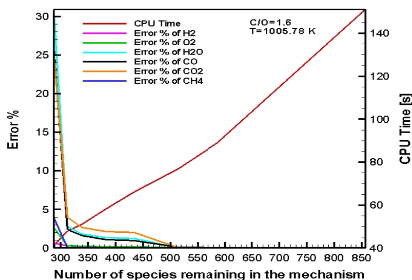
Figure 5.12 : CPU Time – Remaining Species – Error % graph of important species in CPOX of i-octane: C/O=1.6 , 1005.78 K - 1
