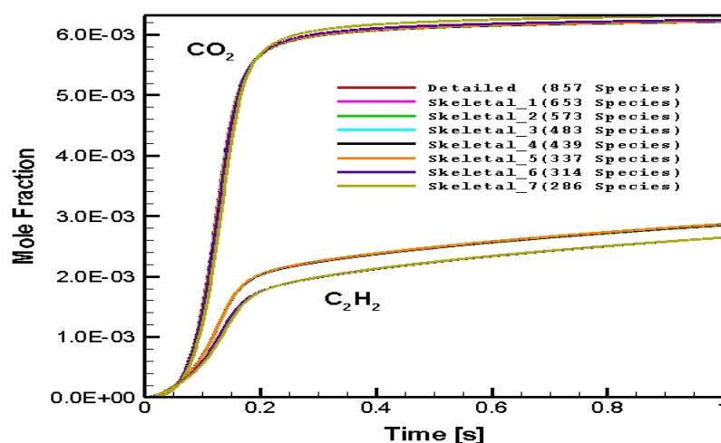
Figure 5.39 : Numerically predicted \text{C}_2\text{H}_2 and \text{CO}_2 distribution in CPOX of i-octane as a function of time in the batch reactor: \text{C}/\text{O}=1.6 , 1005.78 K, t=1.0\text{s}
