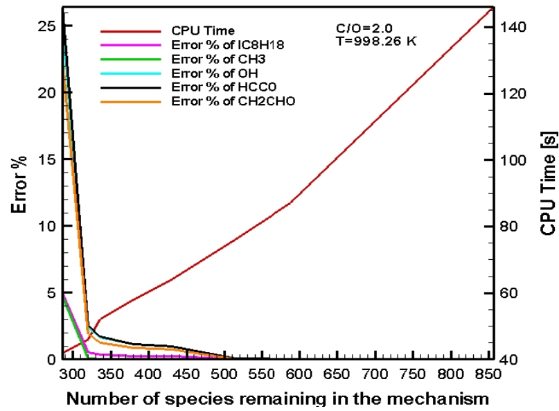
Figure 5.21 : CPU Time – Remaining Species – Error % graph of important species in CPOX of i-octane: C/O=2.0, 998.26 K - 3
