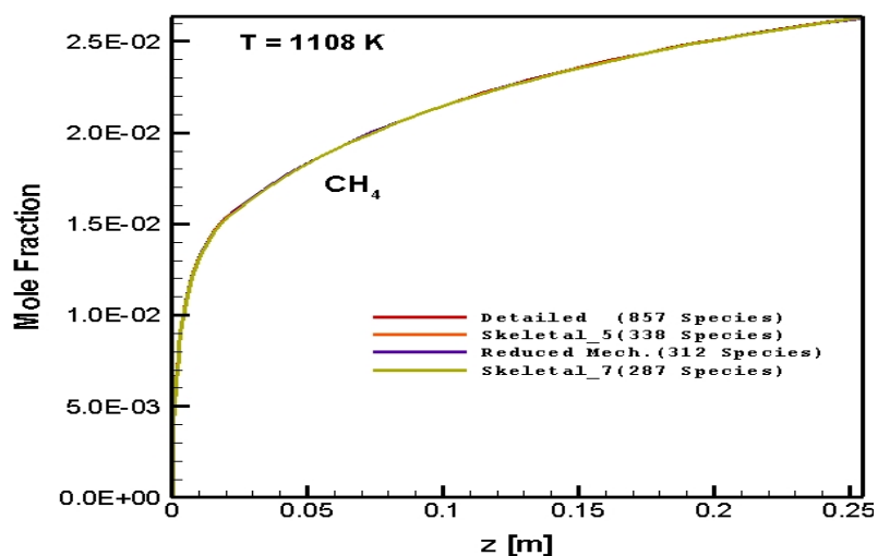
Figure 5.54 : Numerically predicted \text{CH}_4 distribution as a function of axial position along the reactor: \text{C}/\text{O}=1.6 , 1108 K
