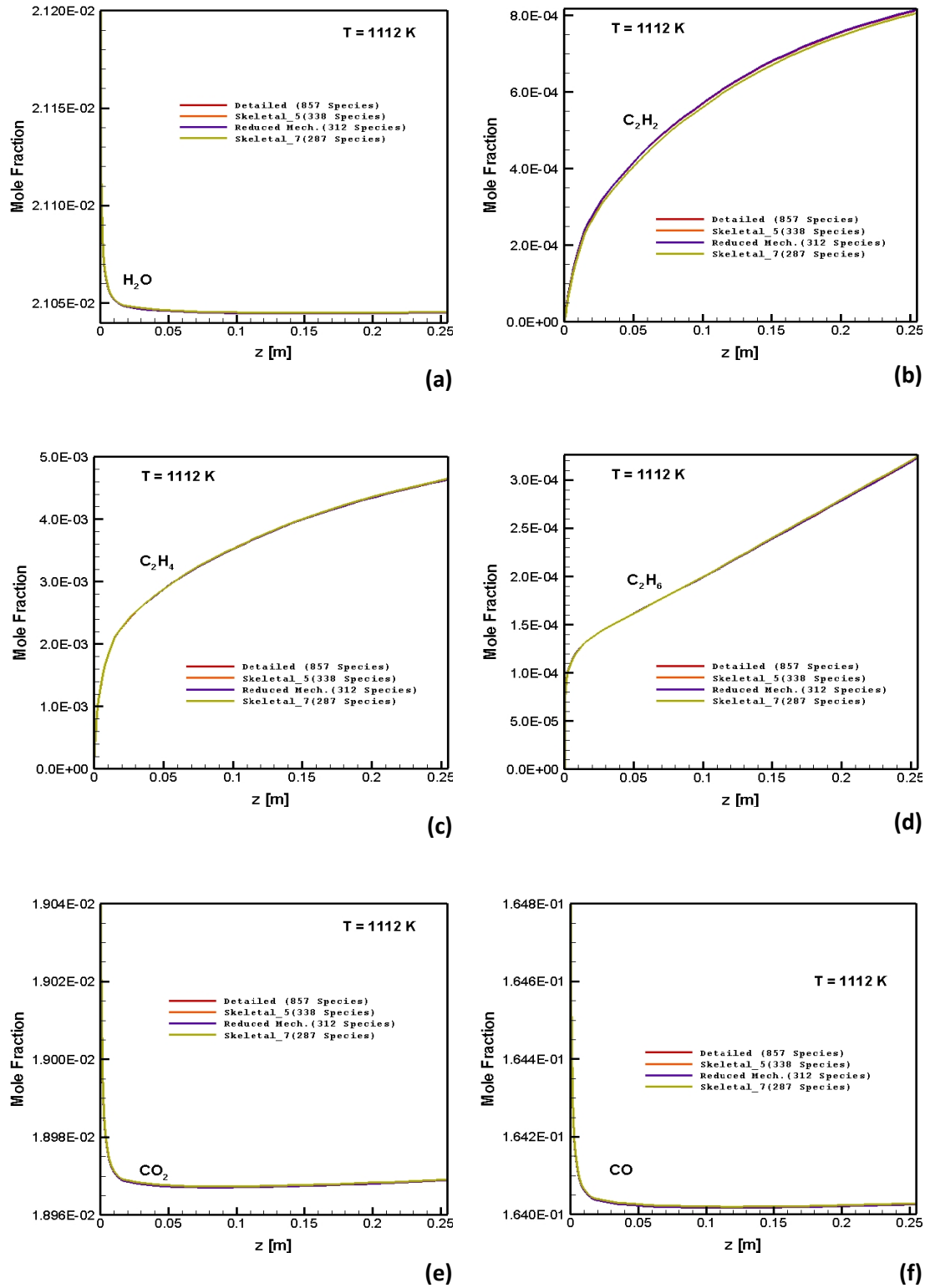
Figure A.11 : Numerically predicted species distribution as a function of axial position along the reactor: C/O=2.0 , 1112 K: (a) H_2O . (b) C_2H_2 . (c) C_2H_4 . (d) C_2H_6 . (e) CO_2 . (f) CO
