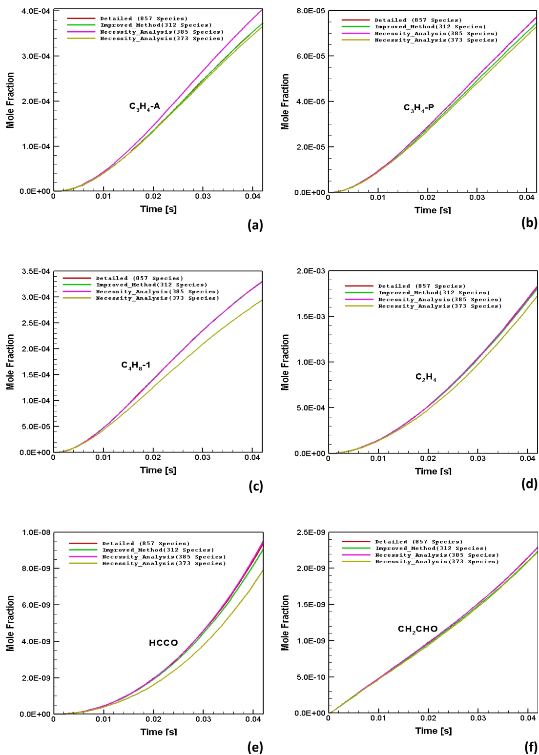
Figure A.7 : Comparison of the necessity analysis method and improved method for numerically predicted species distribution in CPOX of i-octane as a function of time in the batch reactor: C/O=1.6, 1005.78 K: (a) C_3H_4-A . (b) C_3H_4-P . (c) C_4H_8-1 . (d) C_2H_4 . (e) HCCO . (f) CH_2CHO
