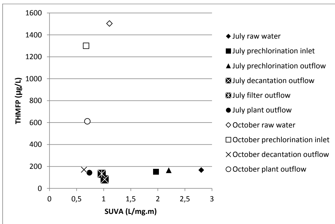
Figure 5.10 : THMFP and SUVA relation for the WTP samples
