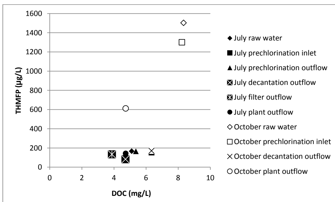
Figure 5.12 : THMFPP and DOC relation for the WTP samples
