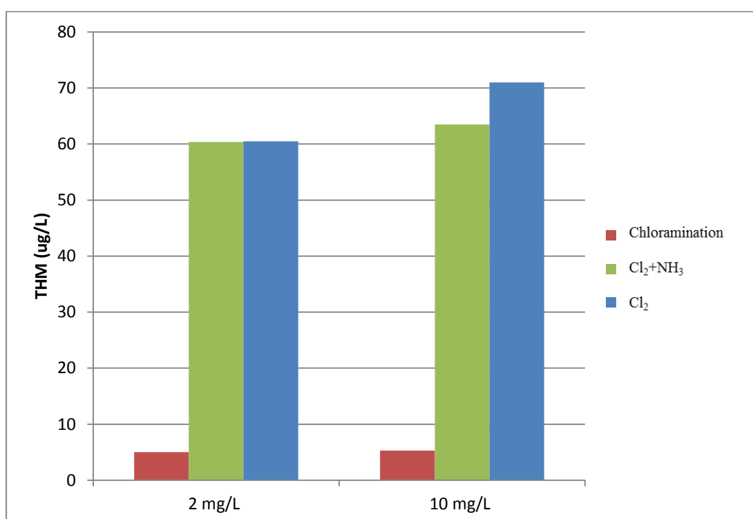
Figure 5.13 : THM concentrations in lake water for different disinfection methods conducted in December
