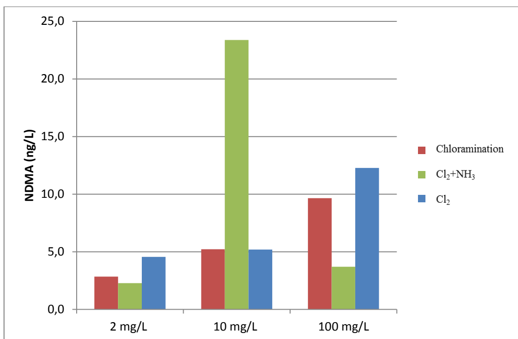
Figure 5.15 : NDMA concentration in lake water for different disinfection methods conducted in December
