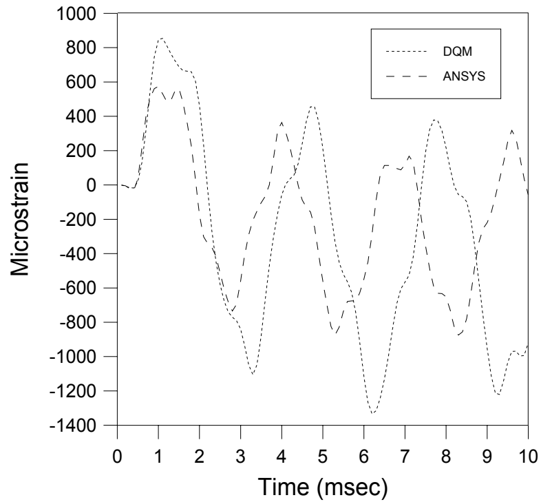
Figure 6.27: Strain-time ( \varepsilon_x ) history of plate centre for the blast-loaded isotropic plate (M1) of variable thickness with clamped boundary condition.
