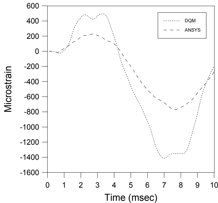
Figure 6.30: Strain-time ( \varepsilon_y ) history of plate centre for the blast-loaded bidirectional laminated composite plate (M3) of variable thickness with simply supported boundary condition.
