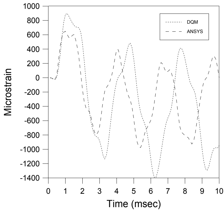
Figure 6.28: Strain-time ( \varepsilon_y ) history of plate centre for the blast-loaded isotropic plate (M1) of variable thickness with clamped boundary condition.
