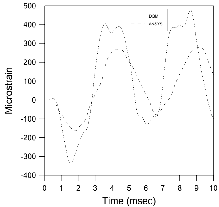
Figure 6.32: Strain-time ( \varepsilon_y ) history of plate centre for the blast-loaded bidirectional laminated composite plate (M3) of variable thickness with clamped boundary condition.
