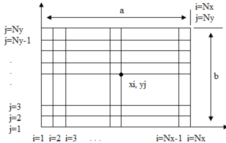
Fig. 2.1 Quadrature grid for a rectangular region
