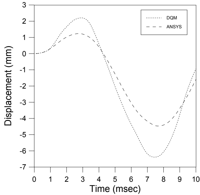
Figure 6.29: Displacement-time history of plate centre for the blast-loaded bidirectional laminated composite plate (M3) of variable thickness with simply supported boundary condition.
