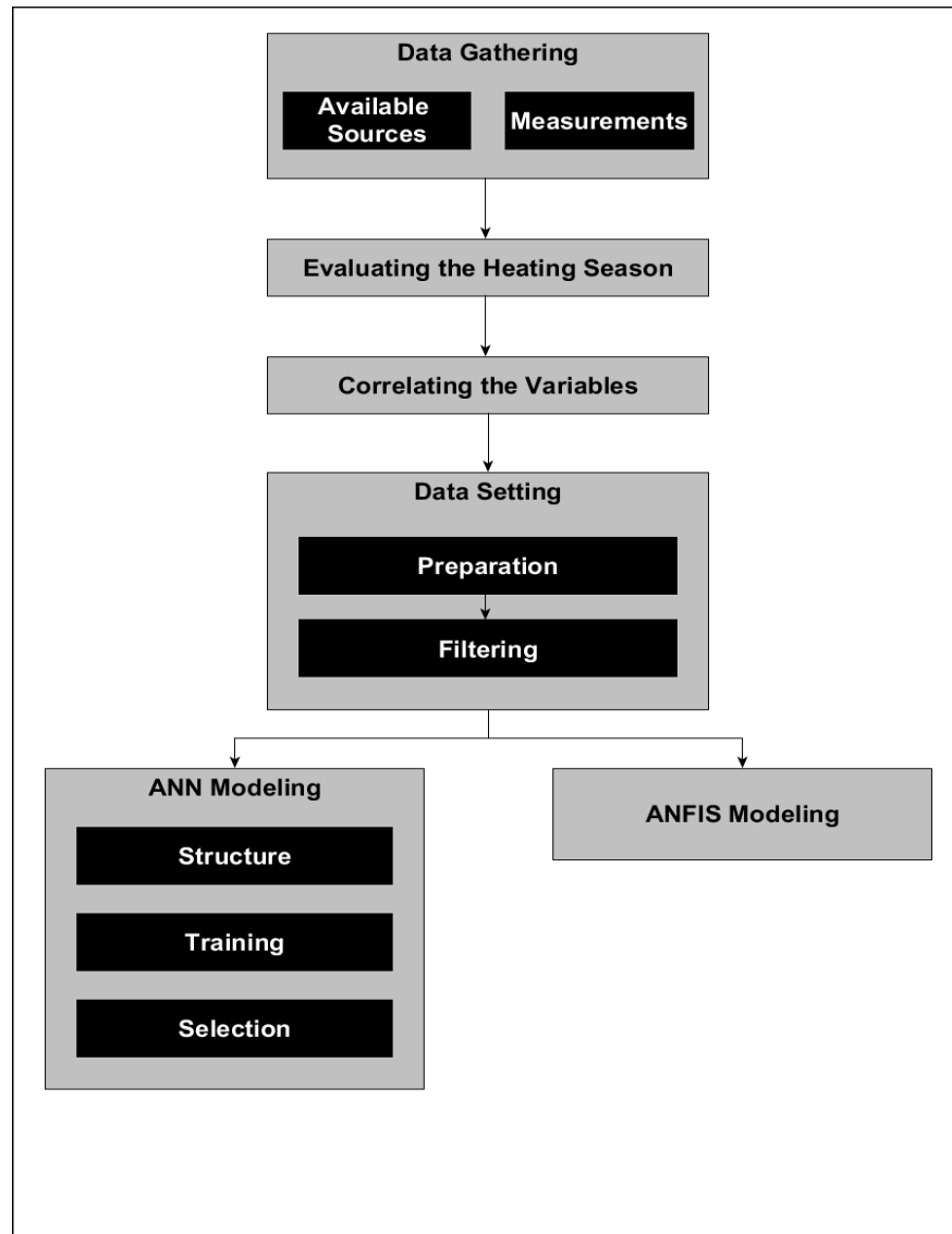
Figure 3.1: Methodology flowchart.
