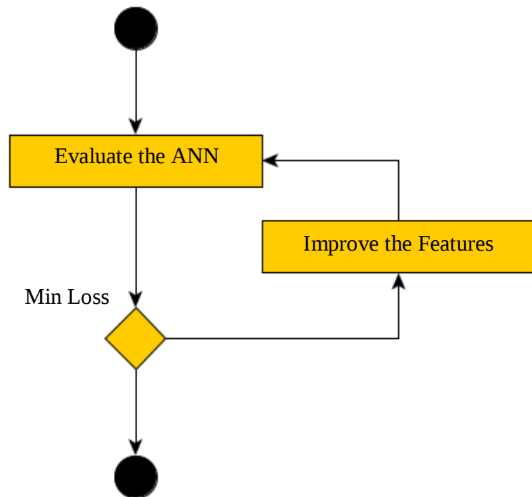
Figure 3.2: Selection model.
