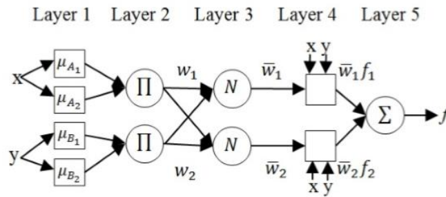
Figure 3.3: Structure of ANFIS. [41]
