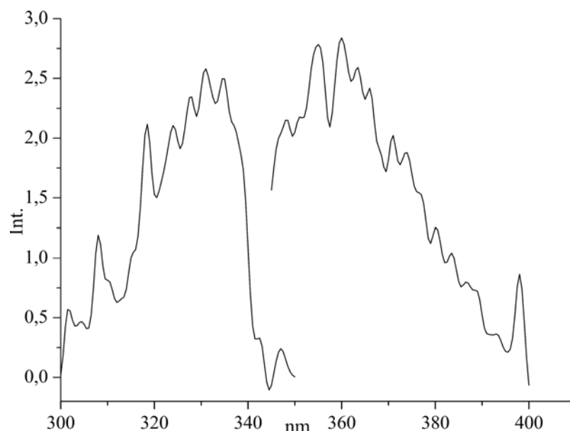
Figure 4.18 : Fluorescence excitation and emission spectra of the naphthoxazine macromonomer in chloroform.
