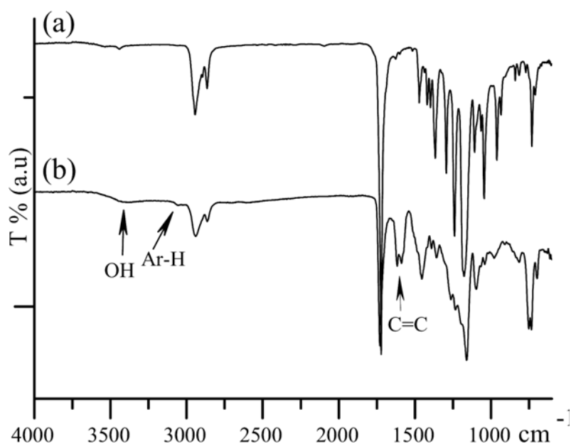
Figure 4.20 : FT-IR spectrum of the cured PCL-N-a (a) and thermally polymerized macromonomer in the absence of added benzoxazine (b).
