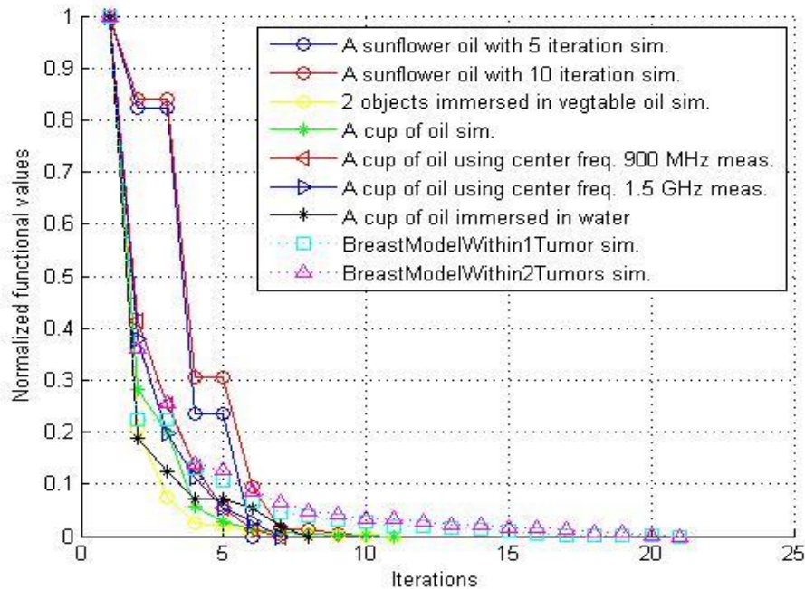
Figure 6.29 : Normalized functional values for 3D reconstruction as a function of iteration number for the simulated and measured data.
