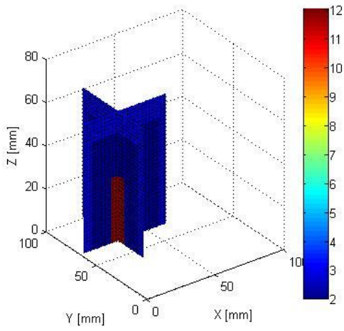
(a) Original \epsilon_r model
