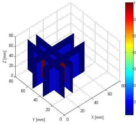
(a) Original \sigma model
