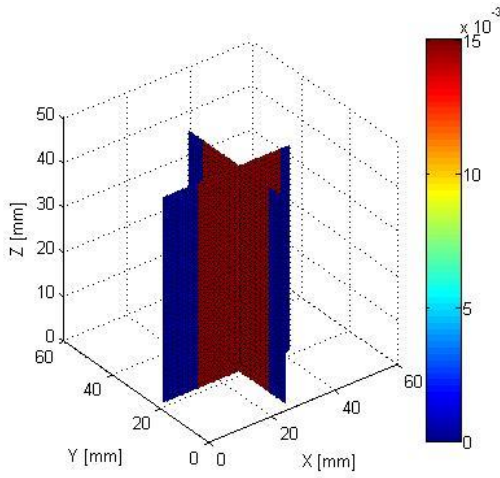
(c) Reconstructed \epsilon_r for measured data at 1.5 GHz
