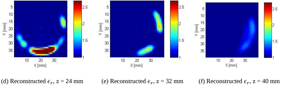
Figure 6.10 : 2D representation of reconstructed images of the single target object using accurate antenna modelling. (a) is the original model of permittivity. (b)-(g) Reconstructed permittivity images of measured data with 6 iteration are shown in different heights using centre frequency 1.5 GHz, FWHM 1.0 GHz.
