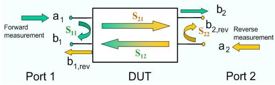
Figure 5.2 : Scattering parameters of a two –port network.
