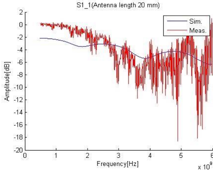
Figure 6.15 : S1_1 parameters for Measured and Simulated data by algorithm (actual length).
