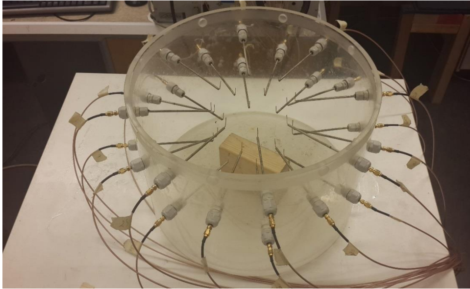
Figure 5.6 : The set up system designed with 24 monopole antenna in cylindrical pattern.
