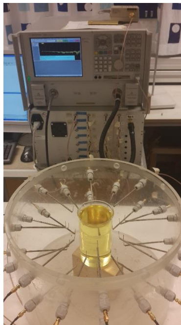
Figure 5.9 : The measurement system connected to VNA including target object.
