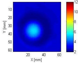
(b) Reconstructed \epsilon_r , z = 8 mm
