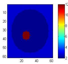
(a) Original permittivity
