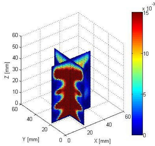
(b) Reconstructed \epsilon_r for simulated data at 1.0 GHz
