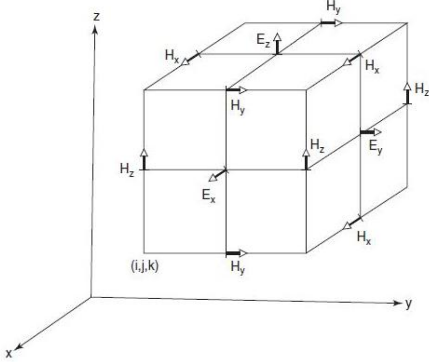
Figure 3.1 : A Yee space lattice, position of electrical and magnetic field vector components in one unit cell.
