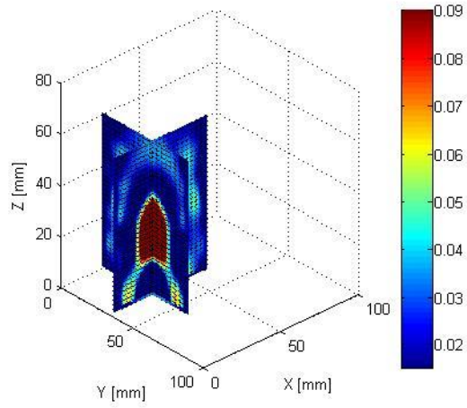
(b) Reconstructed \sigma for simulated data at 1.5 GHz
