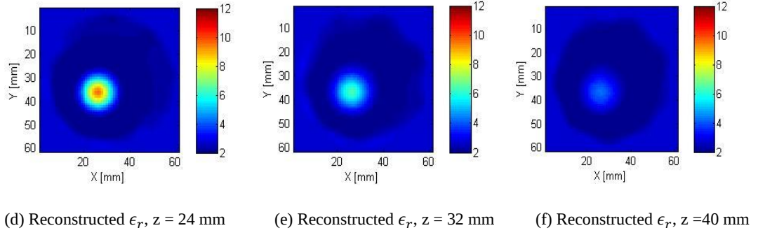
Figure 6.24 : 2D representation of reconstructed images of the simulated breast model within one tumour immersed matching liquid using accurate antenna modelling. (a) is the original model of permittivity. (b)-(g) Reconstructed permittivity images of simulated data with 20 iteration are shown in different heights using centre frequency 1.5 GHz and FWHM 1.0 GHz.
