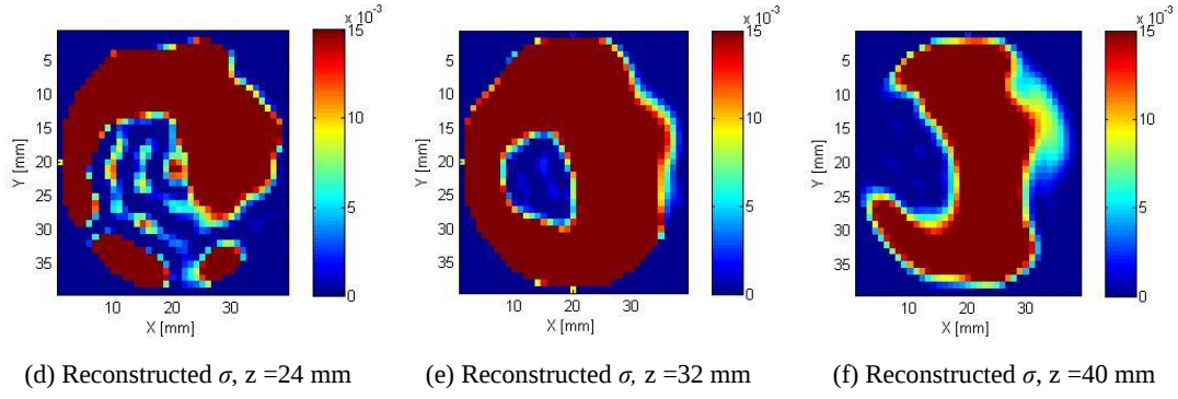
Figure 6.13 : 2D representation of reconstructed images of the single target object using accurate antenna modelling. (a) is the original model of conductivity. (b)-(g) Reconstructed conductivity images of measured data with 6 iteration are shown in different heights using centre frequency 1.5 GHz, FWHM 1.0 GHz.
