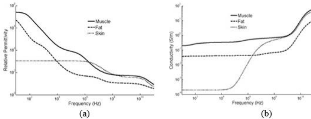
Figure 2.1 : Curves for complex permittivity of different human tissues at 37°C, modelled by Cole-Cole equation, investigated by Mohammad Mahfuz [28].(a) Relative permittivity, (b) conductivity.
