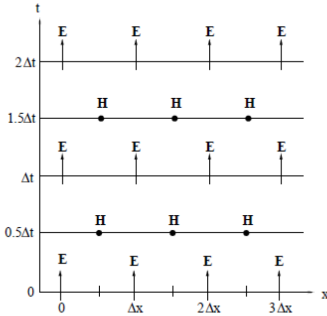
Figure 3.2 : The FDTD time stepping for E- and H-fields.
