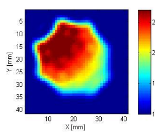
(b) Reconstructed \epsilon_r , z = 8 mm
