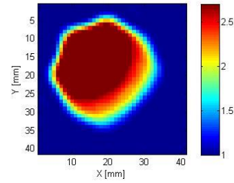
(c) Reconstructed \epsilon_r , z = 16 mm
