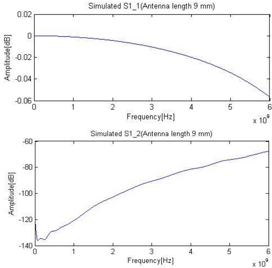
Figure 5.3 : Simulated S1_1 and S1_2 parameters with antenna length of 9 mm and radius 0.2 mm.
