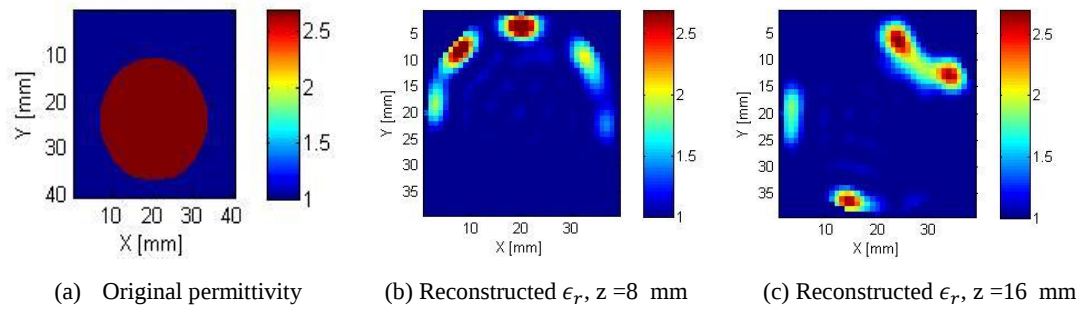
Figure 6.9 : 2D representation of reconstructed images of the single target object using accurate antenna modelling. (a) is the original model of permittivity. (b)-(g) Reconstructed permittivity images of simulated data with 10 iteration are shown in different heights using centre frequency and FWHM 1.0 GHz.
