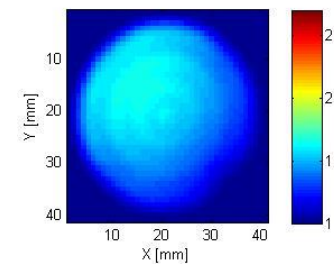
(f) Reconstructed \epsilon_r , z = 40 mm
