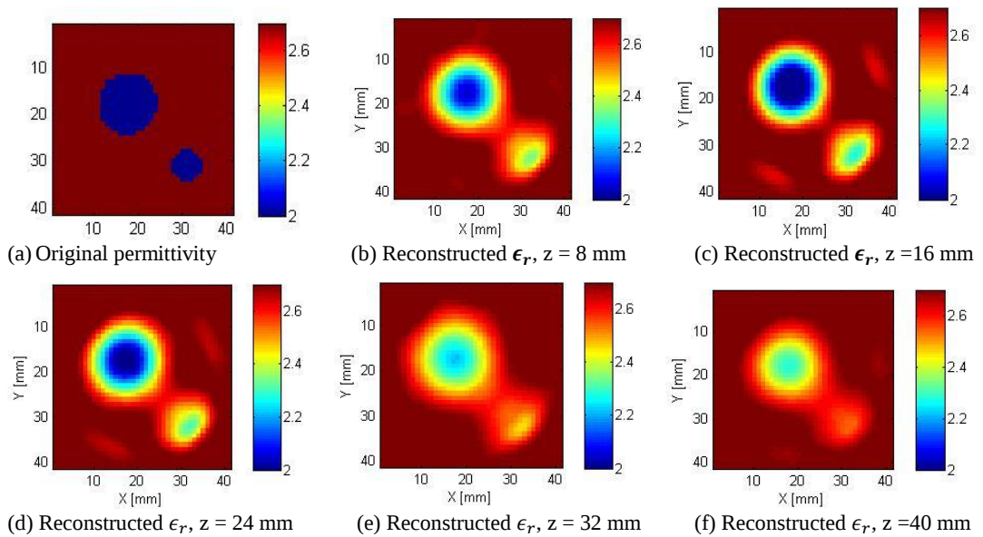
Figure 6.20 : 3D representation of the original model and simulated reconstruction.
