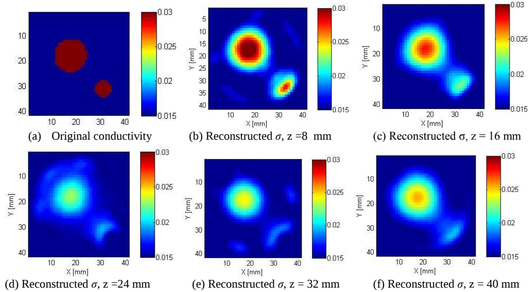
Figure 6.22 : 2D representation of reconstructed images of the two target objects
