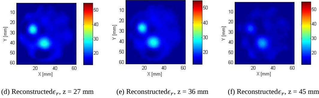
Figure 6.27 : 2D representation of reconstructed images of the simulated breast model within one tumour immersed in matching liquid using accurate antenna modelling. (a) is the original model of permittivity. (b)-(g) Reconstructed permittivity images of simulated data with 20 iteration are shown in different heights using centre frequency and FWHM 900 MHz.
