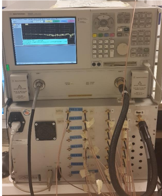
Figure 5.5 : The switching matrix connected to VNA.
