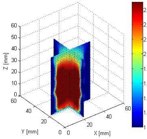
(c) Original \sigma model
