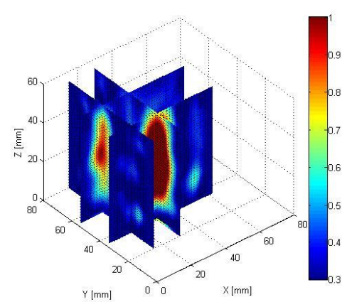
(b) Reconstructed \sigma for simulated data at 900 MHz
