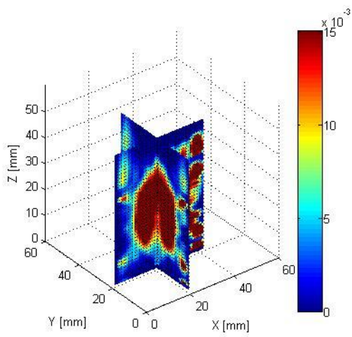
(d) Reconstructed \epsilon_r for measured data at 900 MHz
