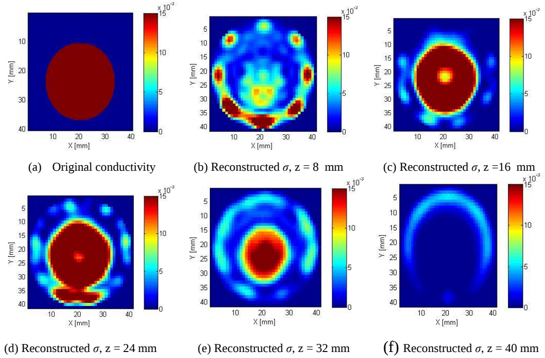
Figure 6.12 : 2D representation of reconstructed images of the single target object
