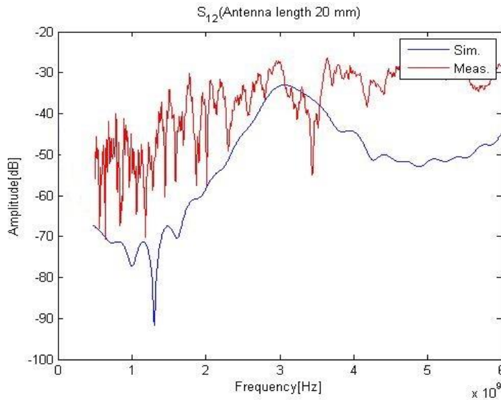
Figure 6.16 : S1_2 parameters for Measured and Simulated data by algorithm (actual length).
