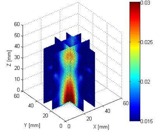
(b) Reconstructed \sigma for simulated data at 1.0 GHz
