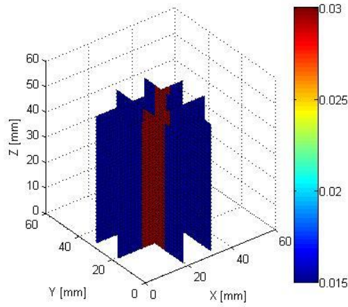
(a) Original \sigma model
