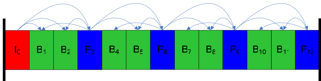
Figure 5.5: Display Order
