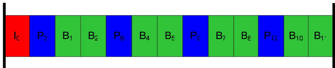
Figure 5.6: Coded Order
