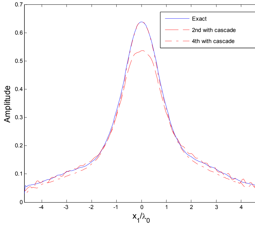
Figure 4.10 : Comparison of normal derivatives of the fields at the lower boundary of the thin layer applying cascaded TLC for Example 4.1.2
