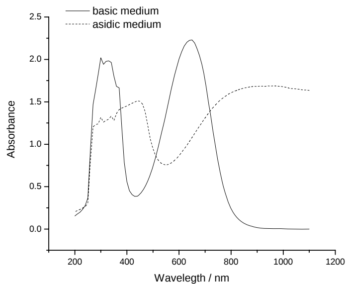
Figure A.6: UV-visible spectra of PANI-HCl sample in the basic and acidic medium.
