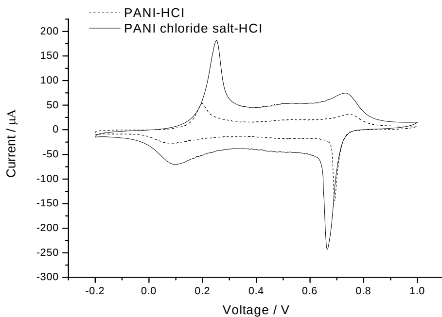
Figure A.5: The comparison of CV of PANI-HCl and PANI-HCl grown applying 16 cycles at the 100mV/s scan rate
