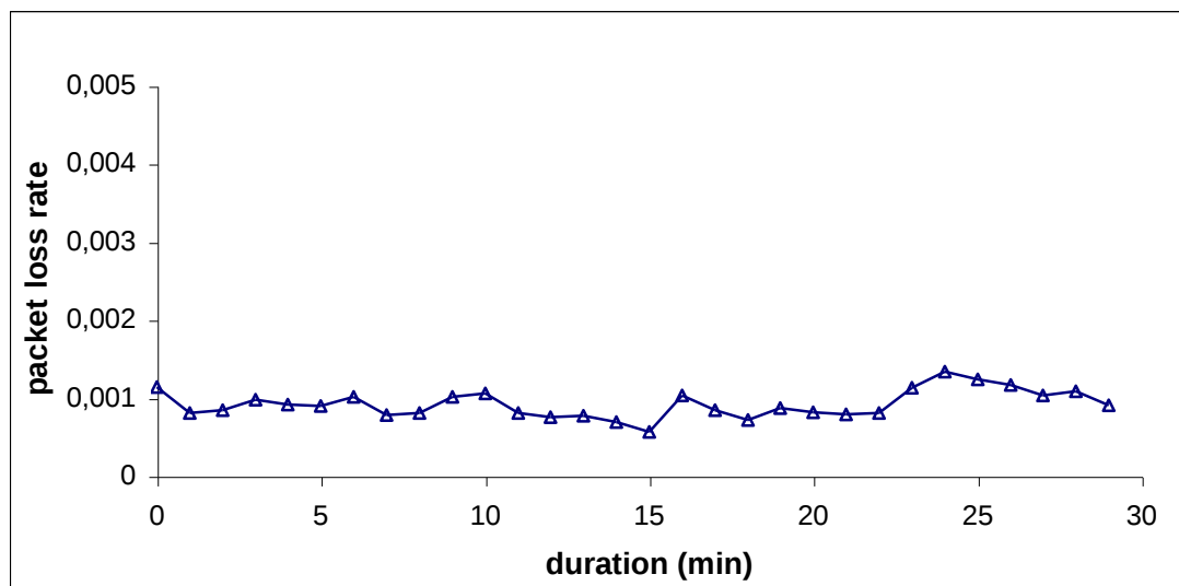
Figure 6.12 Packet lost rate for Scenario-3.
