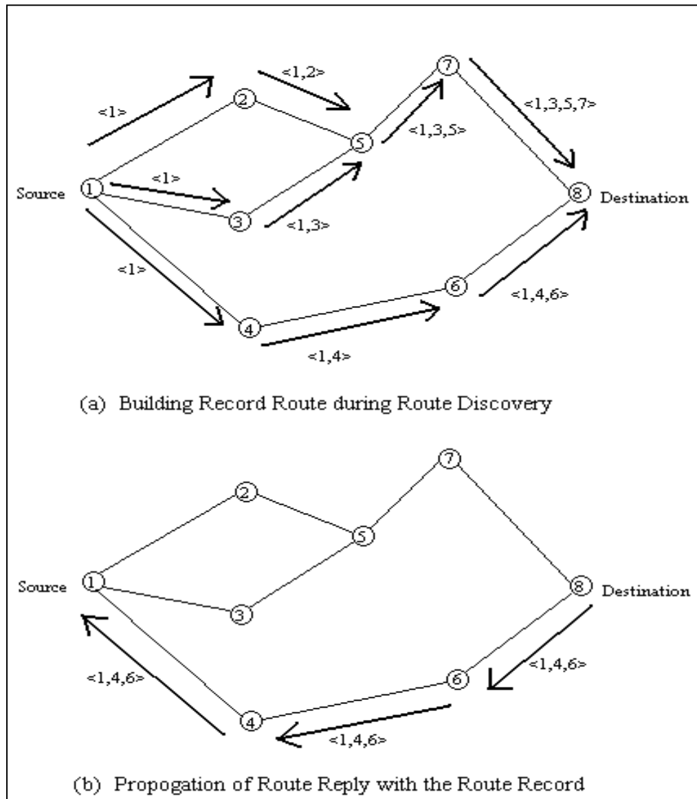
Figure 3.9 Creation of record route in DSR protocol.
