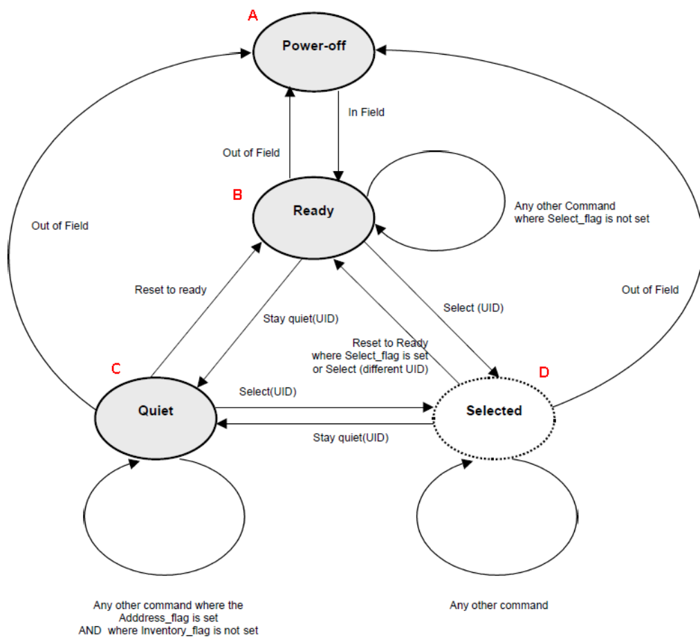
Figure 2.7: The States of a RFID Tag
