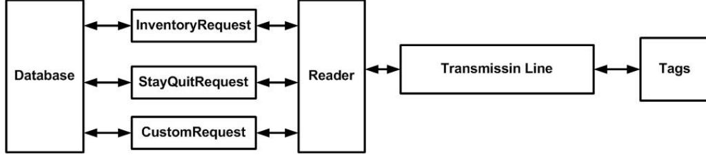
Figure 2.10: The Detailed Structure of PETRA
