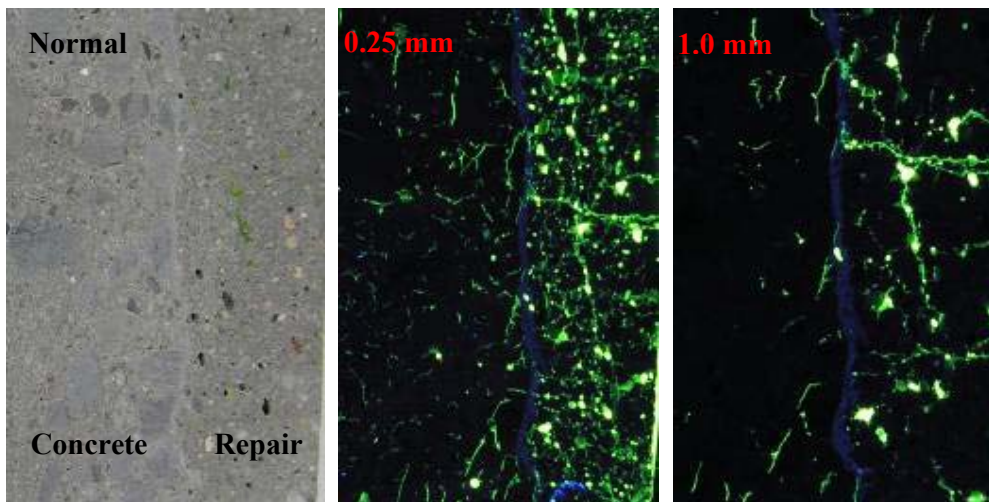
Figure 7.6 : Plane Section Pictures B88 with Epoxy Primer
