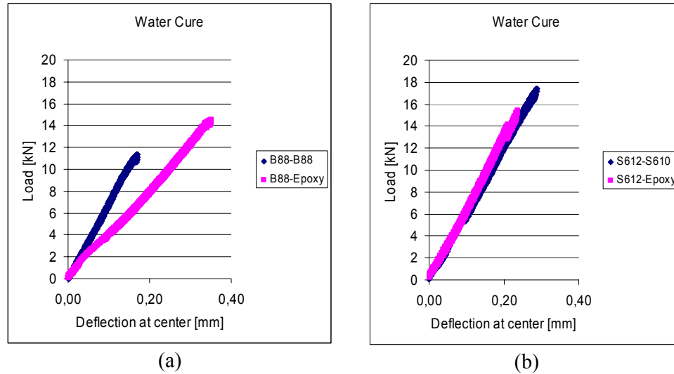
Figure 6.13 : Load Deflection of B88 Composite Beam in Water Curing
