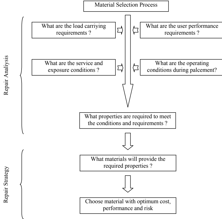
Figure 4.3 : The Selection Process for a Repair Material [1]
