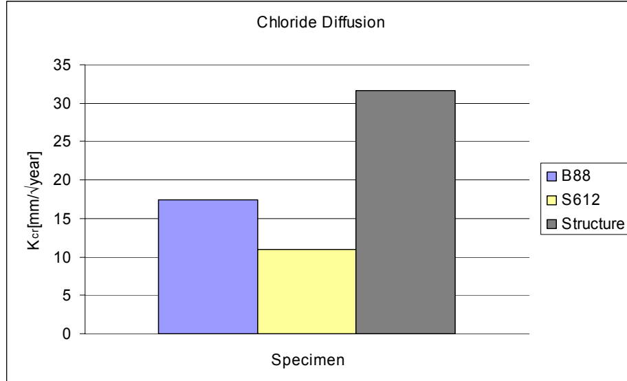
Figure 6.9 : Penetration Parameter, K_{Cr}
