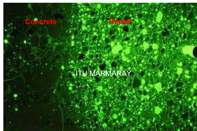
Figure 7.11 : S612 with S610 Primer Thin Section, 35x45 mm
