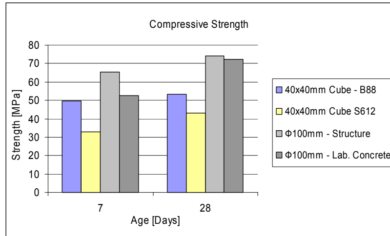
Figure 6.3 : Difference in Compressive Strength Results
