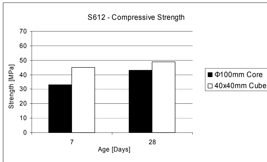
Figure 6.2 : Size Effect on S612 Repair Mortar
