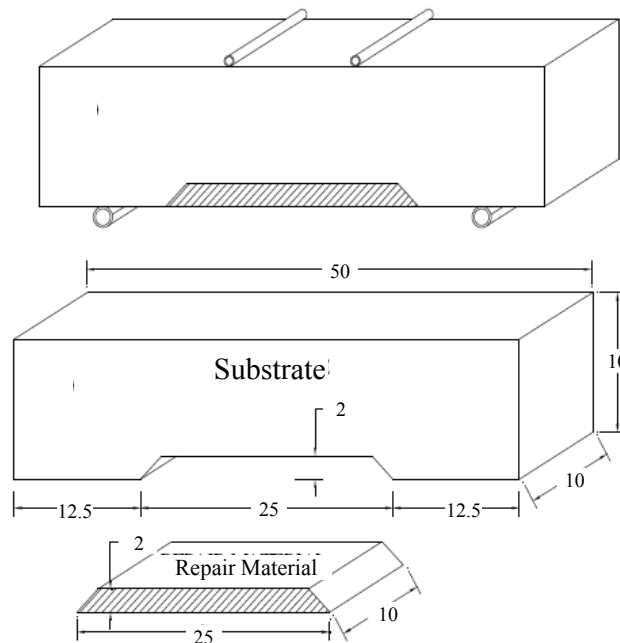
Figure 4.8 : Composite Beam Test Specimen (dimensions in cm) [7]
