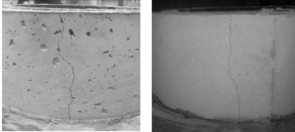
Figure 6.6 : Ring Test, B88 and S612
