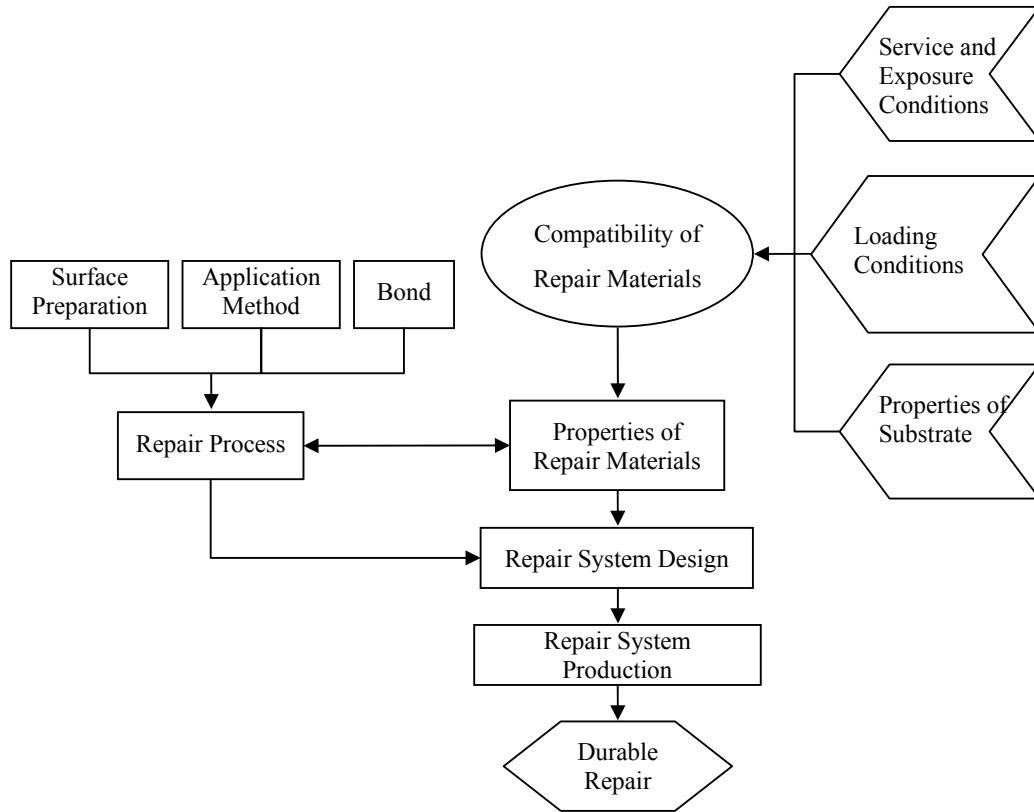
Figure 4.1 : Factors Affecting the Durability of Concrete Repair Systems [16]
