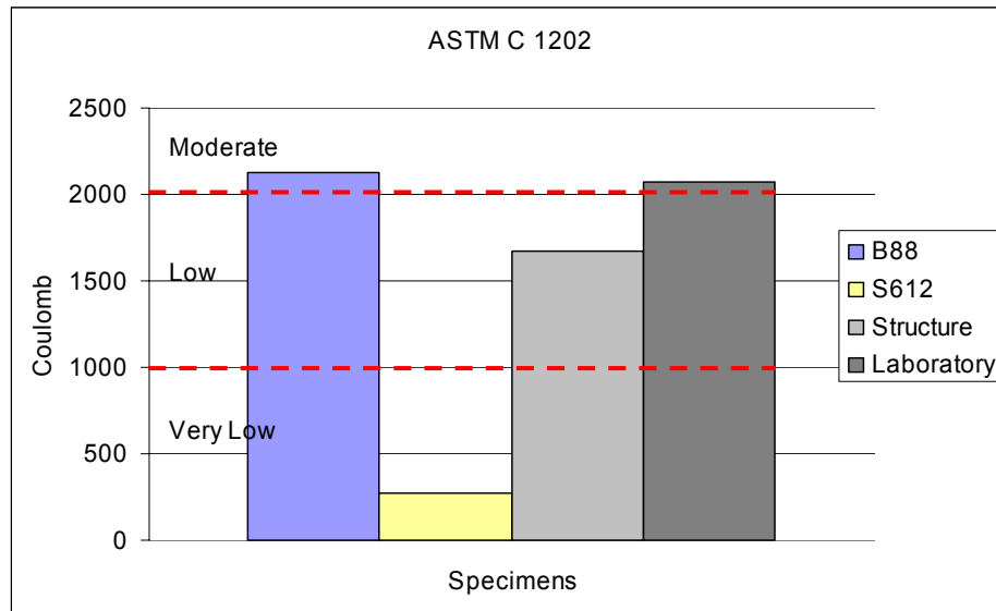
Figure 6.8 : Rapid Chloride Test Results
