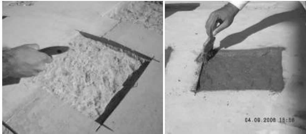
Figure 5.5 : Preparation of the Repair Surface and Application of the Primer
