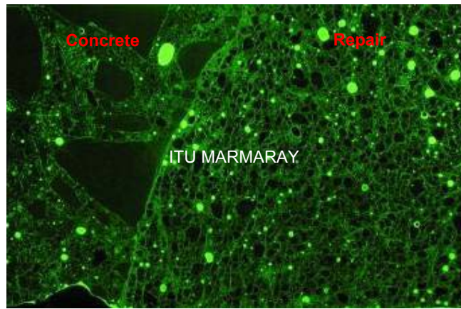
Figure 7.9 : B88 with B88 Primer Thin Section, 30x45 mm
