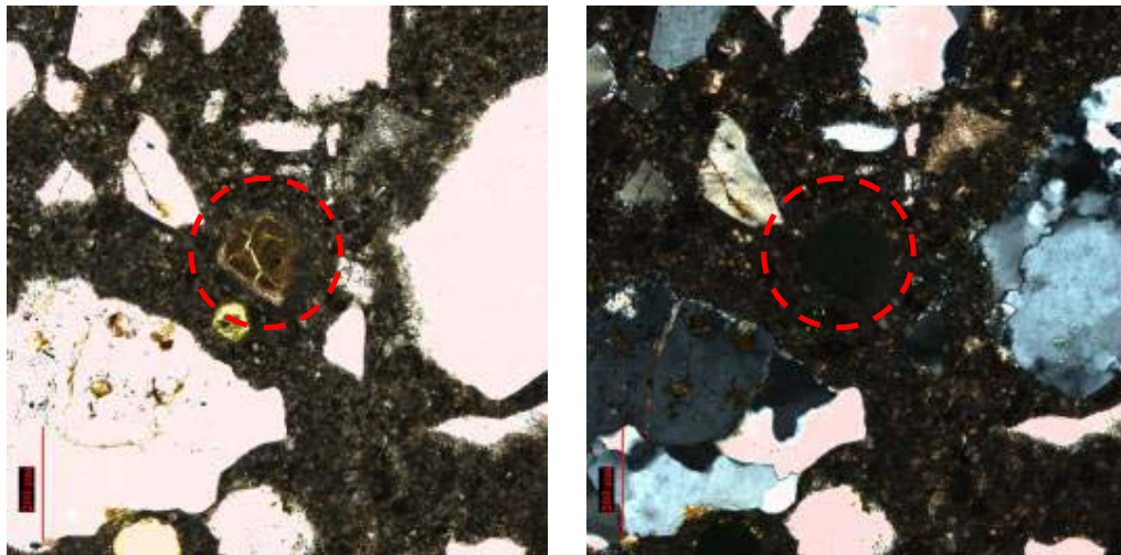
Figure 7.17 : Undispersed Silica-Fume Particle
