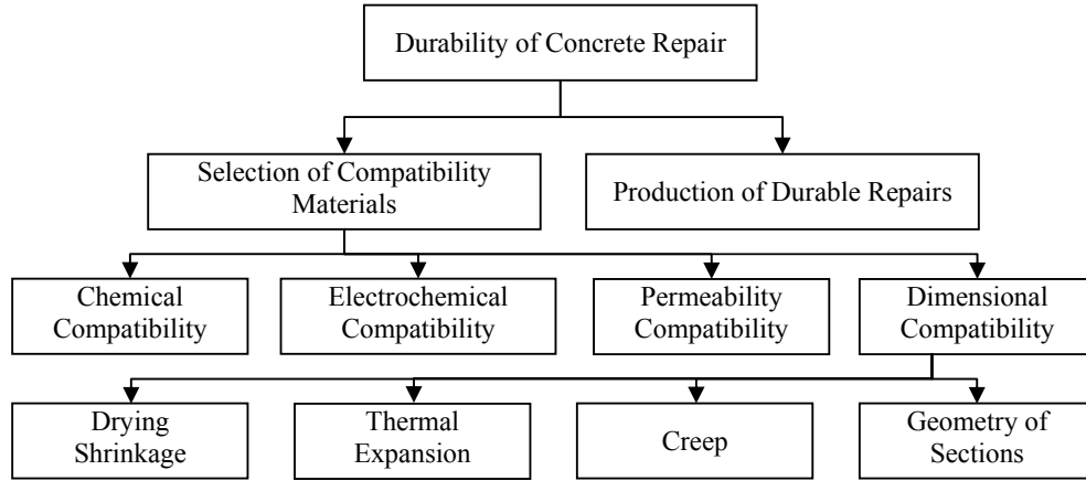
Figure 4.2 : Durability of Concrete Repairs due to Compatibility [15]
