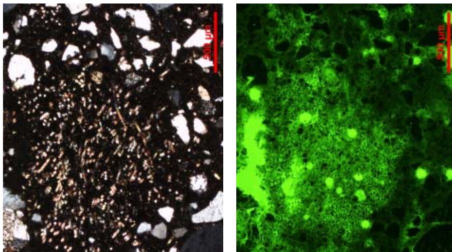
Figure 7.18 : Clump of Fibers in the Matrix
