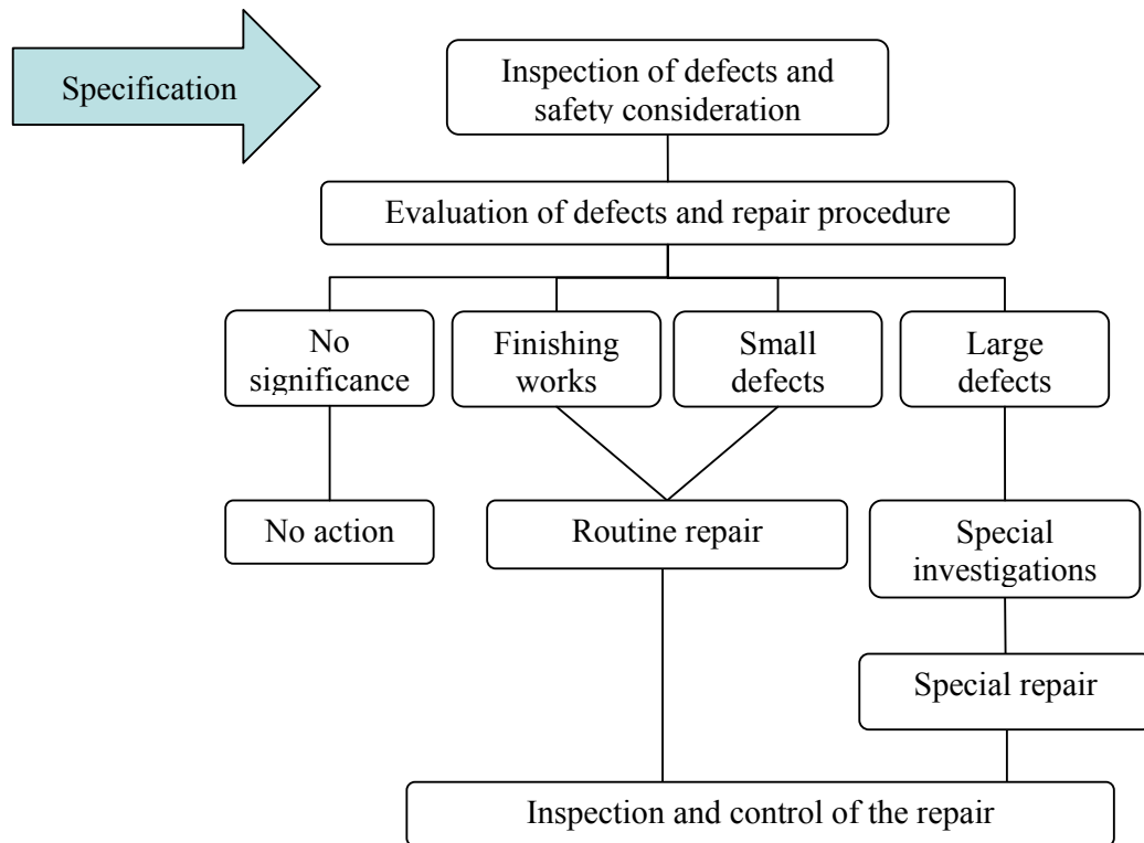
Figure 1.2: Procedure for Repair Management [43, 44]
