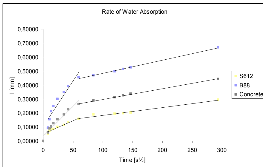
Figure 6.7 : The Average Capillary Water Absorption
