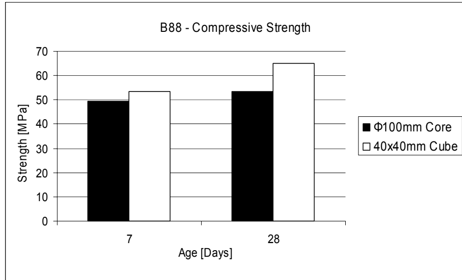
Figure 6.1 : Size Effect on B88 Repair Mortar
