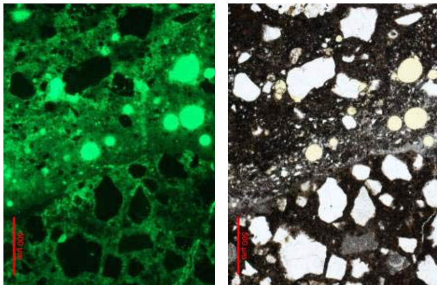
Figure 7.16 : Interface of Repair S612 with Epoxy Primer
