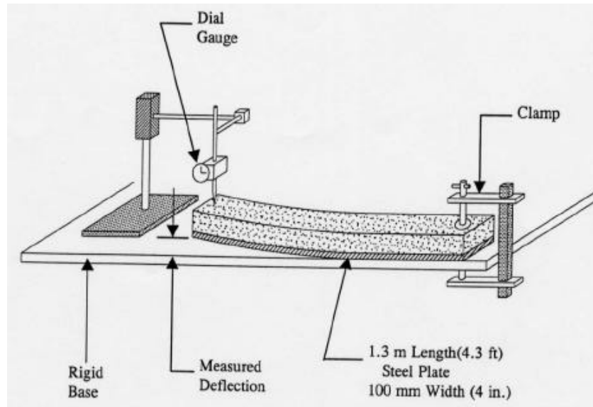
Figure 4.5 : SPS Plate Test [9]
