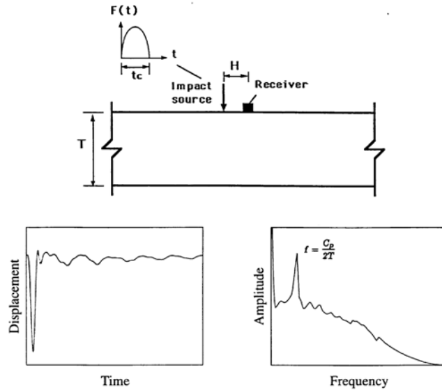
Figure 4.12 : Impact-echo Test, Displacement Waveform, Amplitude Spectrum [20]
