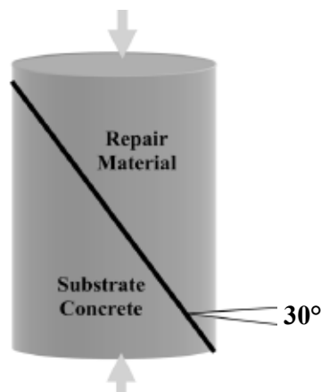
Figure 4.11 : Slant Shear Test Setup [13]
