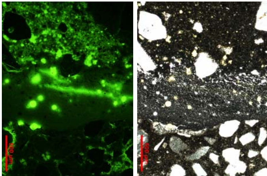
Figure 7.14 : Interface of Repair B88 with Epoxy Primer
