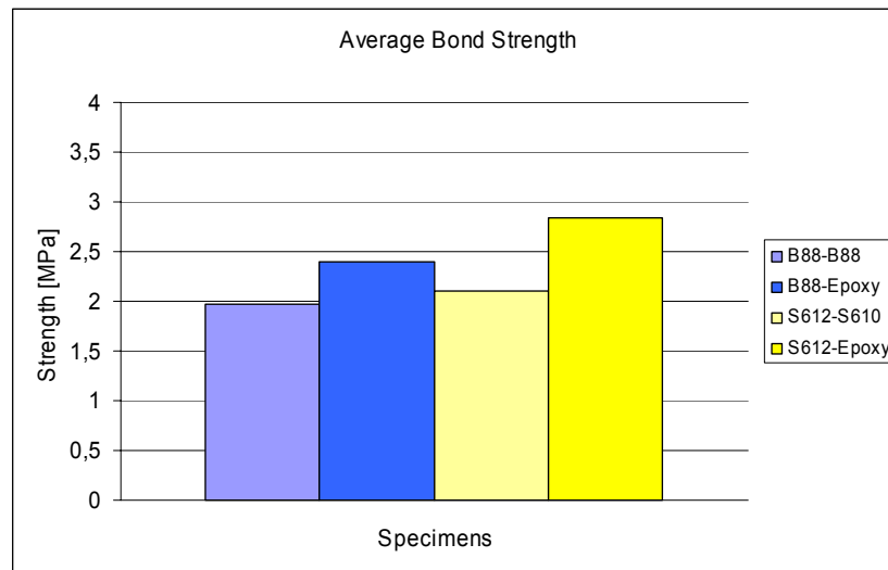
Figure 6.15 : Average Bond Strengths
