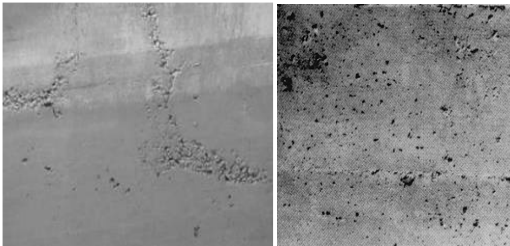
Figure 2.5 : Honeycombing and Bug Holes on the Surface [2]
