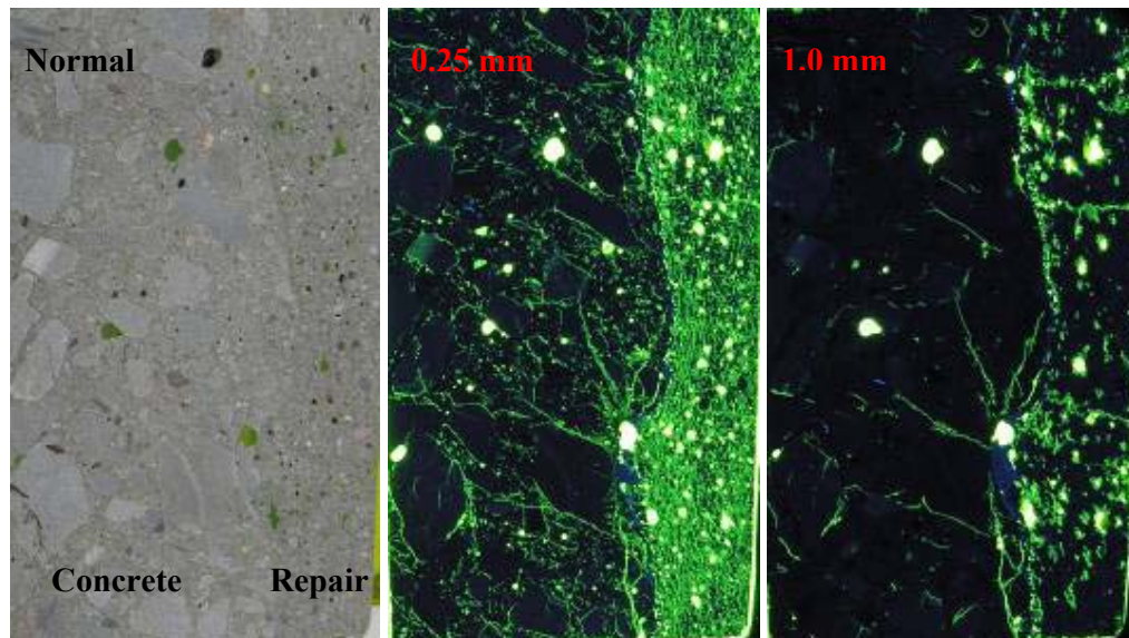
Figure 7.8 : Plane Section Pictures S612 with Epoxy Primer
