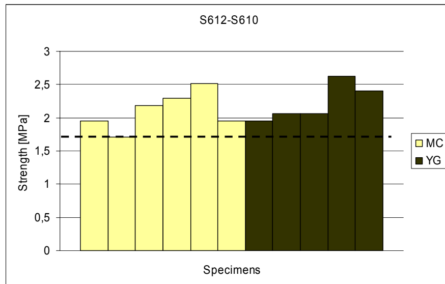
Figure 6.18 : Effect of Workmanship on S612 Repair with Cementitious Primer
