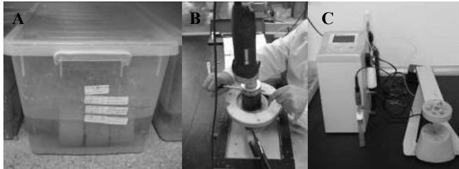
Figure 5.2 : Chloride Diffusion Test Procedure. A- NaCl Exposure, B- Powder Grinding, C- Potentiometric Titration
