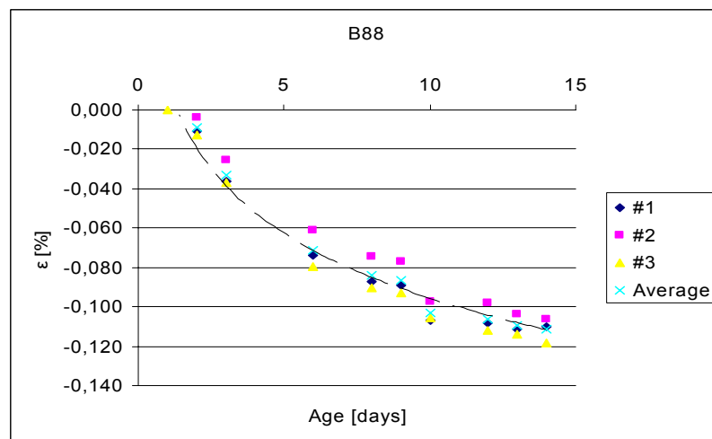
Figure 6.4 : Autogenous Shrinkage Test Results of B88
