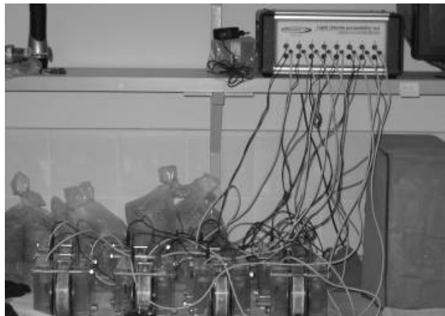
Figure 5.1 : ASTM C1202 Test Setup
