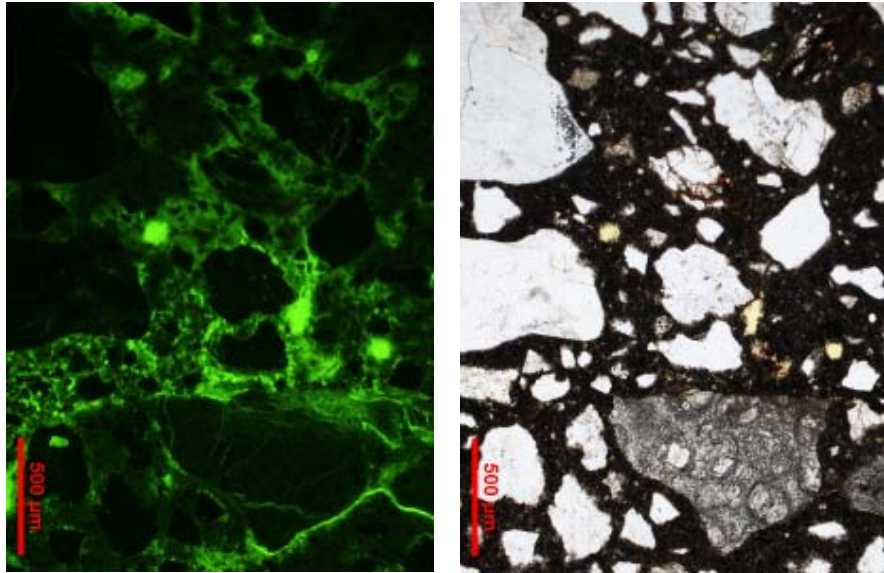
Figure 7.15 : Interface of Repair S612 with S610 Primer
