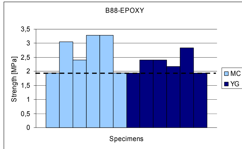
Figure 6.17 : Effect of Workmanship on B88 Repair with Epoxy Primer
