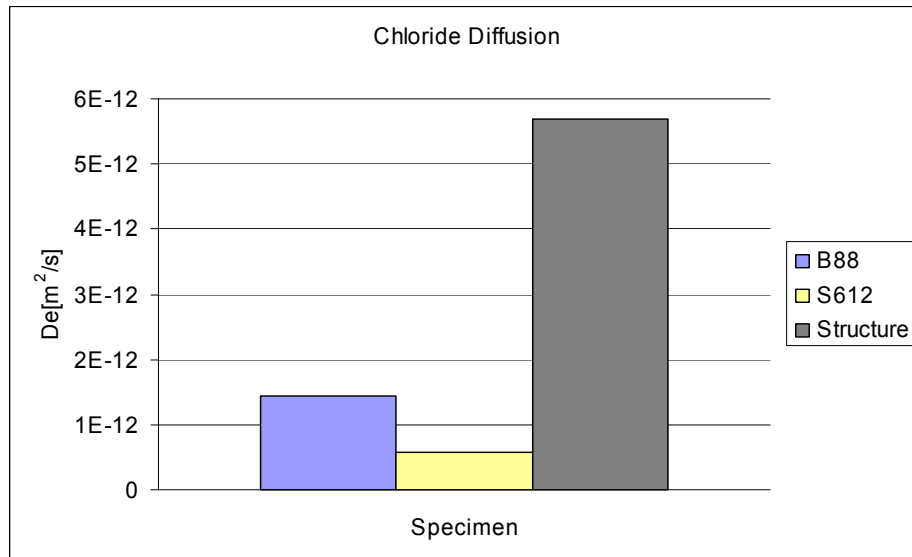
Figure 6.10 : Transport Coefficient, D_e
