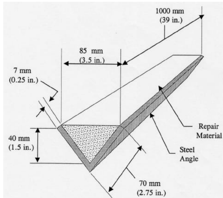
Figure 4.6 : German Angle Test [9]
