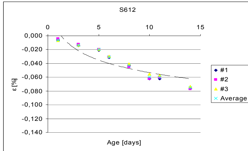
Figure 6.5 : Autogeneous Shrinkage Test Results of S612
