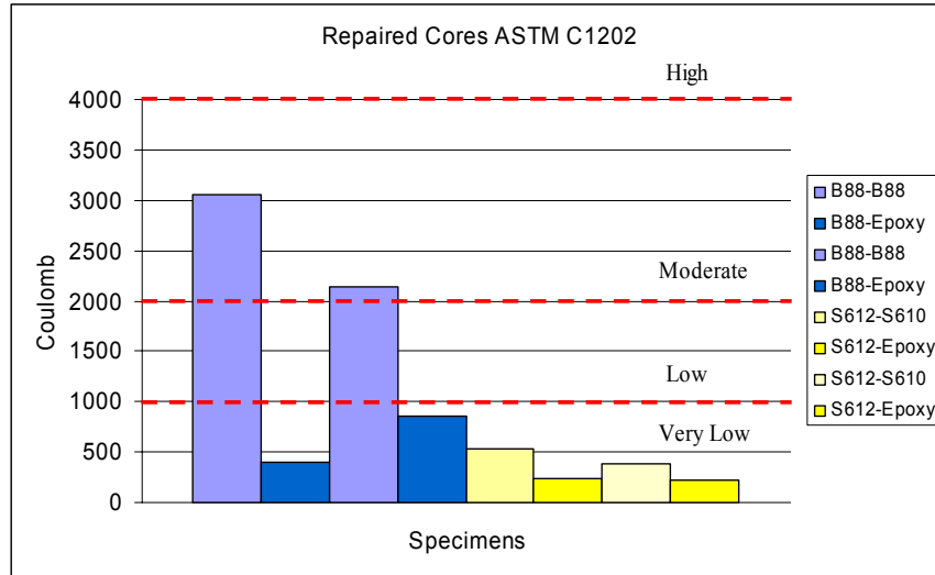
Figure 6.11 : Composite Cores Test Results
