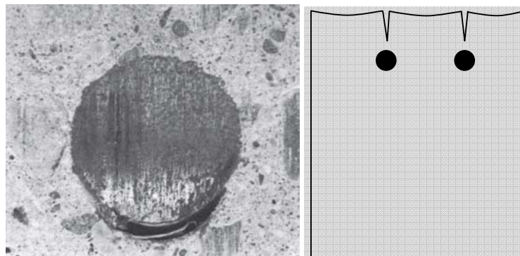
Figure 2.2: Void Under Rebar, Plastic Settlement Over Rebars [1]
