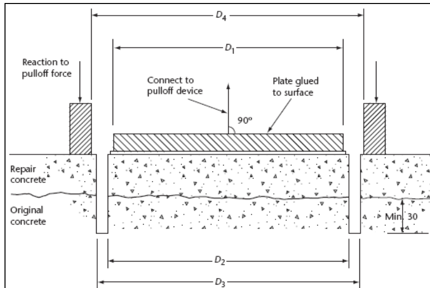
Figure 4.10 : Pull-Off Test (dimensions in mm) [24]
