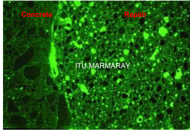
Figure 7.12 : S612 with Epoxy Primer Thin Section, 35x45 mm
