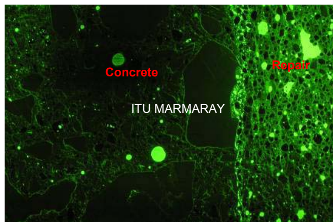
Figure 7.10 : B88 with Epoxy Primer Thin Section, 35x45 mm
