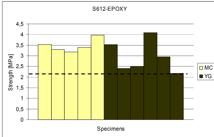
Figure 6.19 : Effect of Workmanship on S612 Repair with Epoxy Primer
