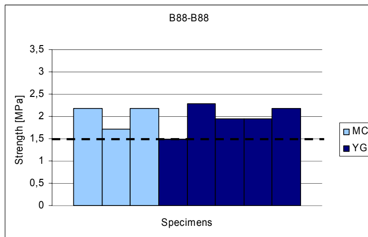
Figure 6.16 : Effect of Workmanship on B88 Repair with Cementitious Primer
