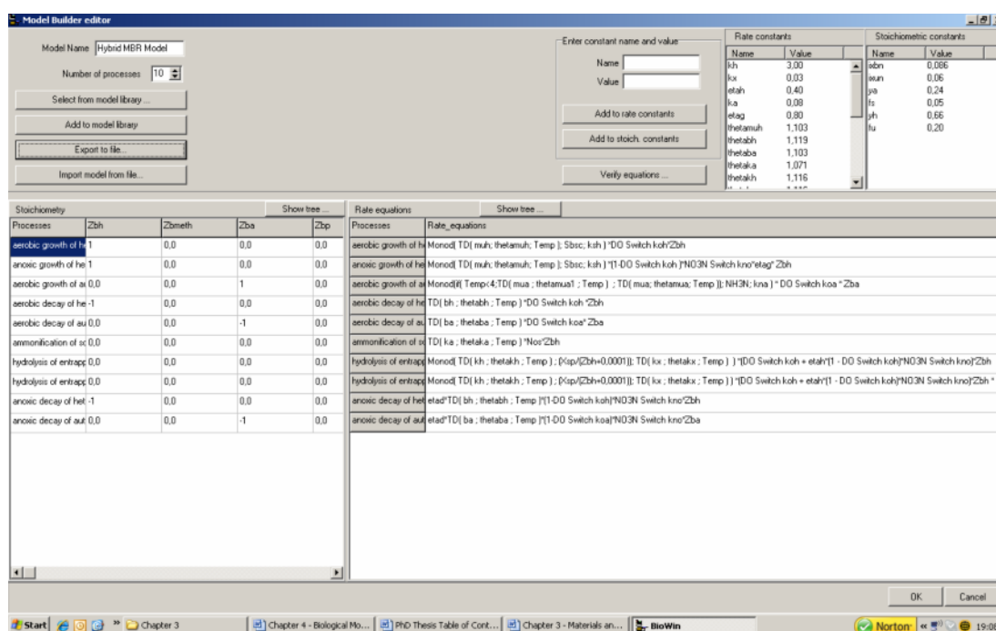
Figure 4.11: Model builder unit in BioWin for implementing the new adopted MBR process matrix
