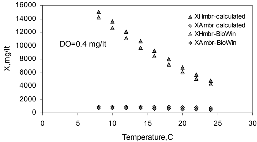
Figure 5.8: Variation of active biomass concentration with respect to changing temperature
