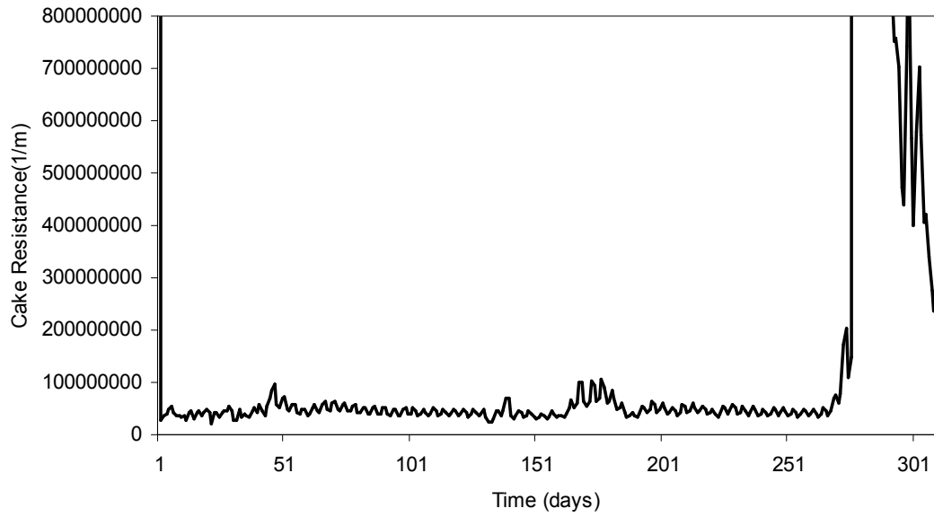
Figure 5.42: Simulated cake resistance
