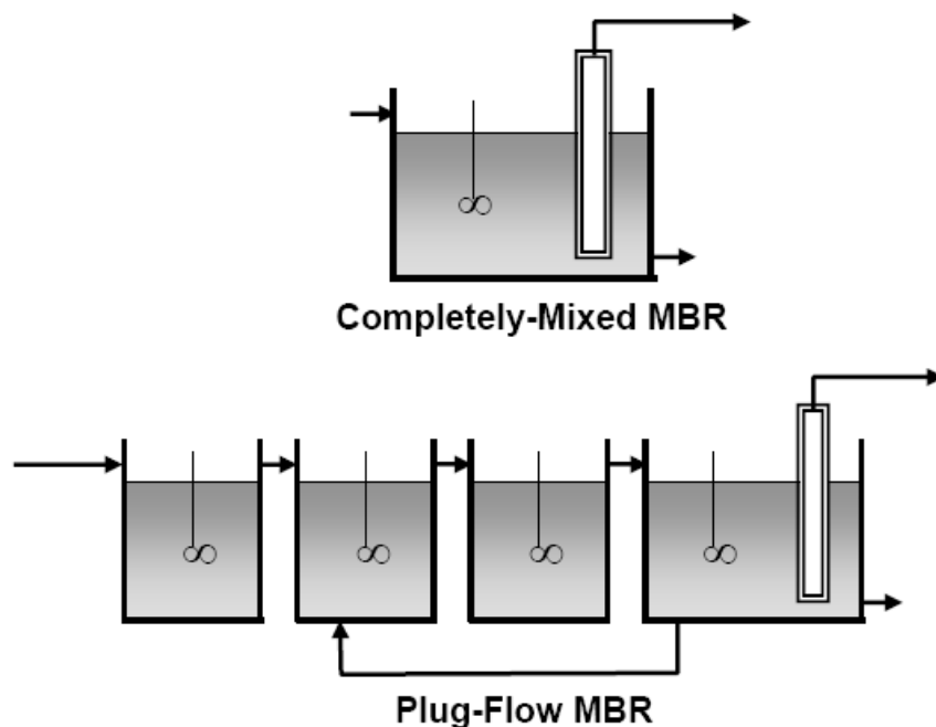
Figure 4.13: Membrane bioreactor model structures
