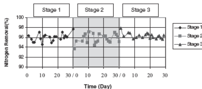
Figure 2.17: Nitrogen removal in intermittent MBR (Ujang et al., 2002)
