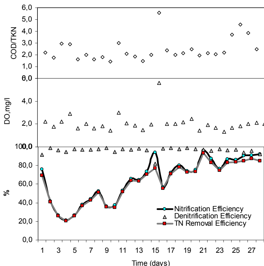
Figure 5.23: Efficiencies nitrification, denitrification and total nitrogen
