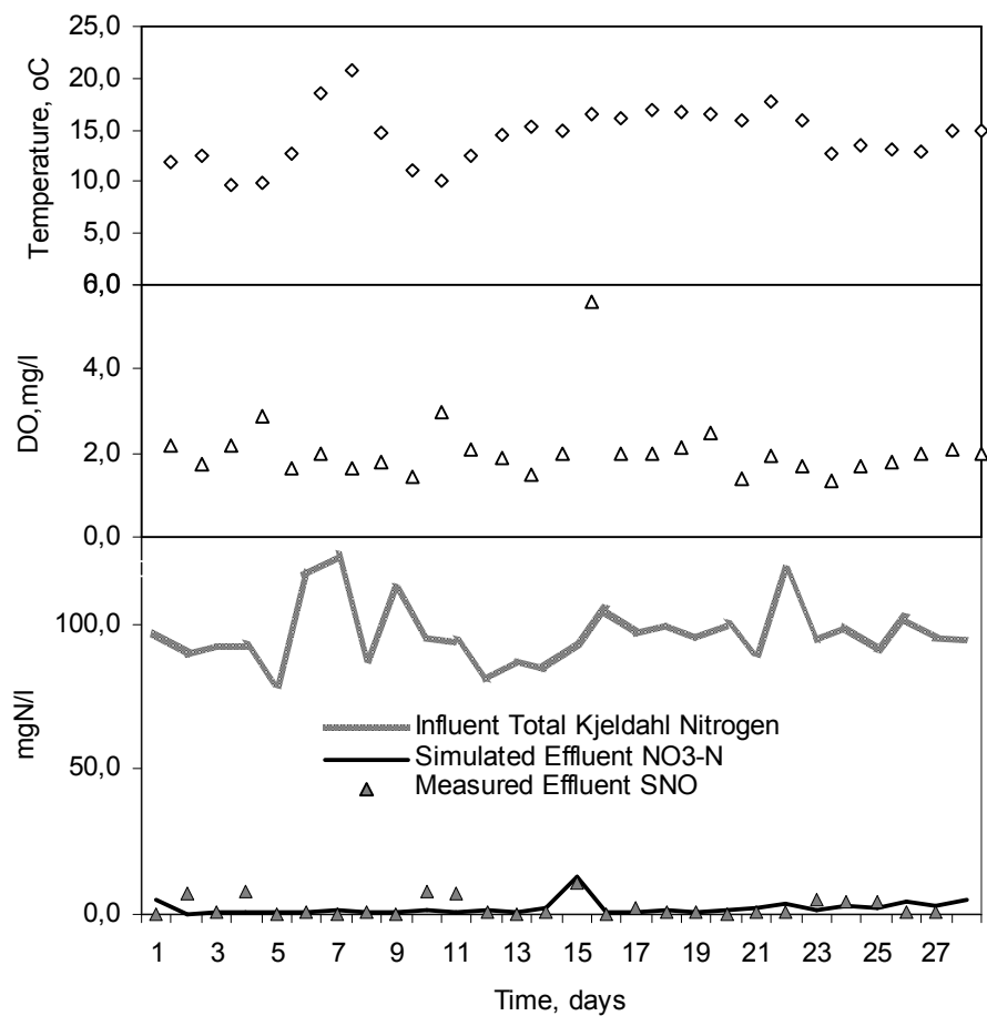
Figure 5.22: Nitrate ( S_{NO} ) profile for Run II
