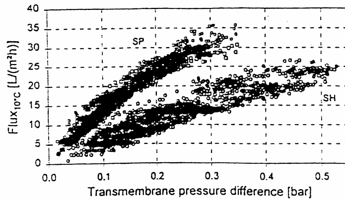
Figure 2.20: Relationship between transmembrane pressure and flux at 10°C (Günder, 2001)
