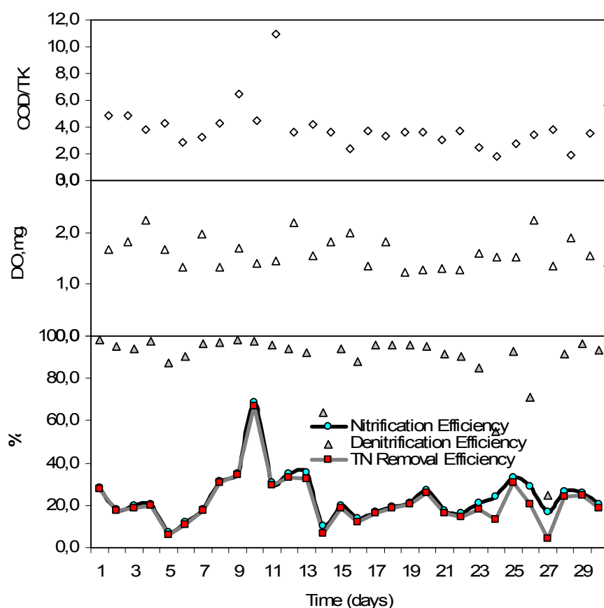
Figure 5.35: Nitrification and denitrification efficiencies
