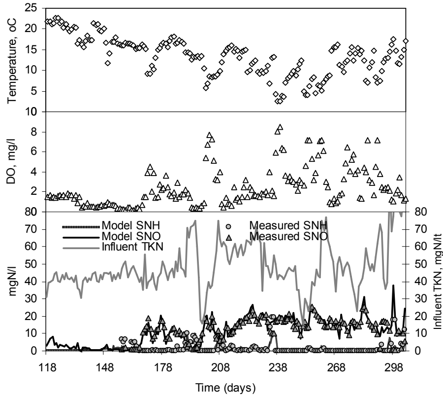
Figure 5.16: Dynamic simulation results and experimental data for S_{NH} and S_{NO}
