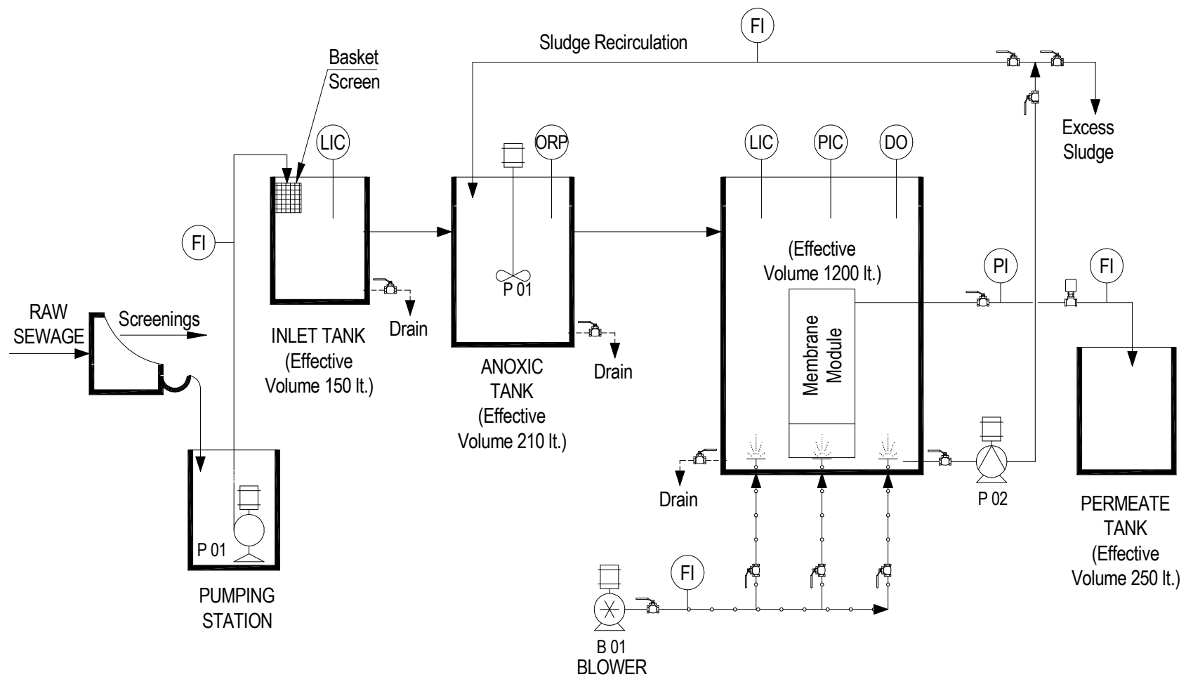
Figure 3.5: Schematic setup of the pilot plant
