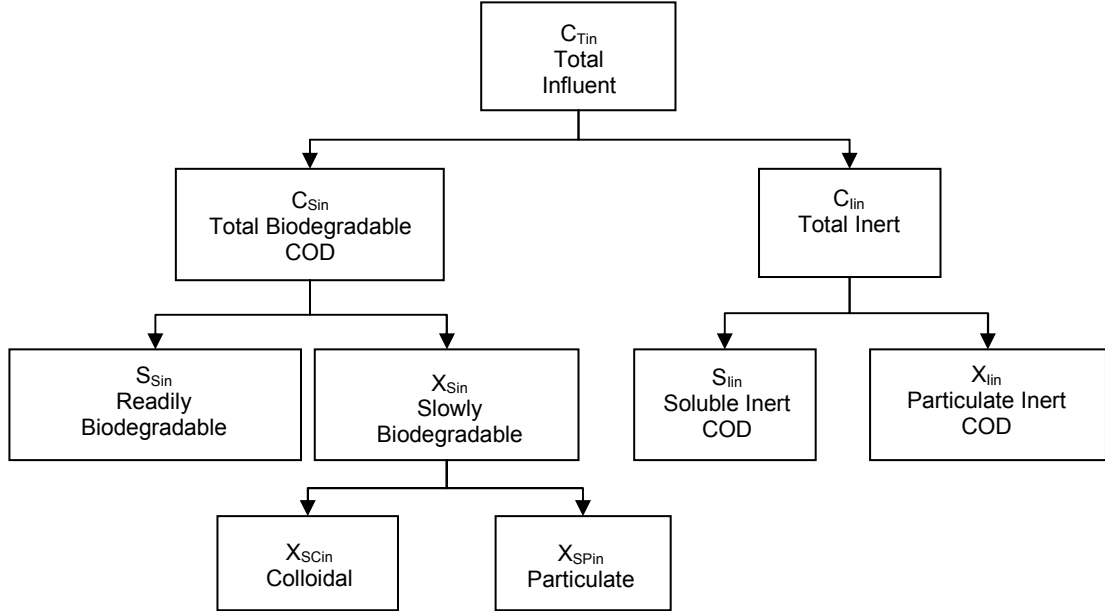
Figure 4.1: Categorization of COD components in raw sewage
