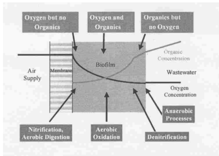
Figure 2.25: Different environments in a membrane aerated biofilm (Semmens and Shanahan,2005)
