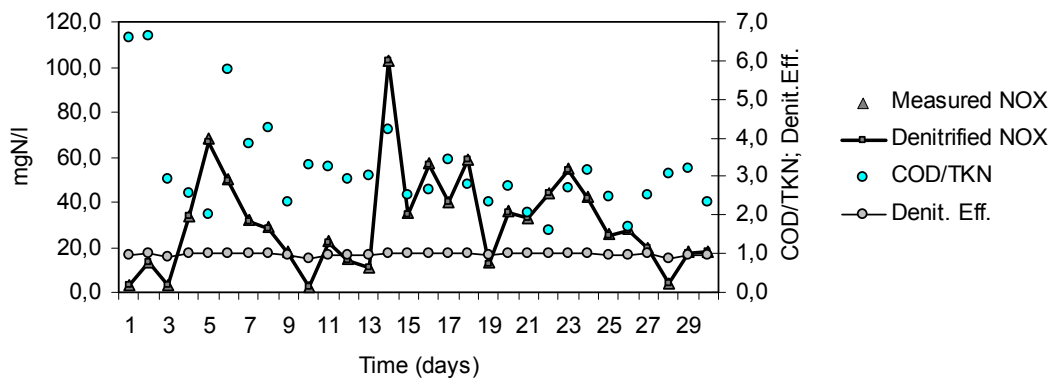
Figure 5.34: Oxidized S_{NH} and denitrified S_{NO}
