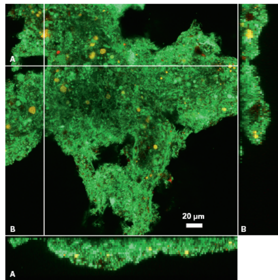
Figure 2.24: Confocal laser scanning microscopic sections through an activated sludge floc, stained with gene probes. Green: general probe for all bacteria; Yellow: specific probe for a group of ammonia-oxidizing bacteria.
