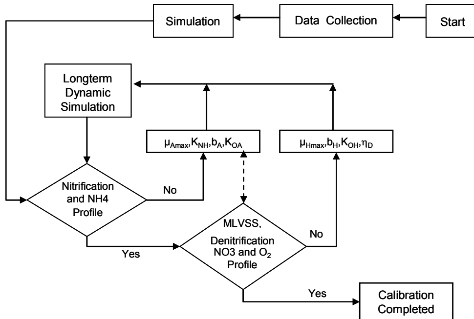
Figure 4.12: Calibration methodology of the new adopted process matrix for MBR (Insel et al., 2006)
