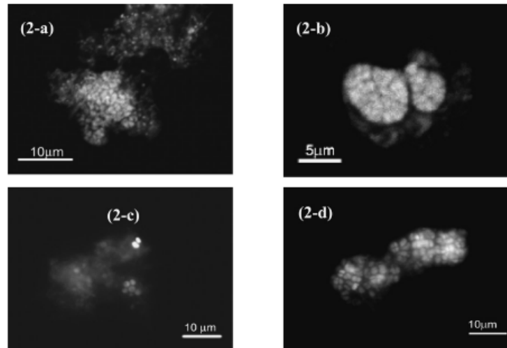
Figure 2.21: Clusters of Nitrosospira spp. (2-a), clusters of Nitrosospira spp. (2-b), genus Paracoccus cells (2-c, 2-d), (Sofia et al., 2004)
