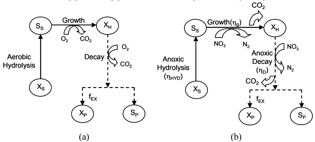
Figure 4.4: Schematic illustration of death-regeneration model (basis of ASM1) under (a) aerobic (b) anoxic conditions (Henze et al., 1987)
