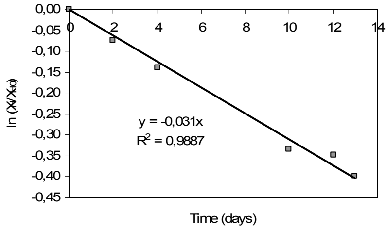
Figure A1: Change of active biomass with respect to time
