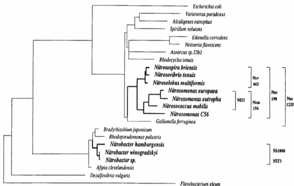
Figure 3.7: Phylogenetic tree inferred from comparison of 16S rRNA sequences. (Target organisms for probes Nso190, Nso1225, Nsm156, Nsv443, NEU, NIT3, and Nb1000) (Mobarry et al., 1996)
