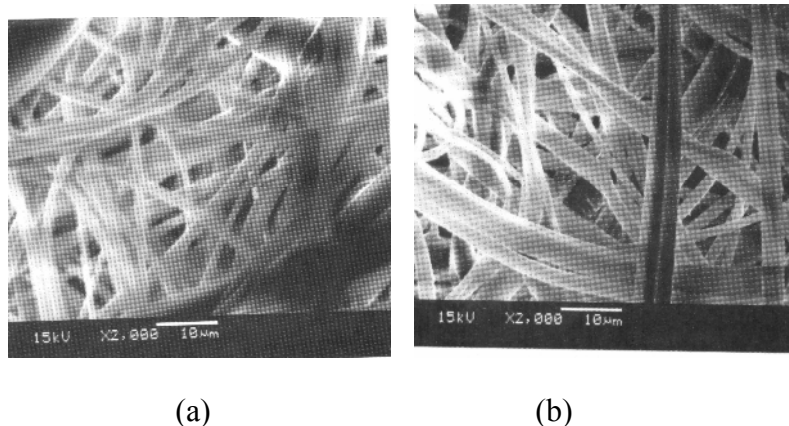
Figure 2.6: (a) 3 \mu\text{m} non-woven membrane surface (b) 5 \mu\text{m} non-woven membrane surface
