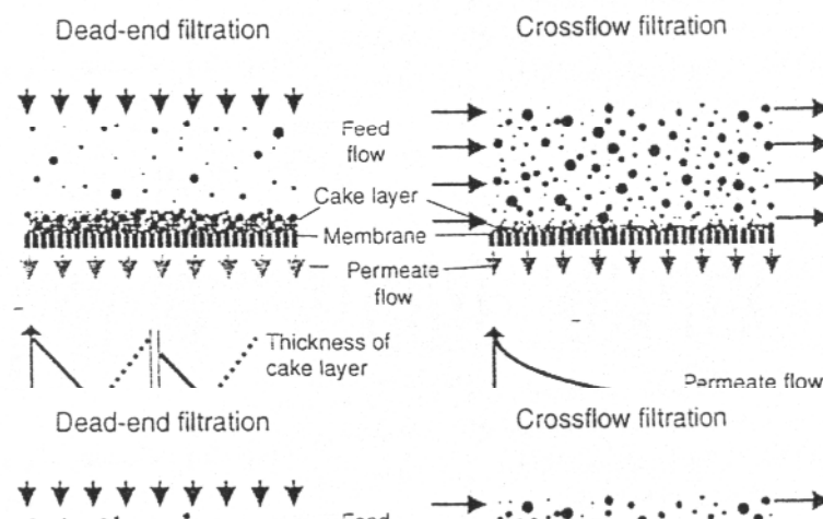
Figure 2.10: Schematic presentation of dead-end and crossflow filtration
