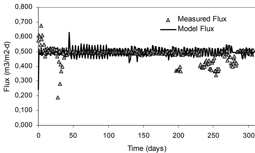
Figure 5.38: Longterm simulated vs measured flux values
