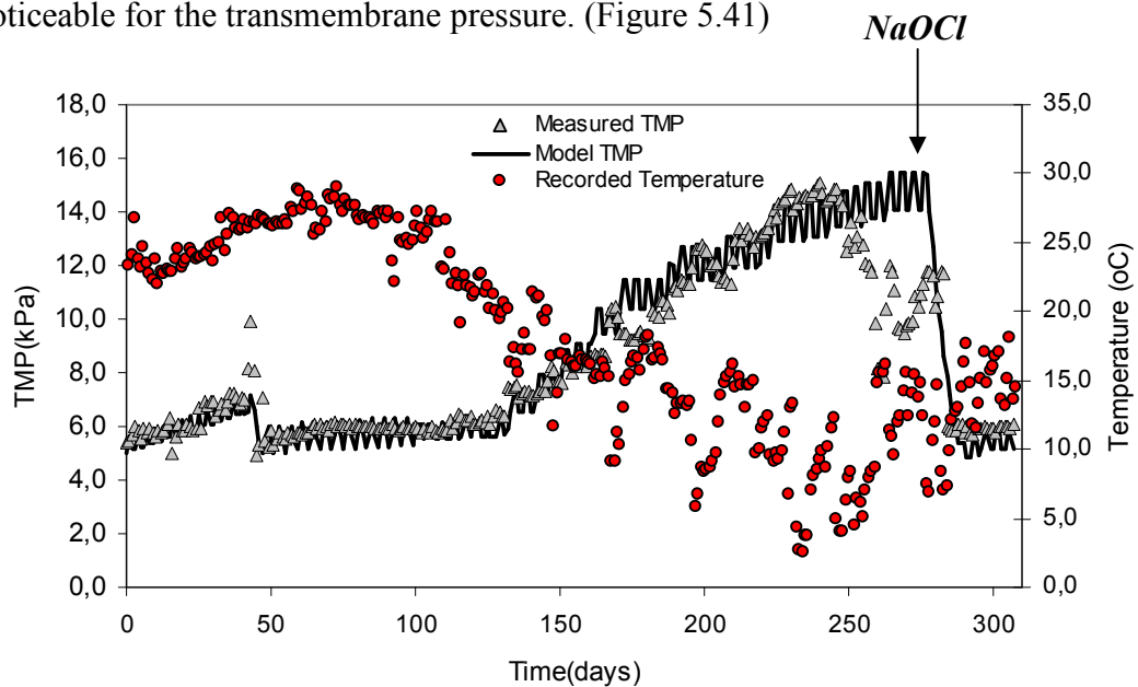
Figure 5.41: Longterm simulated vs measured TMP results with the effect of temperature
