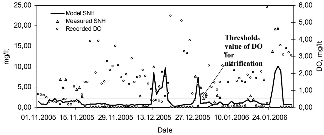
Figure 5.13: Nitrification performance of the pilot membrane bioreactor with respect to dissolved oxygen
