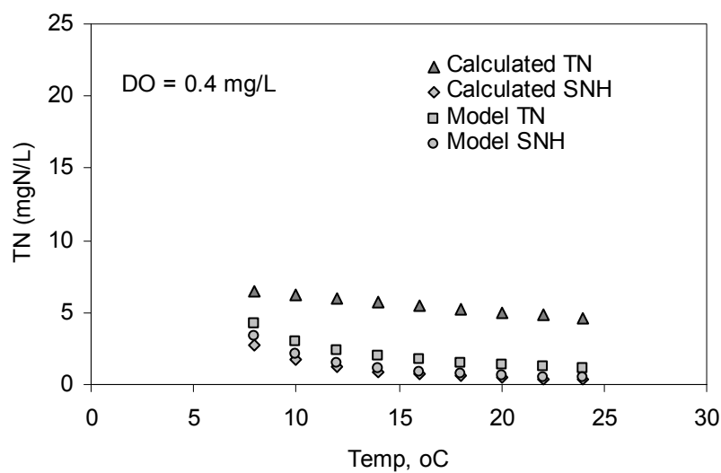
Figure 5.20: Comparison of total effluent nitrogen level with respect to stoichiometric and model results for varying temperature
