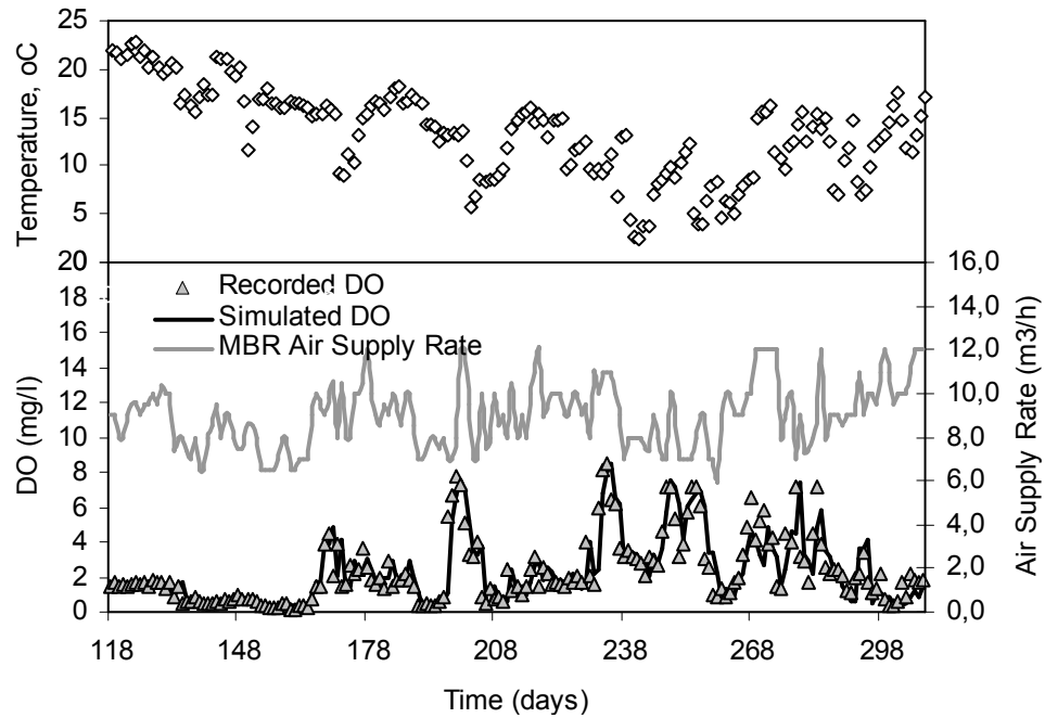
Figure 5.12: Airflowrate vs. measured and simulated DO in MBR unit
