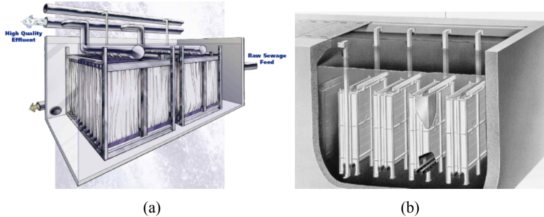
Figure 2.9: (a) Zenon and (b) Kubota membrane modules
