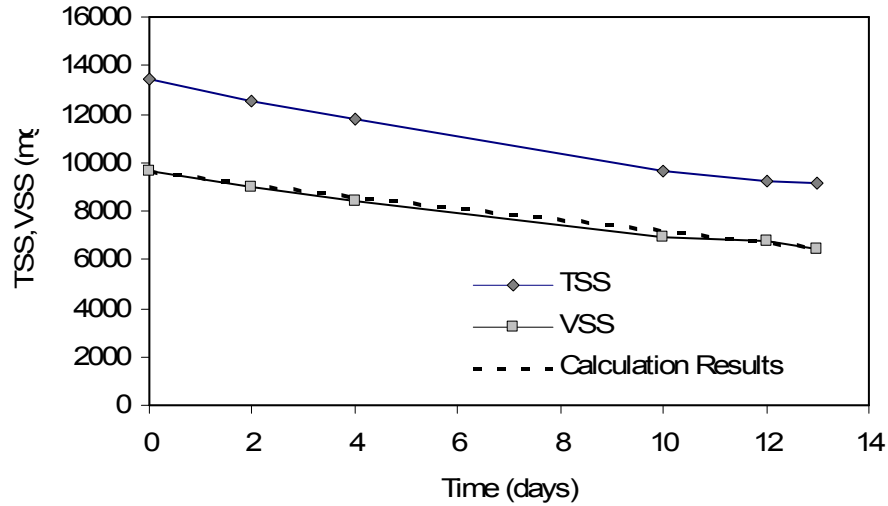
Figure A2: Comparison of the experimental results with the calculation results
