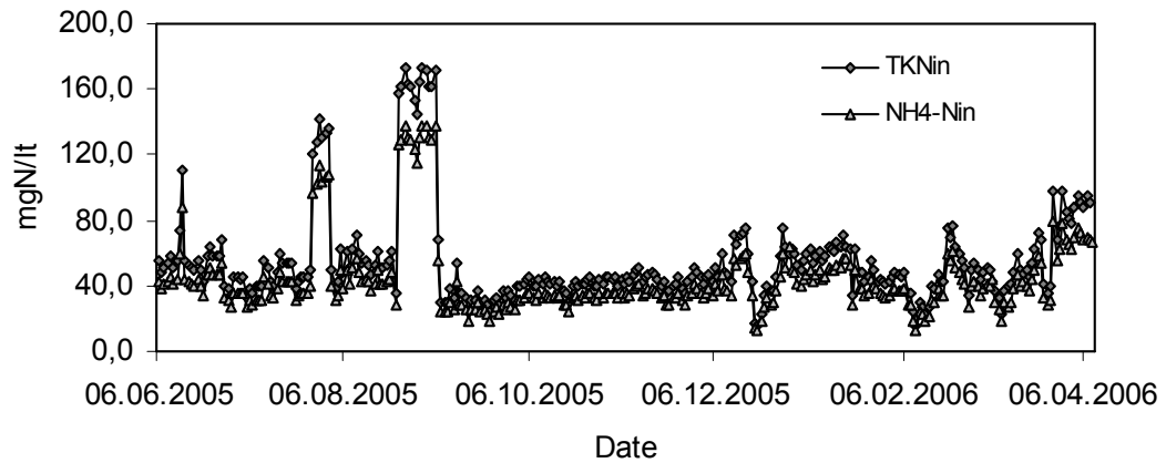
Figure 5.3: Influent TKN and ammonia nitrogen profiles
