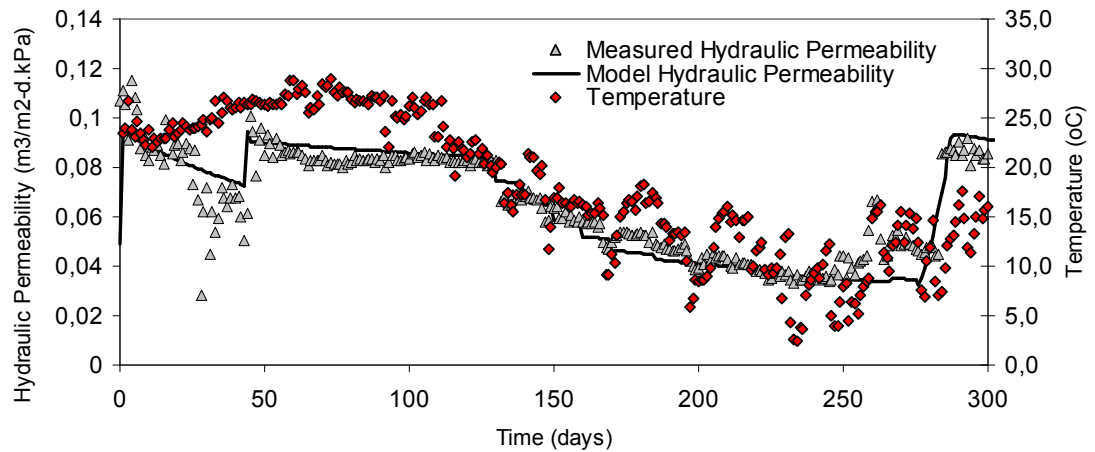
Figure 5.40: Temperature effect on the hydraulic permeability
