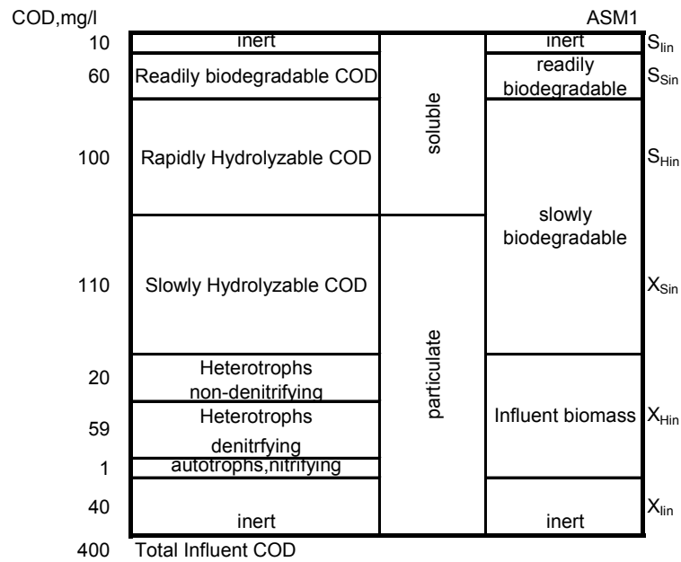
Figure 4.2: Quantified COD components in raw sewage , C_{Tin}=400\text{mg/l}
