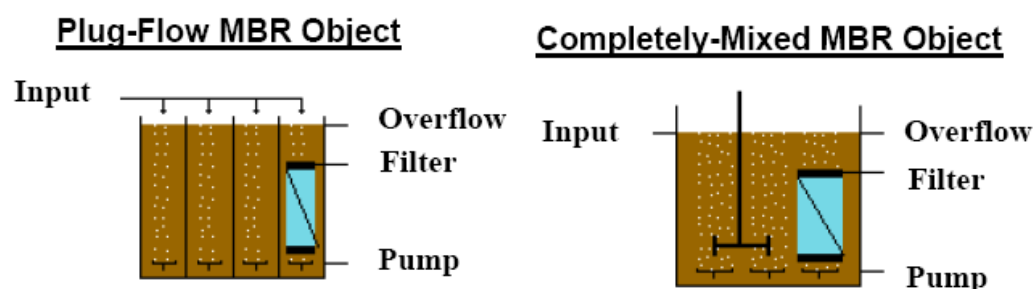
Figure 4.14: GPS-X membrane bioreactor objects
