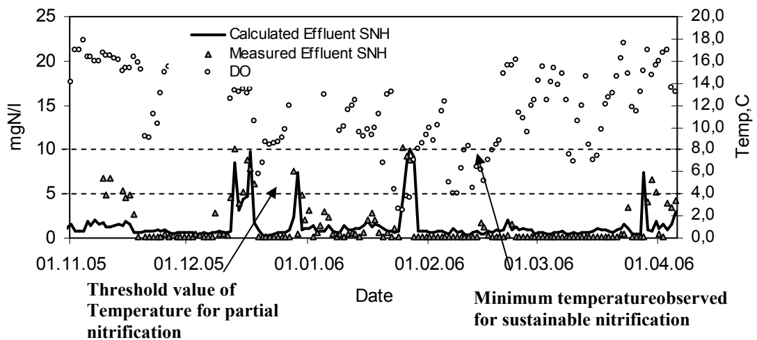
Figure 5.14: Nitrification performance of the pilot membrane bioreactor with respect to temperature
