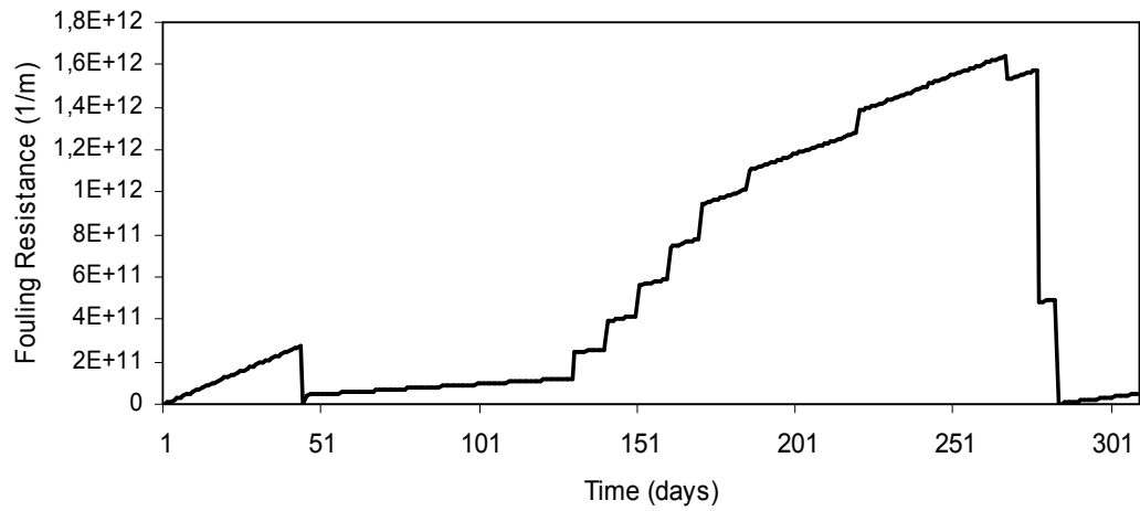
Figure 5.44: Foulant resistance of the membrane bioreactor
