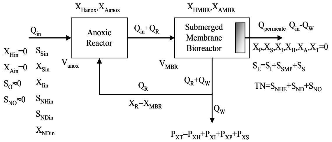
Figure 4.8: Schematic process diagram for carbon and nitrogen removal in submerged membrane bioreactor
