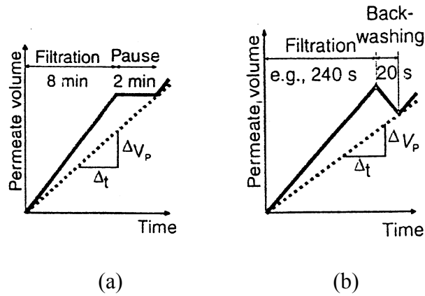
Figure 2.19: Relationship between the permeate volume and time (a) flat sheet membranes, (b) hollow fiber membranes (operational sequence) (Günder, 2001)
