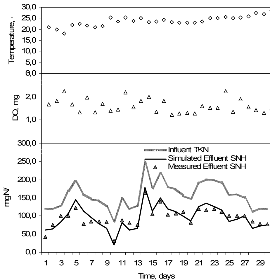
Figure 5.31: Ammonia nitrogen profile with respect to dissolved oxygen and temperature
