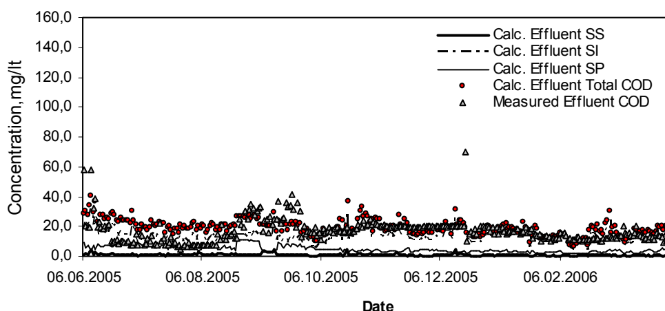
Figure 5.10: Simulated effluent COD fractions
