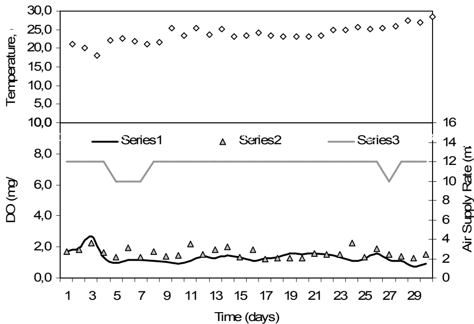
Figure 5.29: Oxygen modelling results
