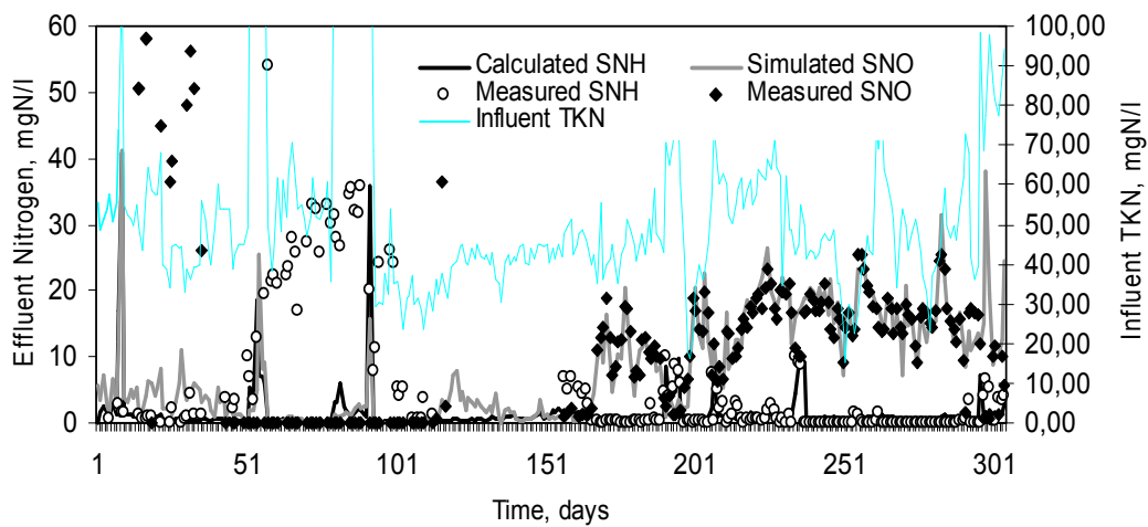
Figure 5.18: Simulated and calculated effluent ammonia ( S_{NH} ) and nitrate ( S_{NO} ) concentrations
