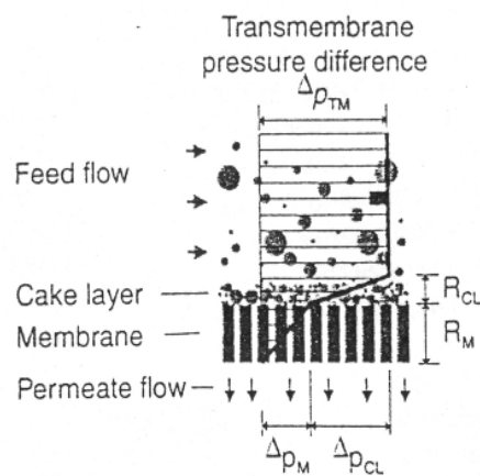
Figure 2.12: Schematic illustration of pressure distribution across the membrane and the cake layer
