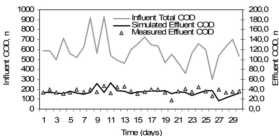
Figure 5.28: Influent, effluent COD and removal efficiencies
