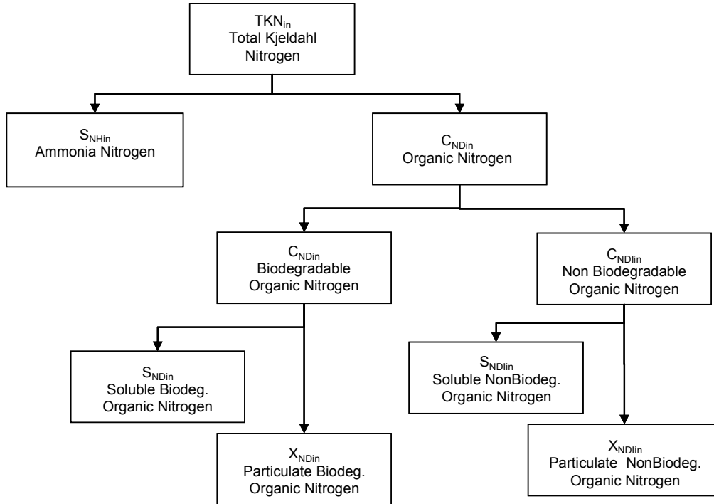
Figure 4.3: Influent wastewater characterization for nitrogenous material
