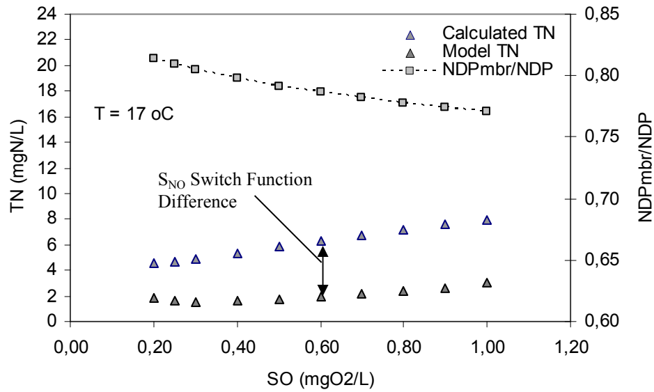
Figure 5.19: Comparison of total effluent nitrogen level with respect to stoichiometric and model results for varying dissolved oxygen
