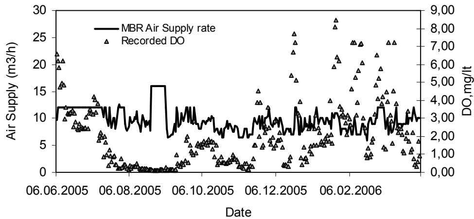
Figure 5.11: MBR air supply rate vs recorded DO
