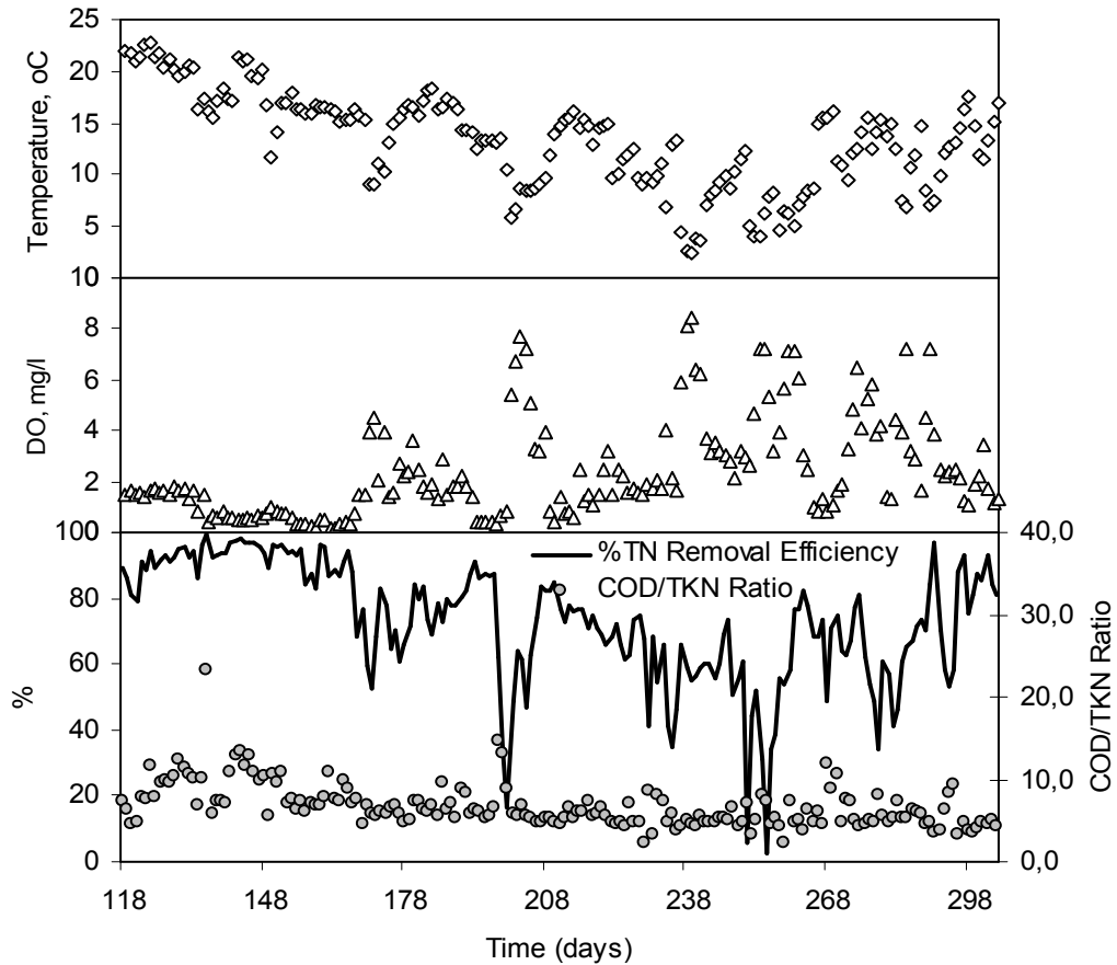
Figure 5.17: Total nitrogen removal efficiency vs. DO and influent COD/TKN ratio
