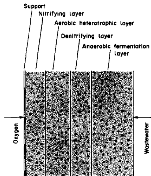
Figure 2.18: Structure of support aerated biofilm in a membrane bioreactor (Timberlake et al.,1988)
