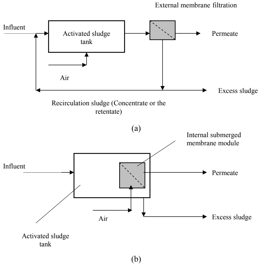
Figure 2.16: Schematic representation of MBR with (a) external membrane filtration, (b) internal submerged membrane filtration
