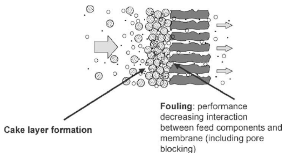
Figure 5.36: Phenomena limiting flux performance in membrane filtration (Wintgens et al., 2003)
