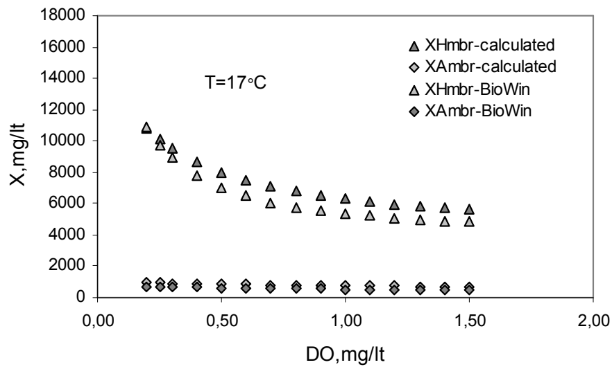
Figure 5.7: Variation of active biomass concentration with respect to changing dissolved oxygen concentration
