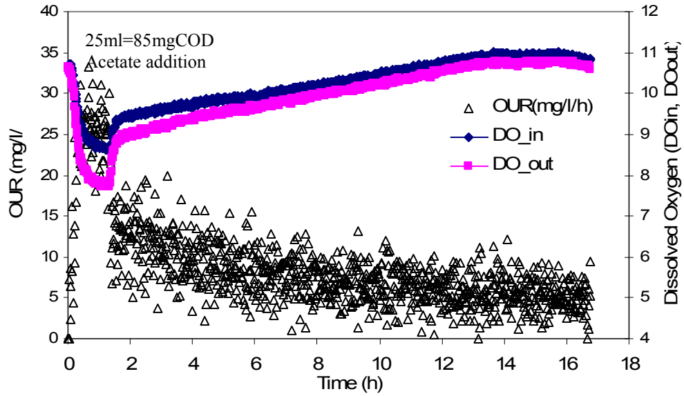
Figure A3: Results of the respirometric analysis
