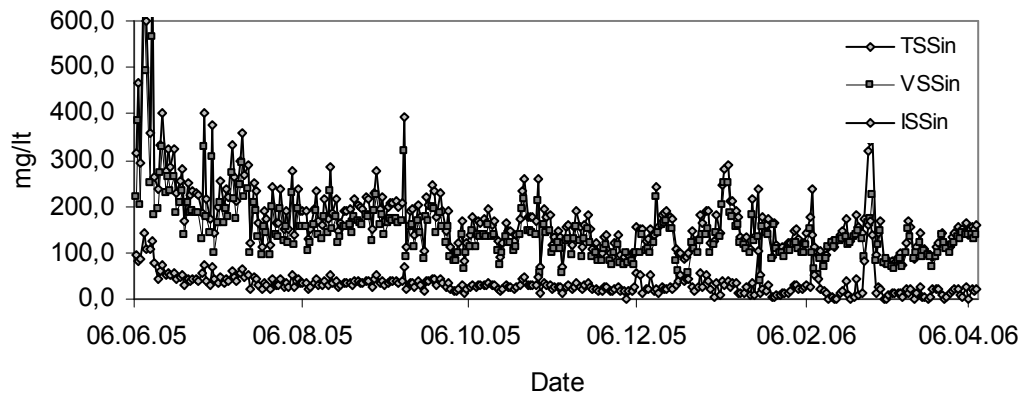
Figure 5.4: Influent TSS,VSS and ISS profiles
