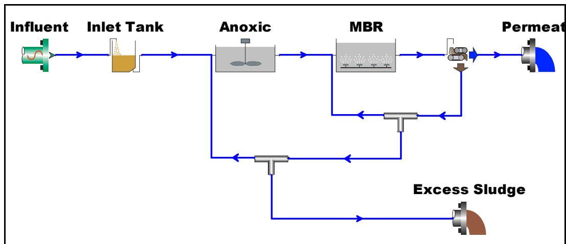
Figure 4.10: Plant layout implemented in BioWin 2.2® software
