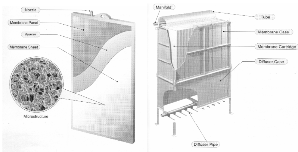
Figure 2.5: Flat sheet membrane structure and a single module
