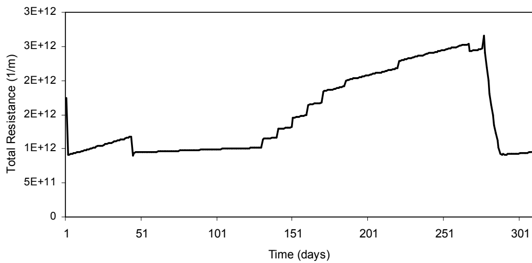
Figure 5.45: Total membrane resistance of the membrane bioreactor
