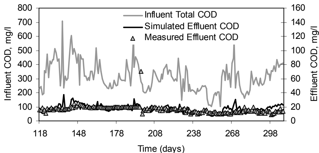
Figure 5.9: Influent COD and simulated/calculated effluent COD concentration profiles
