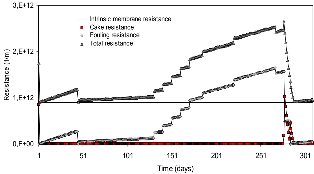
Figure 5.46: Superposed resistance parameters
