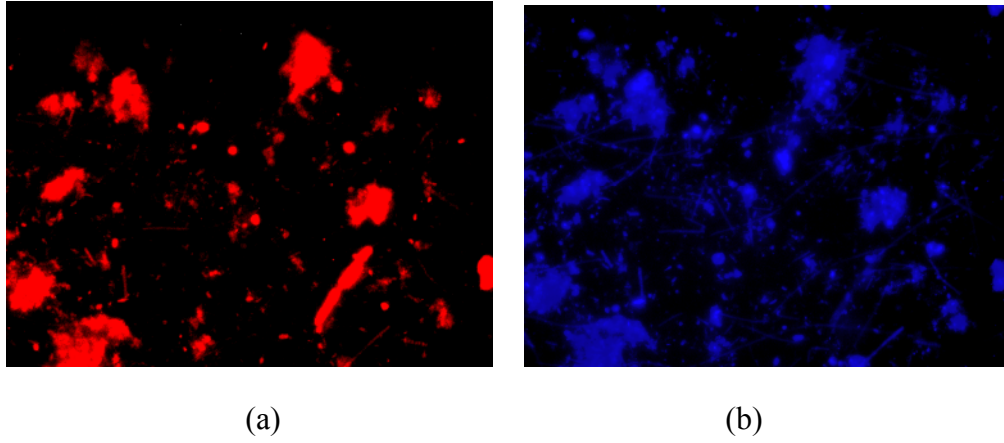
Figure 5.51: Cells detected with NB1000 probe (a) Hybridized cells (b) DAPI-stained cells (Pala, 2006)
