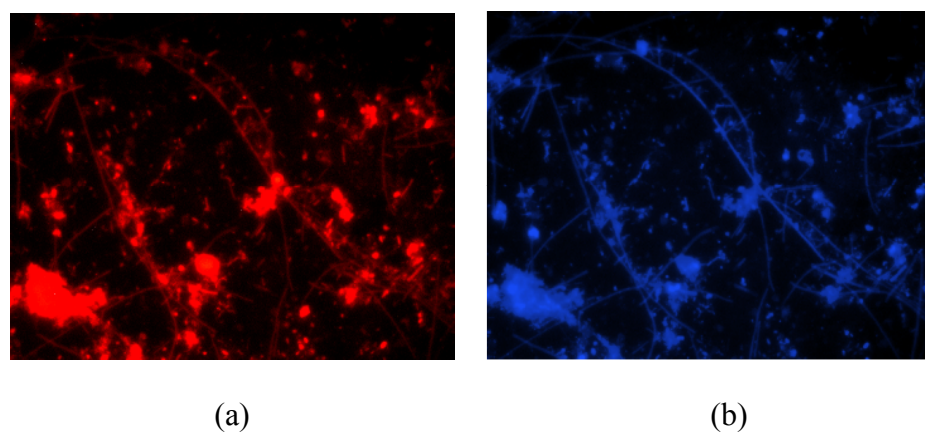
Figure 5.50: Cells detected with ALF968 probe (a) Hybridized cells (b) DAPI-stained cells (Pala, 2006)
