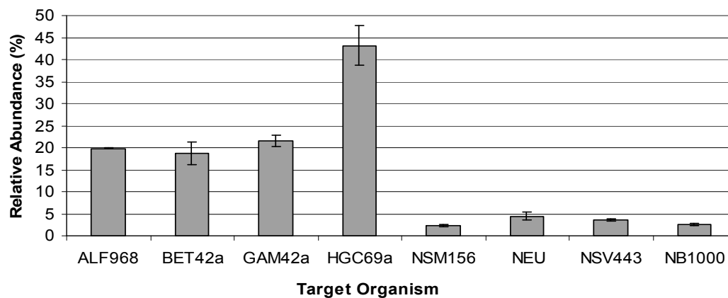
Figure 5.48: Relative abundance of the microbial population (Pala, 2006)
