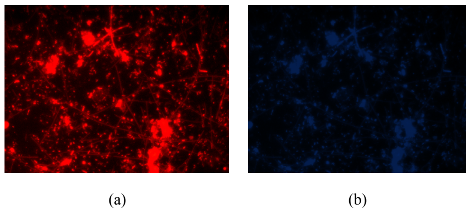
Figure 5.49: Cells detected with EUBMIX probe (a) Hybridized cells (b) DAPI-stained cells (Pala, 2006)
