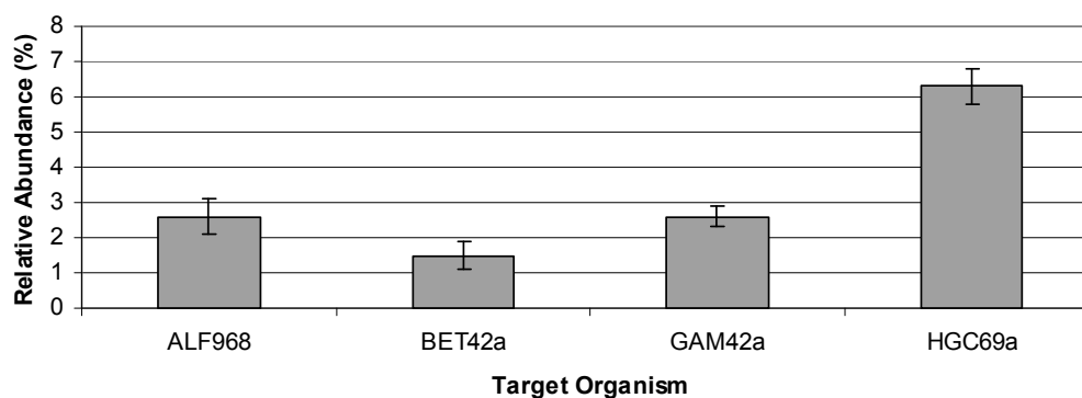
Figure 5.47: Relative abundance of filamentous morphotypes (Pala, 2006)
