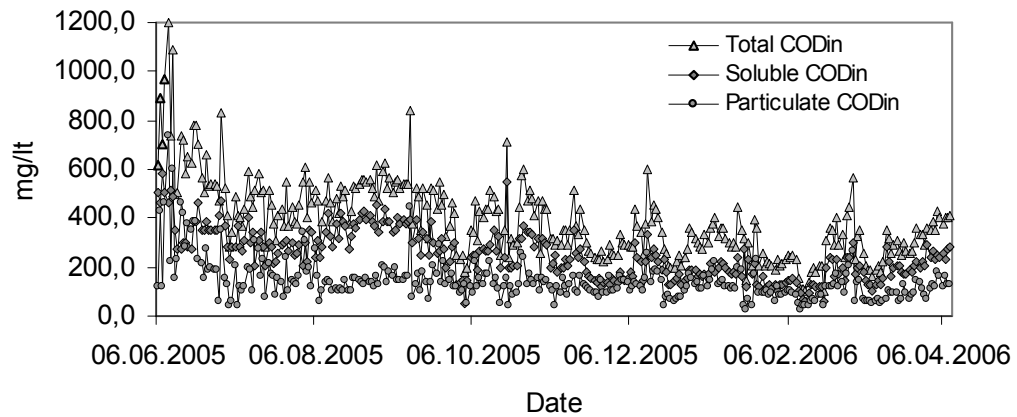
Figure 5.2: Influent total, particulate and soluble COD
