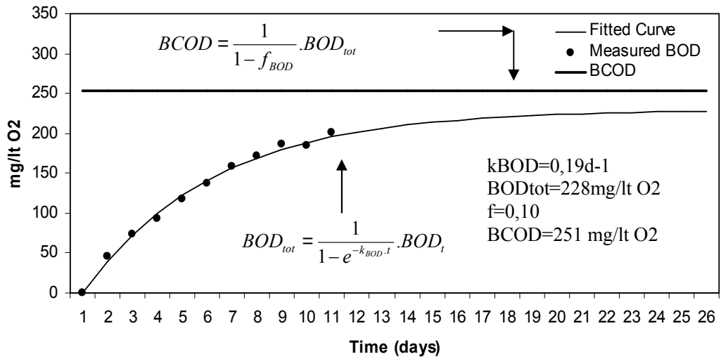
Figure 5.1: Fitted BOD curve for the set of measured BOD 5 data points
