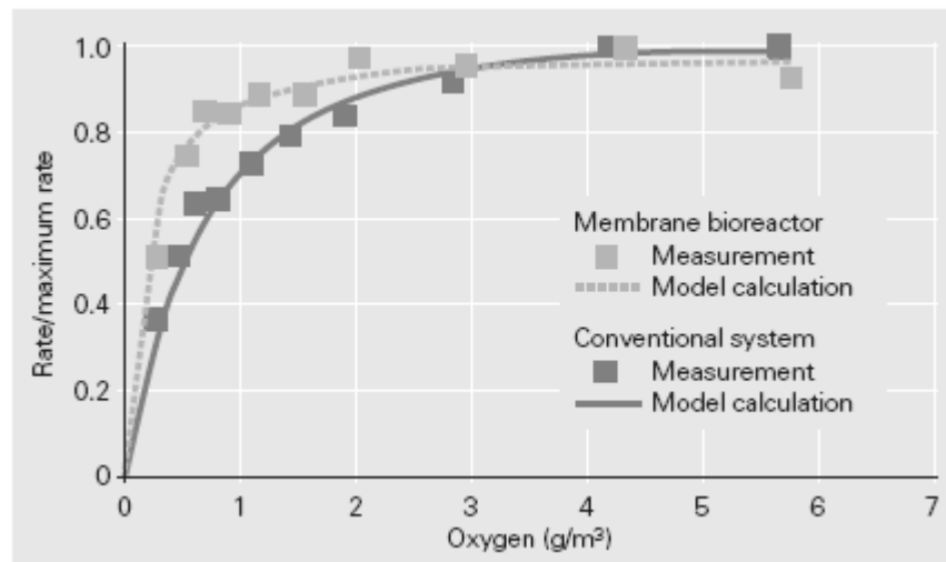
Figure 5.25: Measured and calculated nitrification rates as a function of oxygen concentration under excess substrate conditions (Manser et al., 2005)
