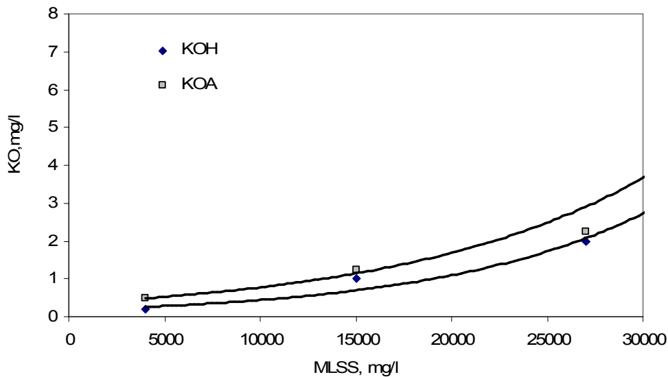
Figure 5.24: Variation of K_{OA} and K_{OH} with respect to MLSS
