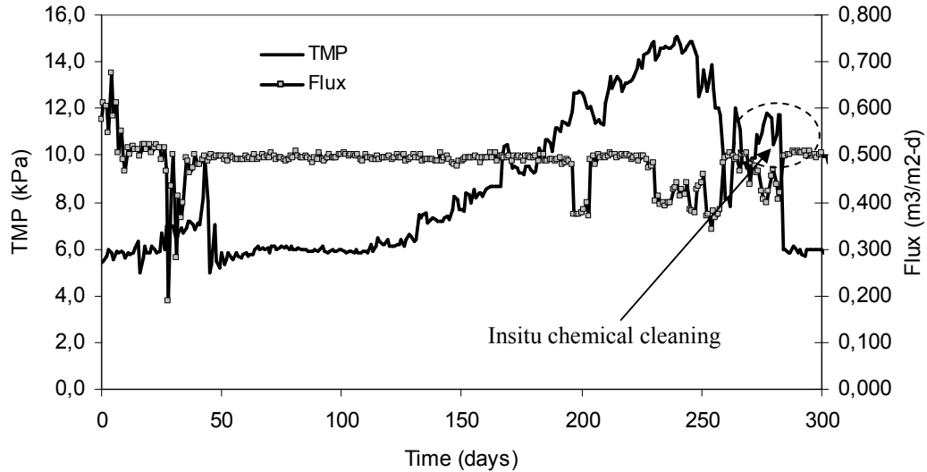
Figure 5.37: Variation of longterm TMP and flux values
