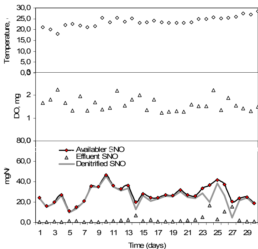
Figure 5.33: N_{OX} vs S_{NO} with respect to dissolved oxygen and COD/TKN ratio
