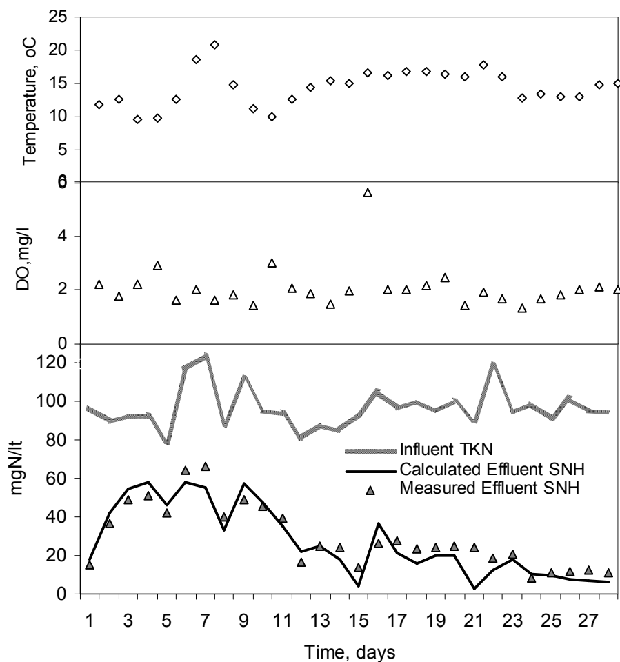
Figure 5.21: Ammonia ( S_{NH} ) profile for Run II
