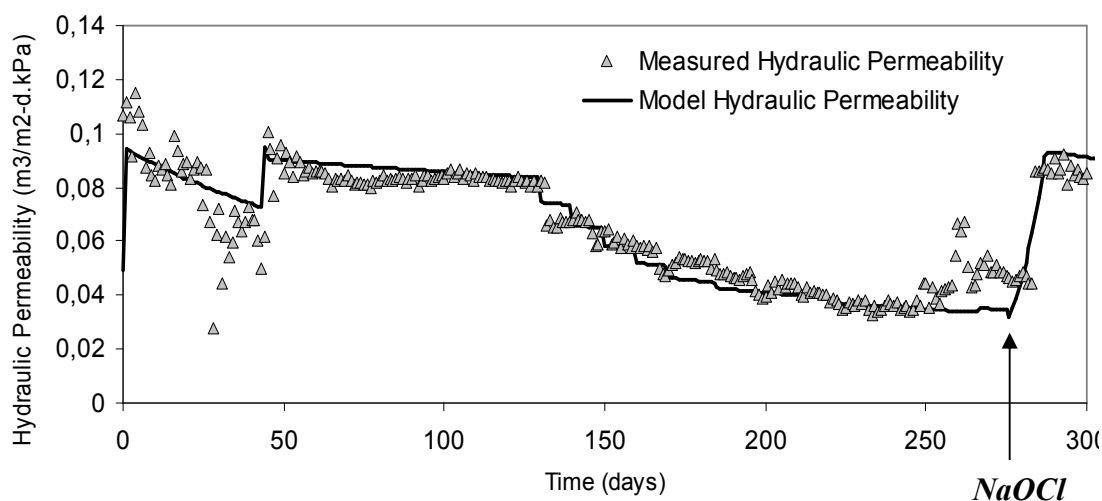
Figure 5.39: Longterm simulated vs measured hydraulic permeability values
