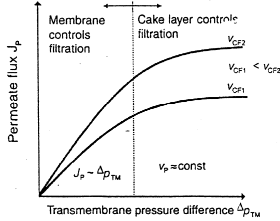
Figure 2.13: Relationship between transmembrane pressure and permeate flux in crossflow microfiltration
