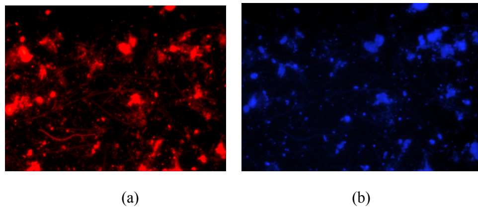
Figure 5.53: Cells detected with GAM42a probe (a) Hybridized cells (b) DAPI-stained cells (Pala, 2006)
