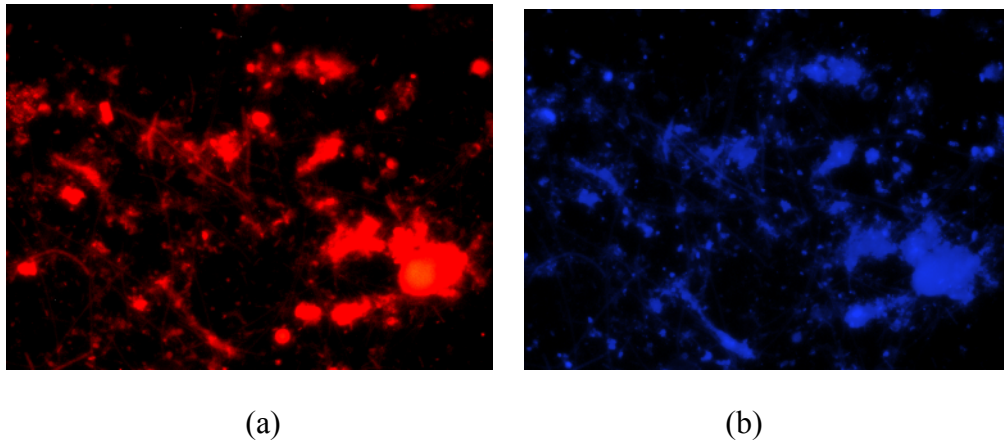
Figure 5.52: Cells detected with BET42a probe (a) Hybridized cells (b) DAPI-stained cells (Pala, 2006)
