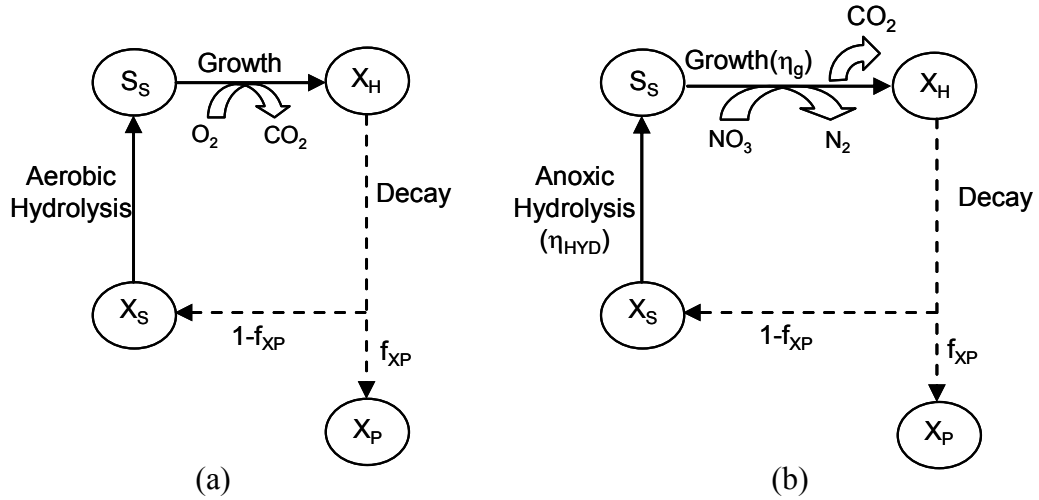
Figure 4.4: Schematic illustration of death-regeneration model (basis of ASM1) under (a) aerobic (b) anoxic conditions (Henze et al., 1987)
