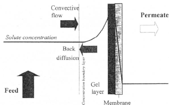
Figure 2.14: Schematic representation of concentration polarization
