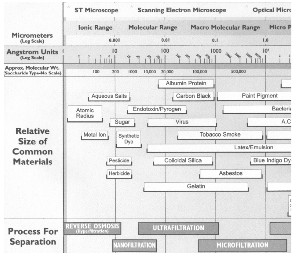
Figure 2.2: The filtration spectrum for different membrane separation processes
