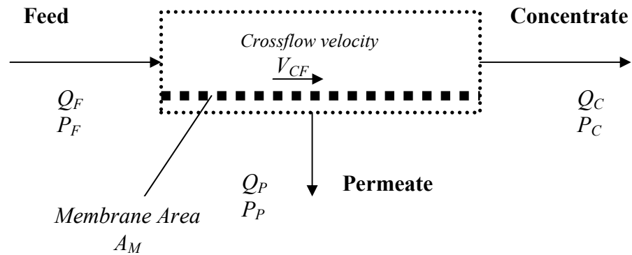
Figure 2.11: Definition of operational parameters in crossflow filtration
