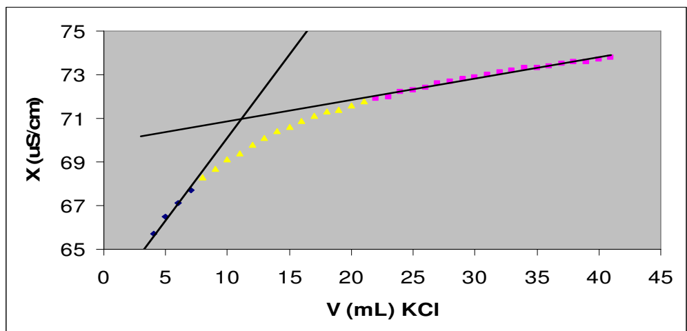
Figure A.80 : Titration of 0.102mg/mL PSP with KCl ( I=1 \times 10^{-2} \text{ mol/L} )
