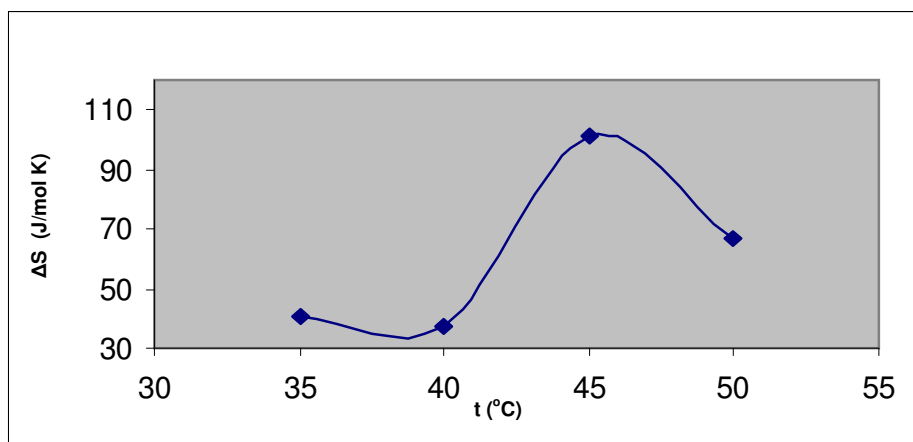
Figure D.48 : \Delta S = f(t^{\circ}\text{C}) Curve of 1 \times 10^{-4}(\text{mol/L}) PAH- 1 \times 10^{-4}(\text{mol/L}) \text{Na}_2\text{SO}_4 , ( I = 1 \times 10^{-3} \text{ mol/L} )
