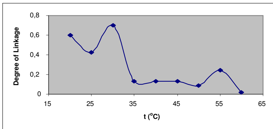
Figure D.32 : Degree of linkage, \theta = f(t\text{ }^{\circ}\text{C}) Curve of 1 \times 10^{-2}(\text{mol/L}) PAH- 1 \times 10^{-2}(\text{mol/L}) \text{Na}_2\text{SO}_4 ( I = 1 \times 10^{-1} \text{ mol/L} )
