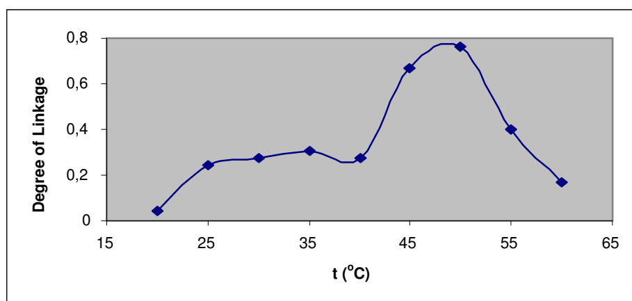
Figure D.20 :Degree of linkage, \theta = f (t °C) Curve of 1 \times 10^{-4} (mol/L) PAH- 1 \times 10^{-4} (mol/L) NaCl , (I= 1 \times 10^{-3} mol/L)
