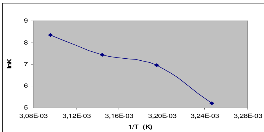
Figure D.105 : Curve of equilibrium constant 1 \times 10^{-4} \text{ (mol/L) PAH- } 1 \times 10^{-4} \text{ (mol/L) CaCl}_2 , (I = 1 \times 10^{-3} \text{ mol/L})
