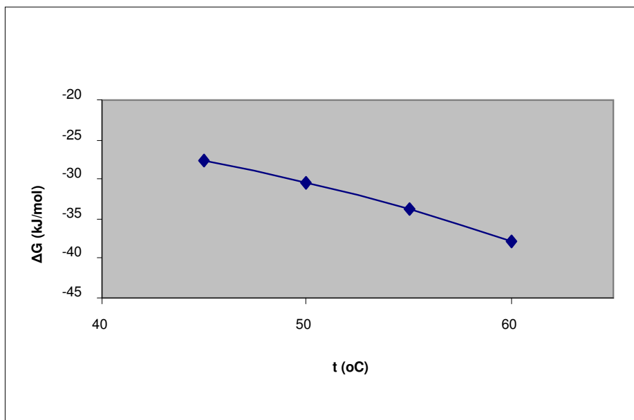
Figure 3. 16: \Delta G = f(t^{\circ}\text{C}) Curve of 1 \times 10^{-4} \text{ (mol/L)} PSP - 1 \times 10^{-4} \text{ (mol/L)} NaCl
