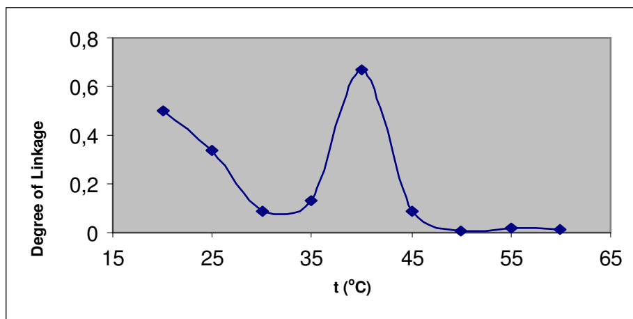
Figure D.86 : Degree of linkage, \theta = f(t(^{\circ}\text{C})) Curve of 1 \times 10^{-1}(\text{mol/L}) PAH- 1 \times 10^{-1}(\text{mol/L}) \text{CaCl}_2 ( I=1 \text{ mol/L} )
