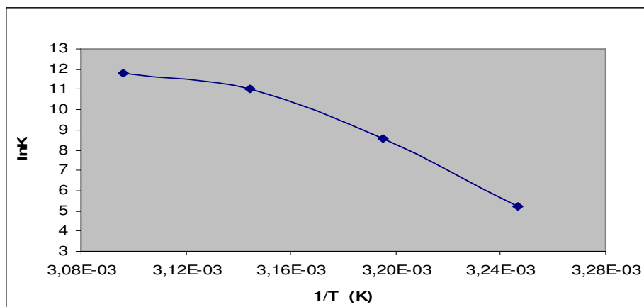
Figure D.21 :Curve of equilibrium constant 1 \times 10^{-4} (mol/L) PAH- 1 \times 10^{-4} (mol/L) NaCl , (I= 1 \times 10^{-3} mol/L)
