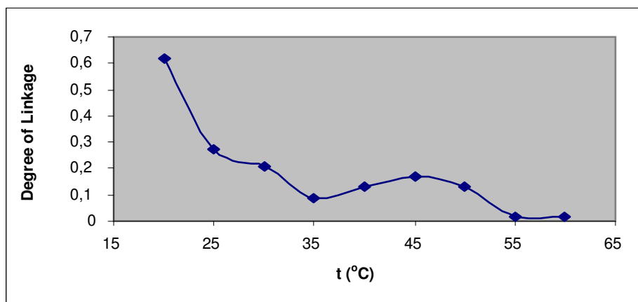
Figure D.26 : Degree of linkage, \theta = f(t\text{ }^{\circ}\text{C}) Curve of 1 \times 10^{-1}(\text{mol/L}) PAH- 1 \times 10^{-1}(\text{mol/L}) \text{Na}_2\text{SO}_4 ( I=1 \text{ mol/L} )
