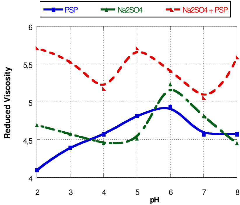
Figure 3. 10: \eta_{\text{rd}} = f(\text{pH}) Curves for 1 \times 10^{-2} mol/L \text{Na}_2\text{SO}_4 , PSP and \text{Na}_2\text{SO}_4 +PSP, ( I=1 \times 10^{-1} M)
