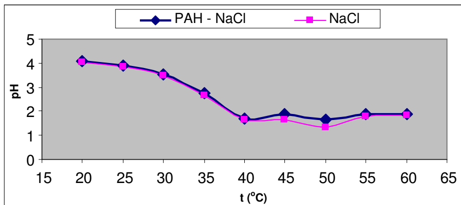
Figure D.19 :pH=f (t °C) Curve of 1 \times 10^{-4} (mol/L) PAH- 1 \times 10^{-4} (mol/L) NaCl, (I= 1 \times 10^{-3} mol/L)
