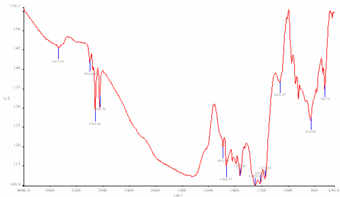
Figure 4.10. The IR spectrum of the Cationic Surfactant
