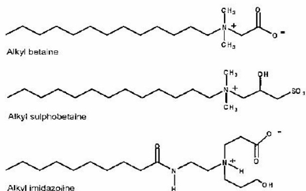
Figure 2.7. Chemical structure of some commonly used nonionic surfactants.
