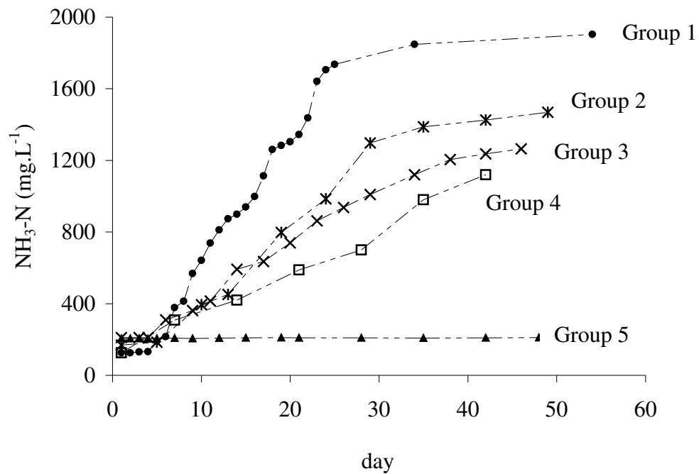
Figure 3.5: \text{NH}_3\text{-N} concentration in different urine combinations.
