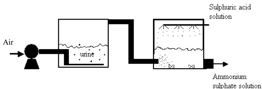
Figure 5.3: Schematic representation of the proposed system of urinary ammonium sulphate production.
