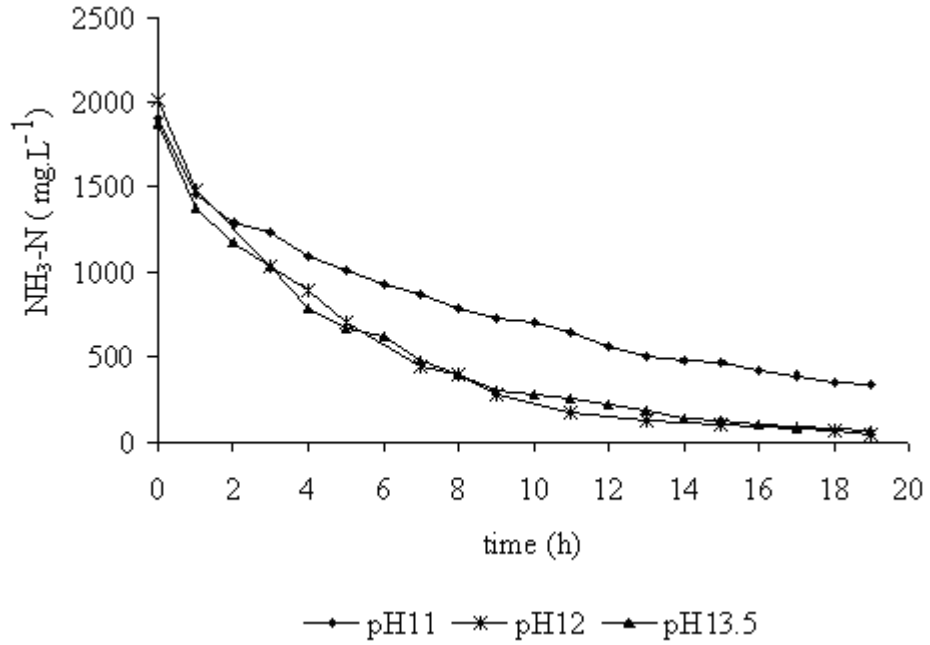
Figure 4.8: \text{NH}_3\text{-N} concentration in the stripping unit with time at constant air flow rate ( 0.12 \text{ m}^3 \cdot \text{h}^{-1} ) where the operational pH was varied as pH 11, 12 and 13.5 .
