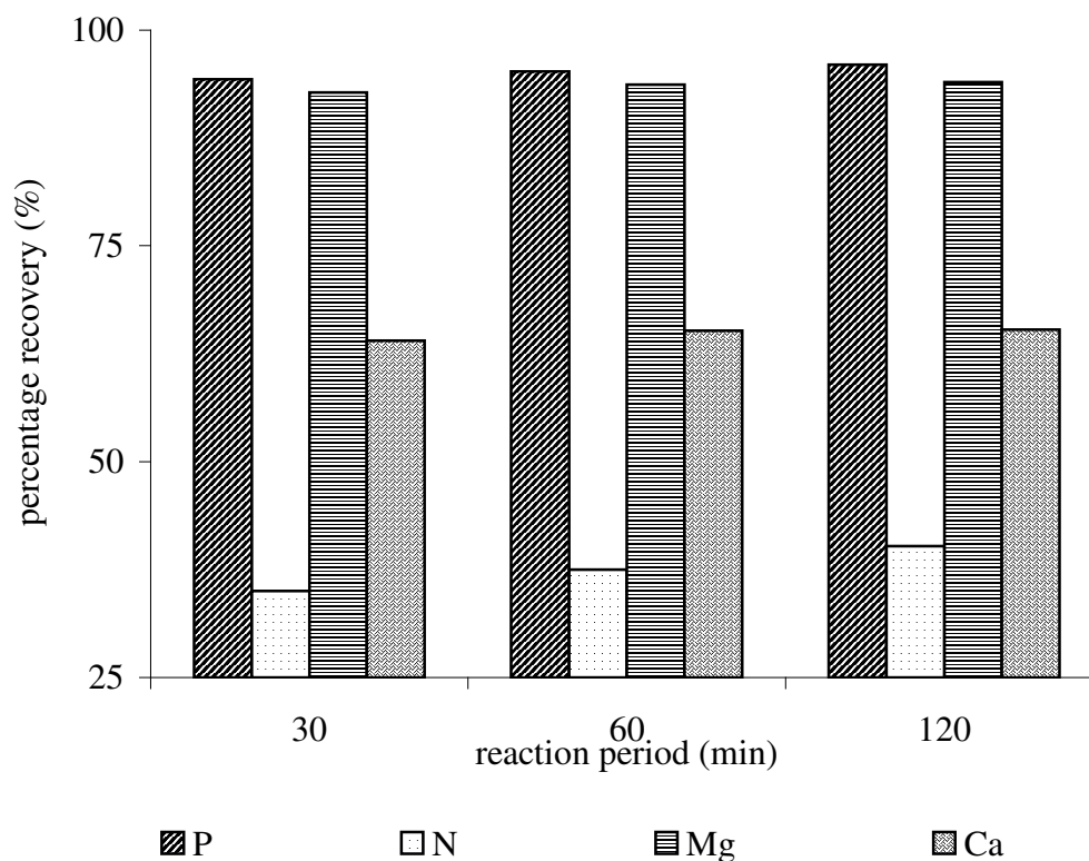
Figure 2.5: Percentage recovery of the constituent ions of struvite and urinary calcium at different reaction periods, ((Mg:P) in = 1:1, pH= 9).
