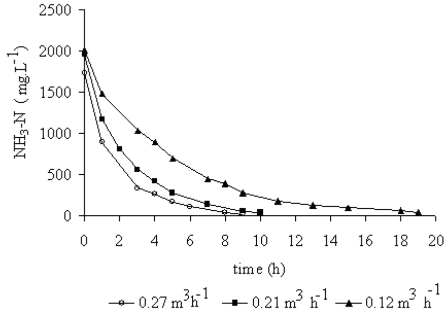
Figure 4.9: \text{NH}_3\text{-N} concentration in the stripping unit with time at constant pH (pH 12) where the air rate was varied as 0.12 , 0.21 and 0.27 \text{ m}^3 \cdot \text{h}^{-1} .
