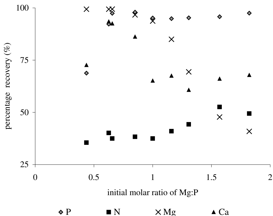
Figure 2.10: Effect of initial mole ratio of Mg:P on percentage recovery of the constituent ions of struvite and urinary calcium ( t_{\text{opt}} : 60 min, \text{pH}_{\text{opt}} :9).
