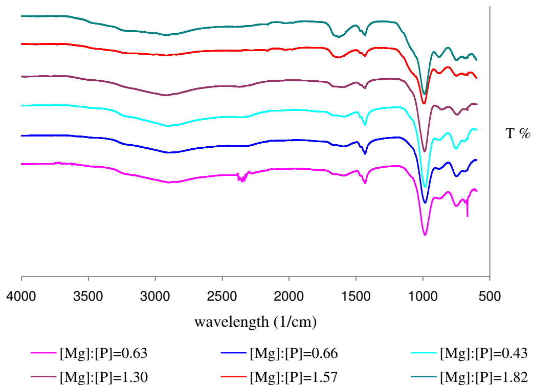
Figure 2.17: FT-IR spectra of precipitates obtained at different initial molar Mg:P ratios.
