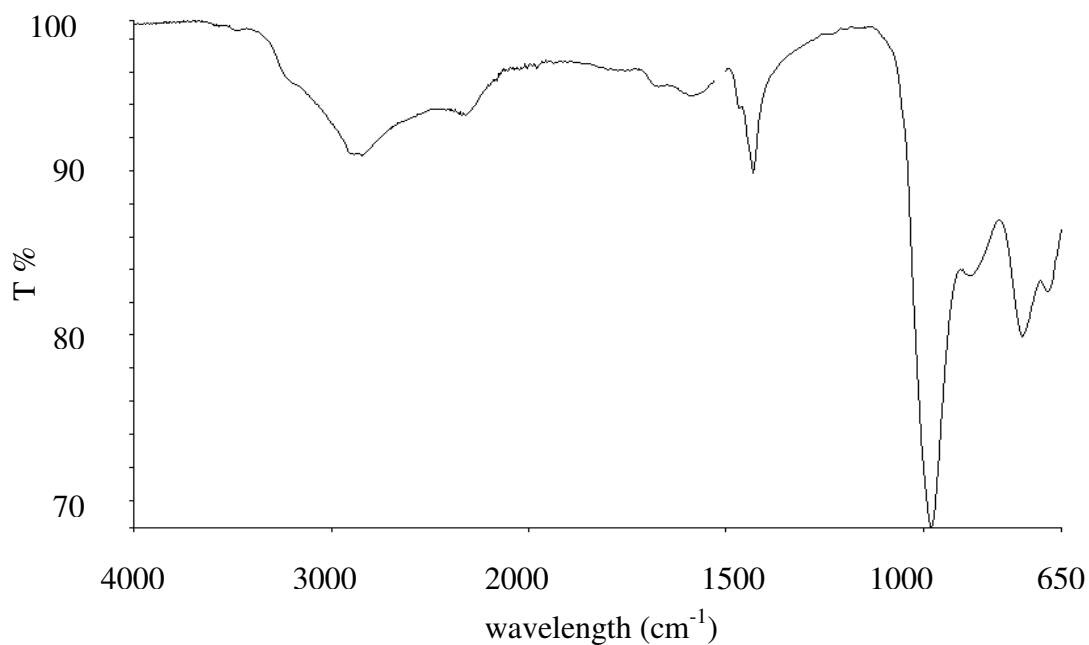
Figure 2.18: FT-IR spectra of struvite obtained from pure solution.
