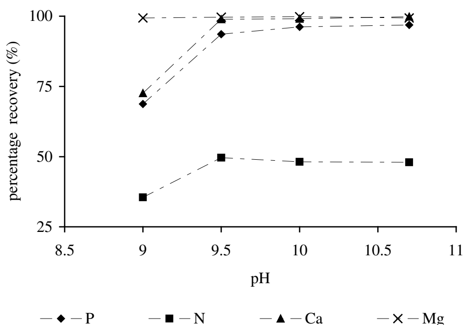
Figure 2.8: The effect of pH on percentage recovery of the constituent ions of struvite and urinary Ca. ( (\text{Mg:P})_{\text{in}} = 0.43:1 , period=60 min ).
