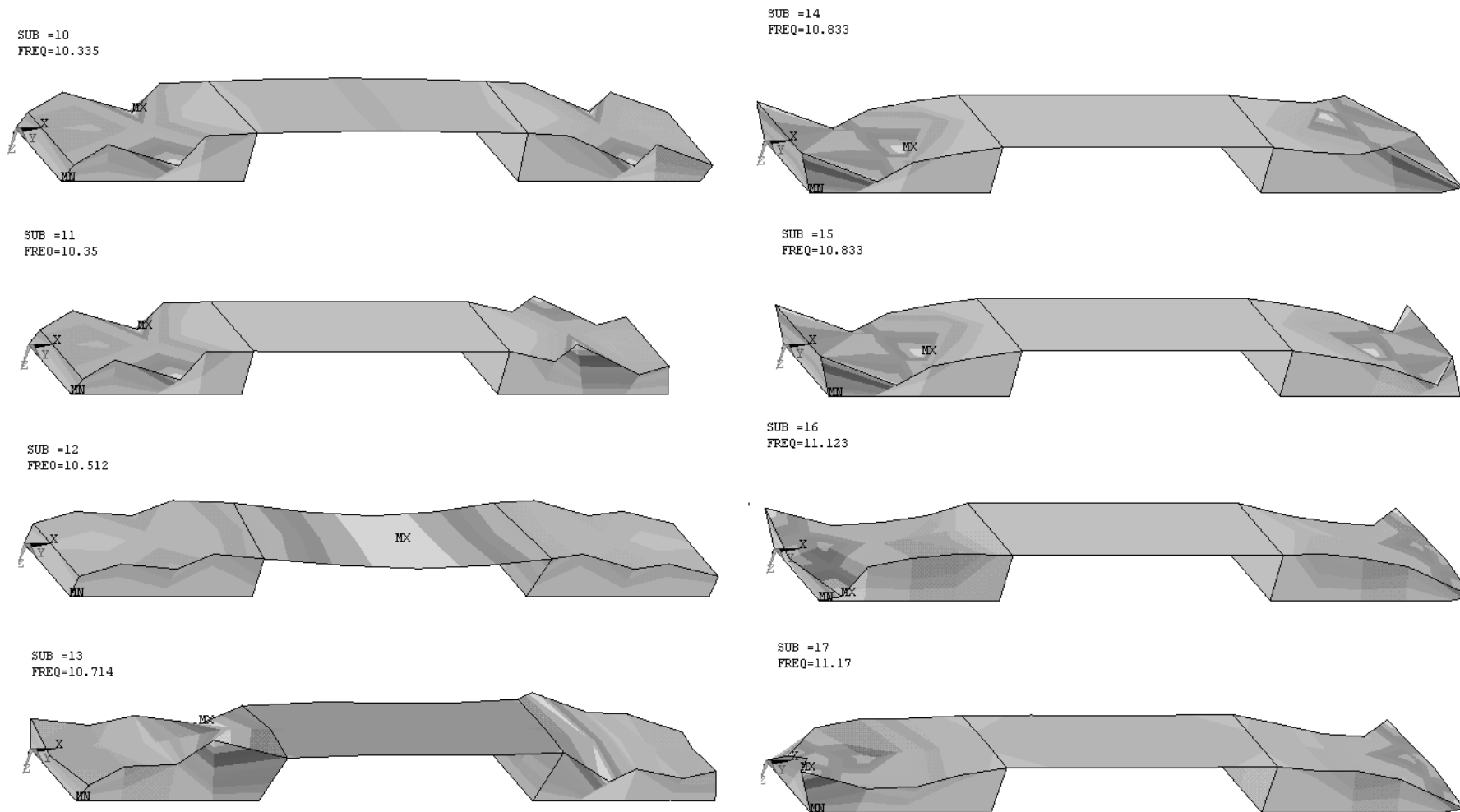
Figure A.2 : Mode shapes of the bridge (10-17).
