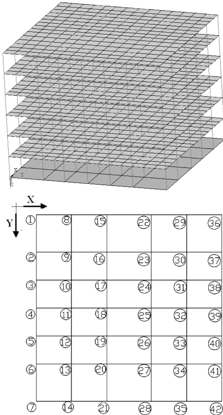
Figure 7.9 : FEM of the building and discretization of the soil-structure interface.
