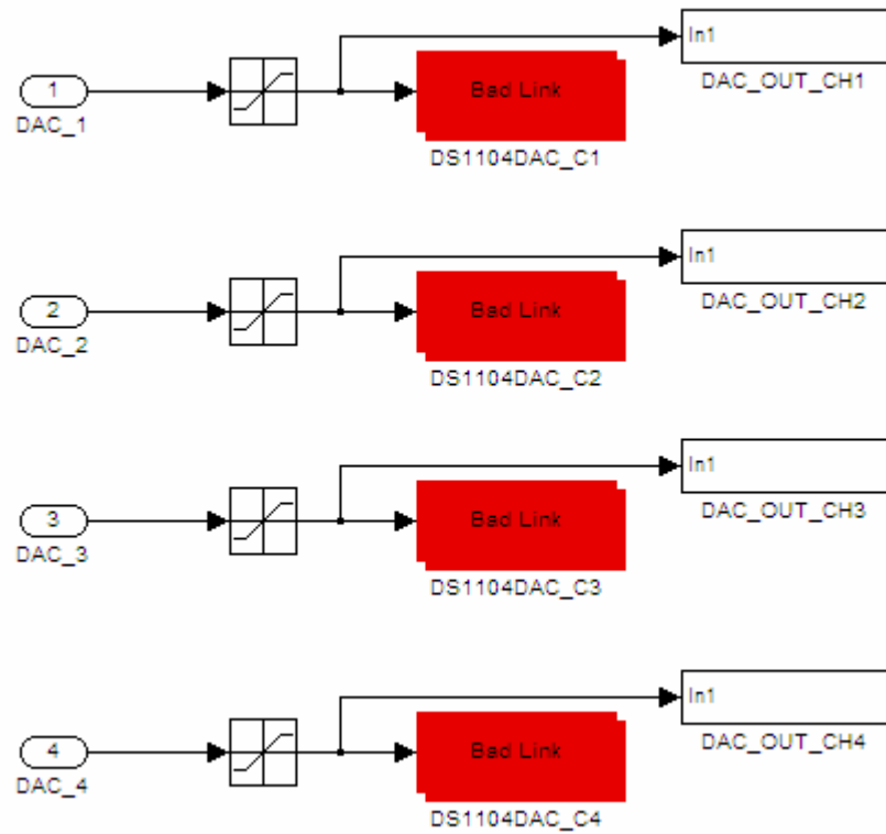
Figure 6.7: Simulink Simple Pendulum Model “DS1104 DAC” Block
