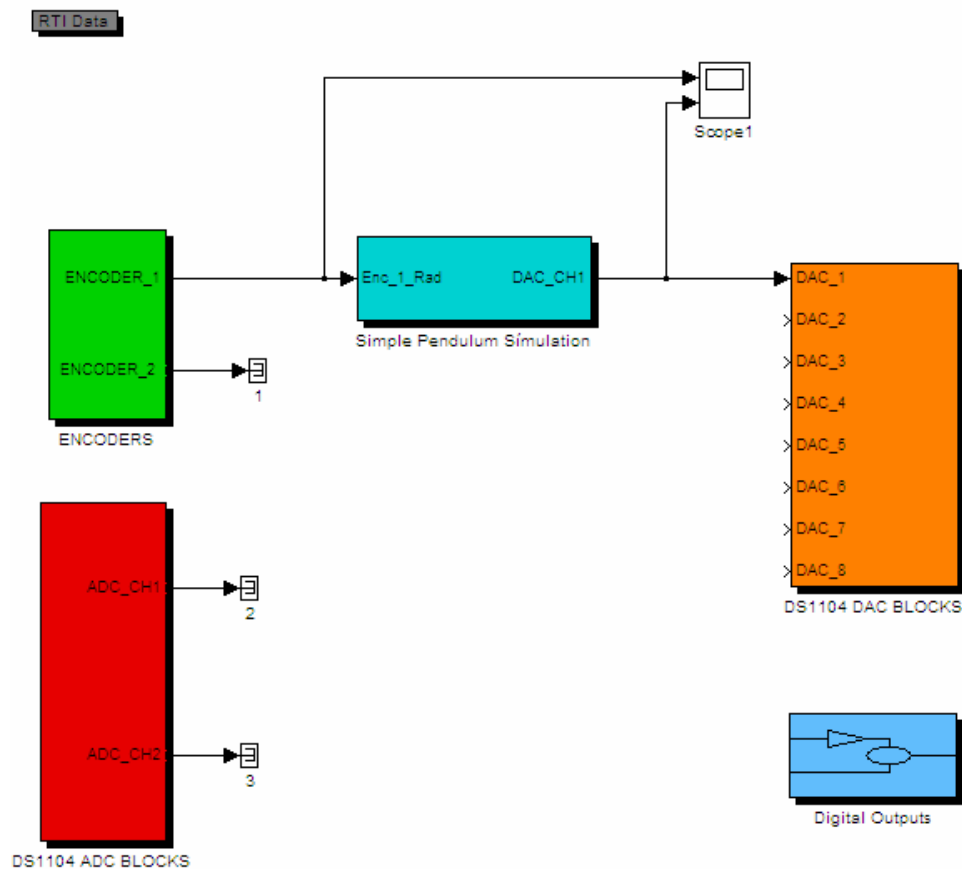
Figure 6.3: Simple Pendulum Model designed in MATLAB / Simulink
