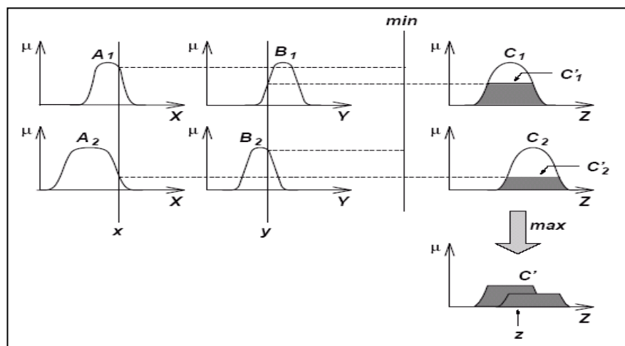
Figure 2.5 : Max-min composition.
