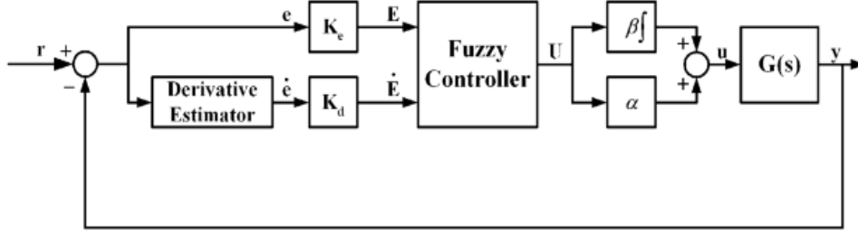
Figure 2.10 : Closed-loop control structure for PID-type FLC.
