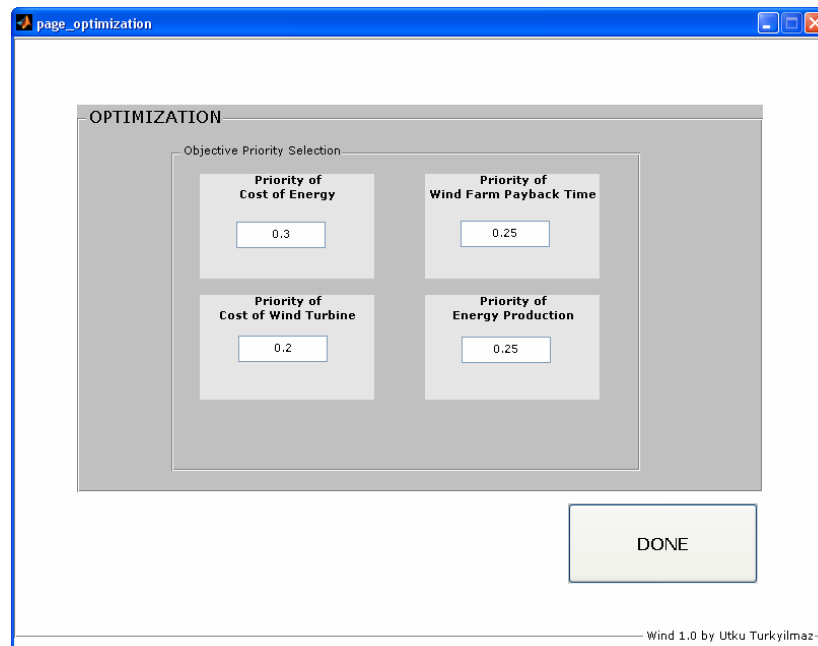
Figure 4.7: Optimization Tab
