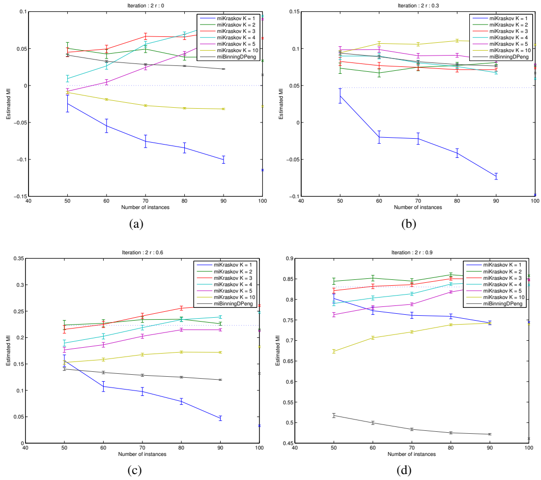
Figure 4.10: Subset selection - Experiment 2
