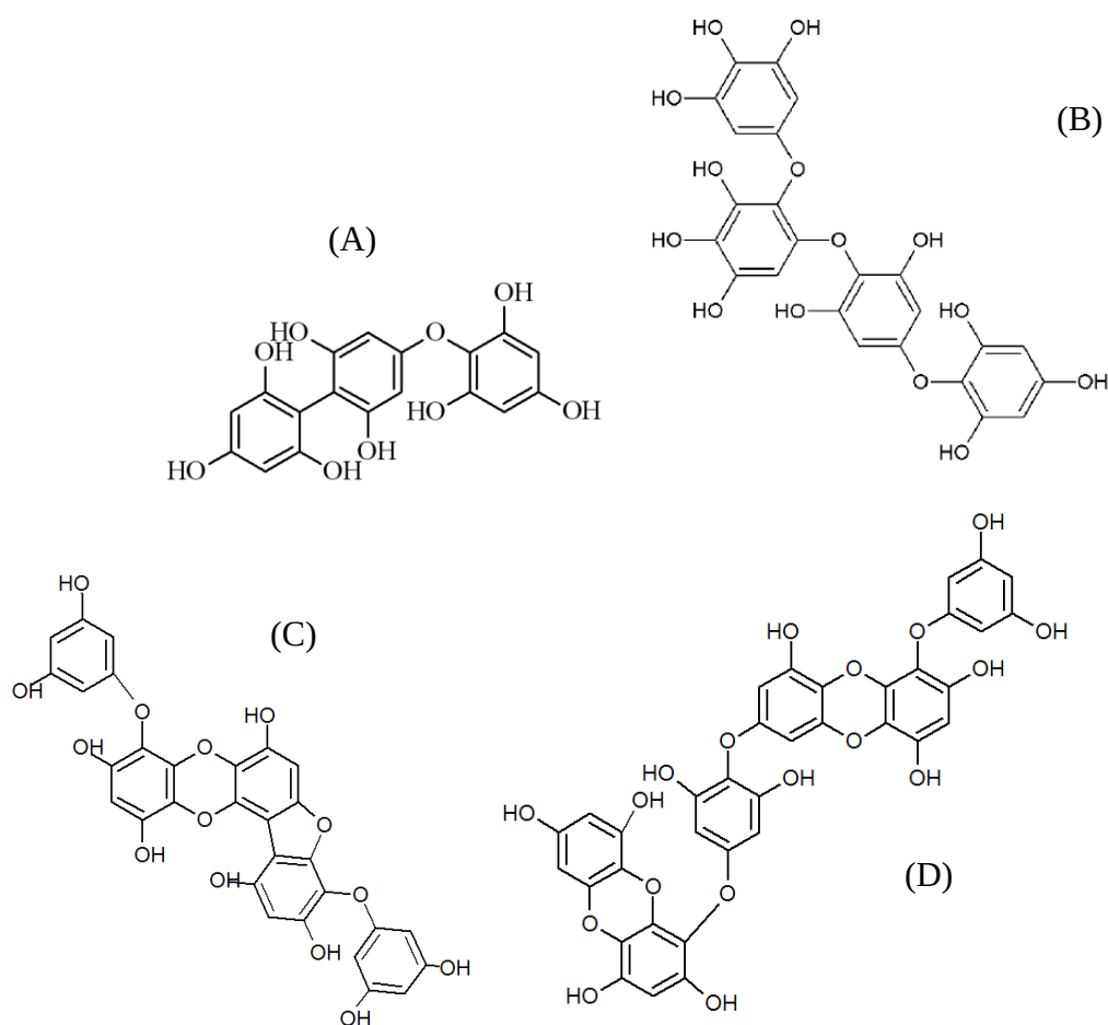
Figure 1.2: Some of the phlorotannin's molecular structures (A) Fucophloroethol A, C_{18}H_{14}O_9 , MW: 374.29 g/mol (Ferreres et al, 2012; Liu and Gu, 2012), (B) Tetrafuhalol A, C_{24}H_{18}O_{14} , MW: 530 (Koivikko, 2008), (C) Phlorofucofuroeckol A, C_{30}H_{18}O_{14} , MW: 602.45 g/mol (Li et al, 2011), (D) dieckol, C_{36}H_{22}O_{18} , MW: 742.52 g/mol (Li et al, 2011).
