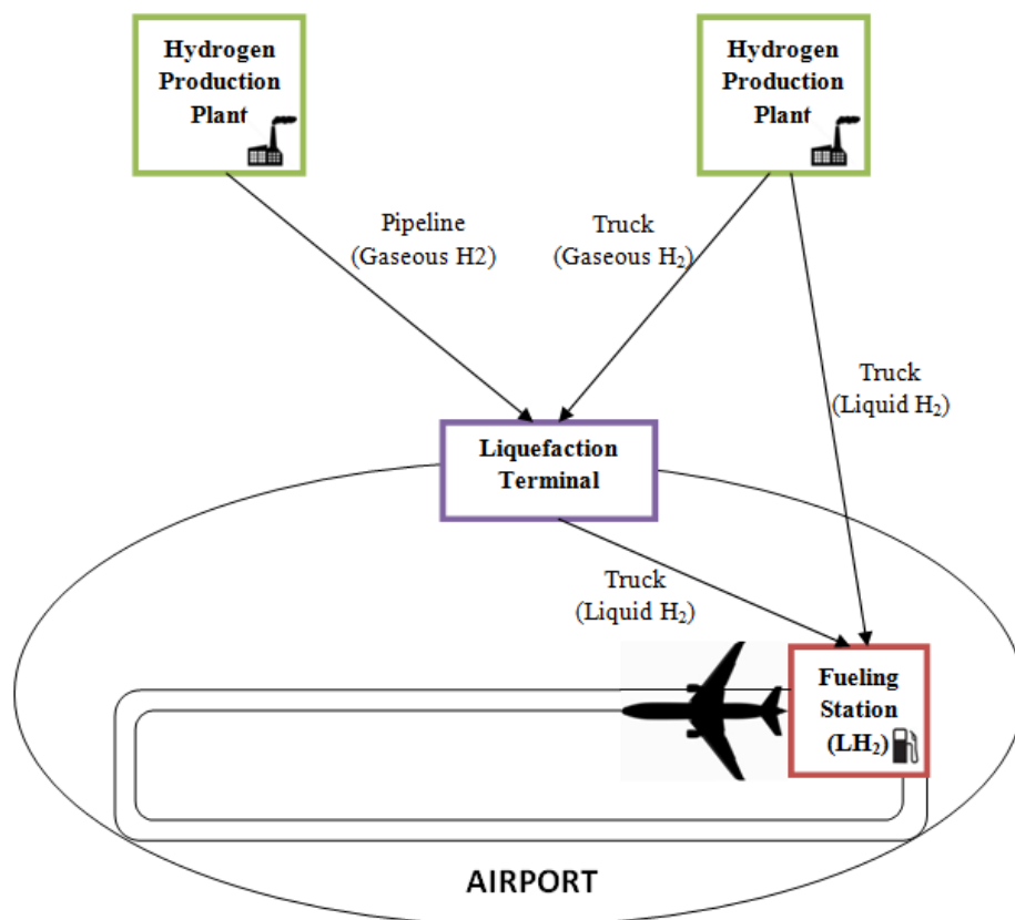
Figure 4.1: Hydrogen delivery infrastructure.
