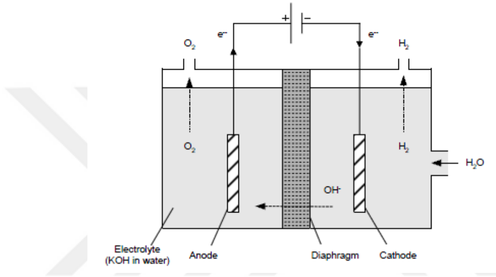
Figure 2.4: Alkaline electrolysis for hydrogen production (Gül, 2008).
