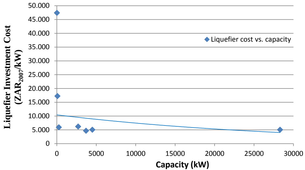
Figure 5.11: Liquefier investment cost by capacity (Amos, 1998).
