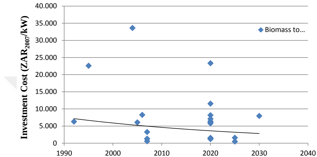
Figure 3.11: Investment costs of hydrogen production from biomass gasification.
