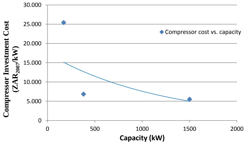
Figure 5.10: Compressor investment cost by capacity (Amos, 1998).
