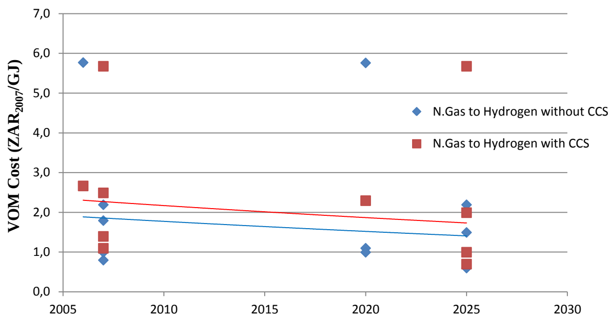
Figure B 13: Variable operation & maintenance costs of hydrogen production from natural gas reforming.
