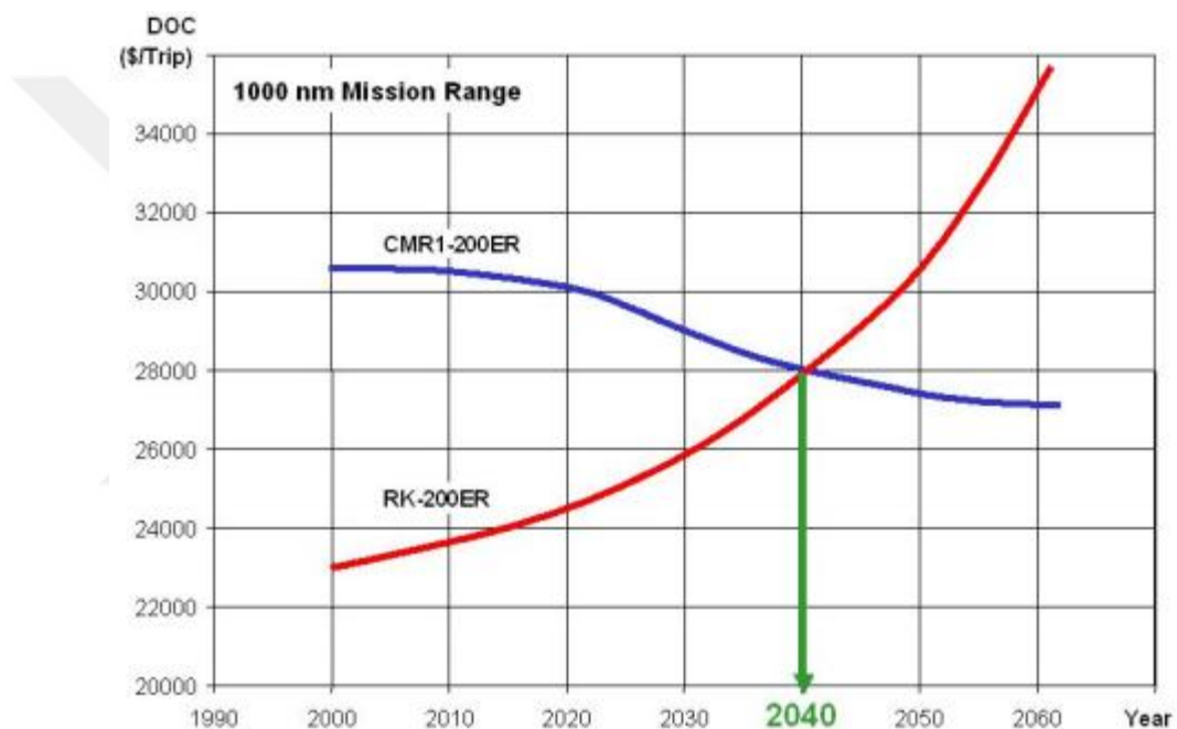
Figure 7.2: Break-even point of DOC (Direct operating cost) for CMR (Cryoplane Medium Range) and RK (Reference a/c Kerosene) (Westenberger, 2007a).
