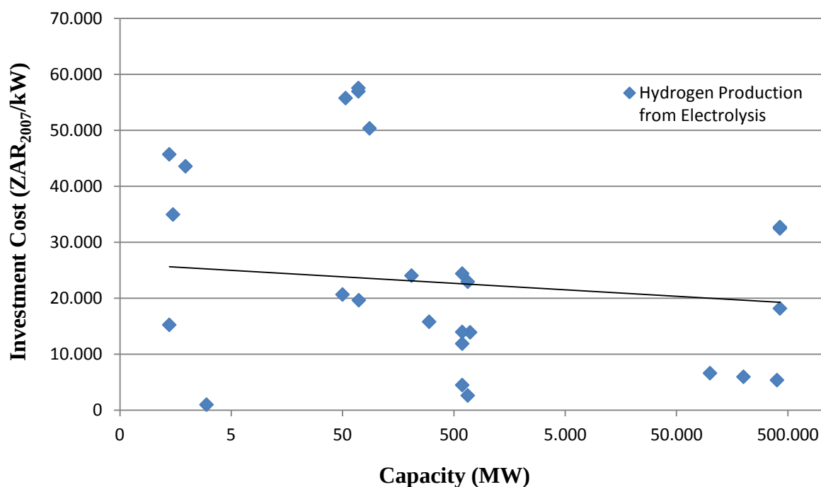
Figure B 26: Investment costs of hydrogen production from electrolysis depending on plant capacity.
