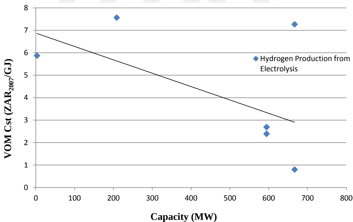
Figure B 30: Variable operation & maintenance costs of hydrogen production from electrolysis gasification depending on plant capacity.
