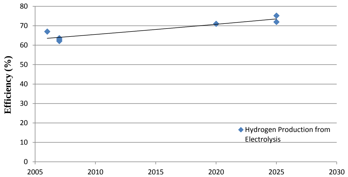
Figure B 31: Efficiency of hydrogen production from electrolysis.
