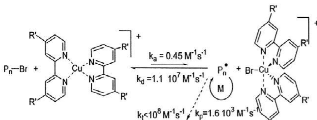
Figure 2.16: k_{\text{active}} and k_{\text{dactive}} of ATRP [68].
