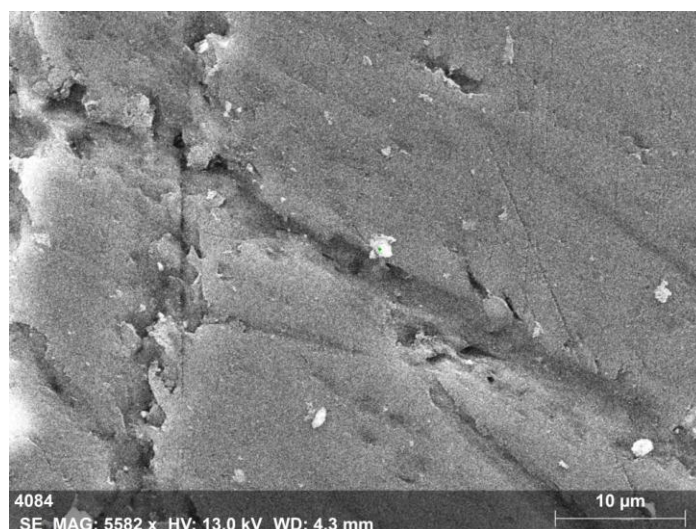
Figure 5.20: Image of EDX applied surface of PMMA with 10 (wt.%) borax.
