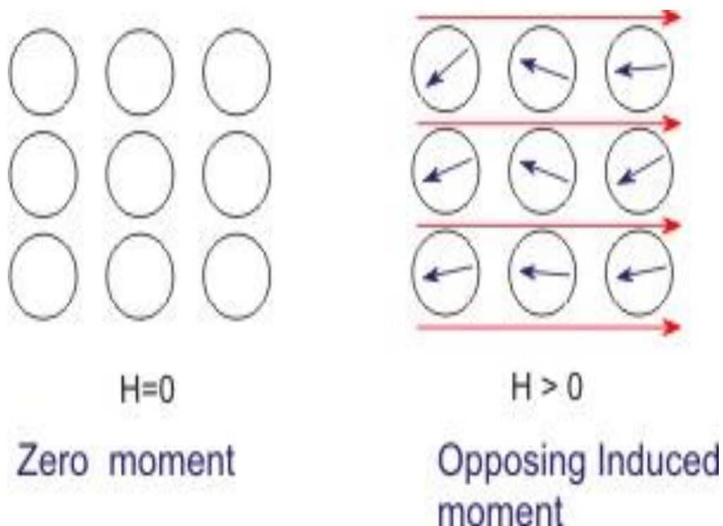
Figure 2.25. Behavior of diamagnetic materials against external magnetic field [93].
