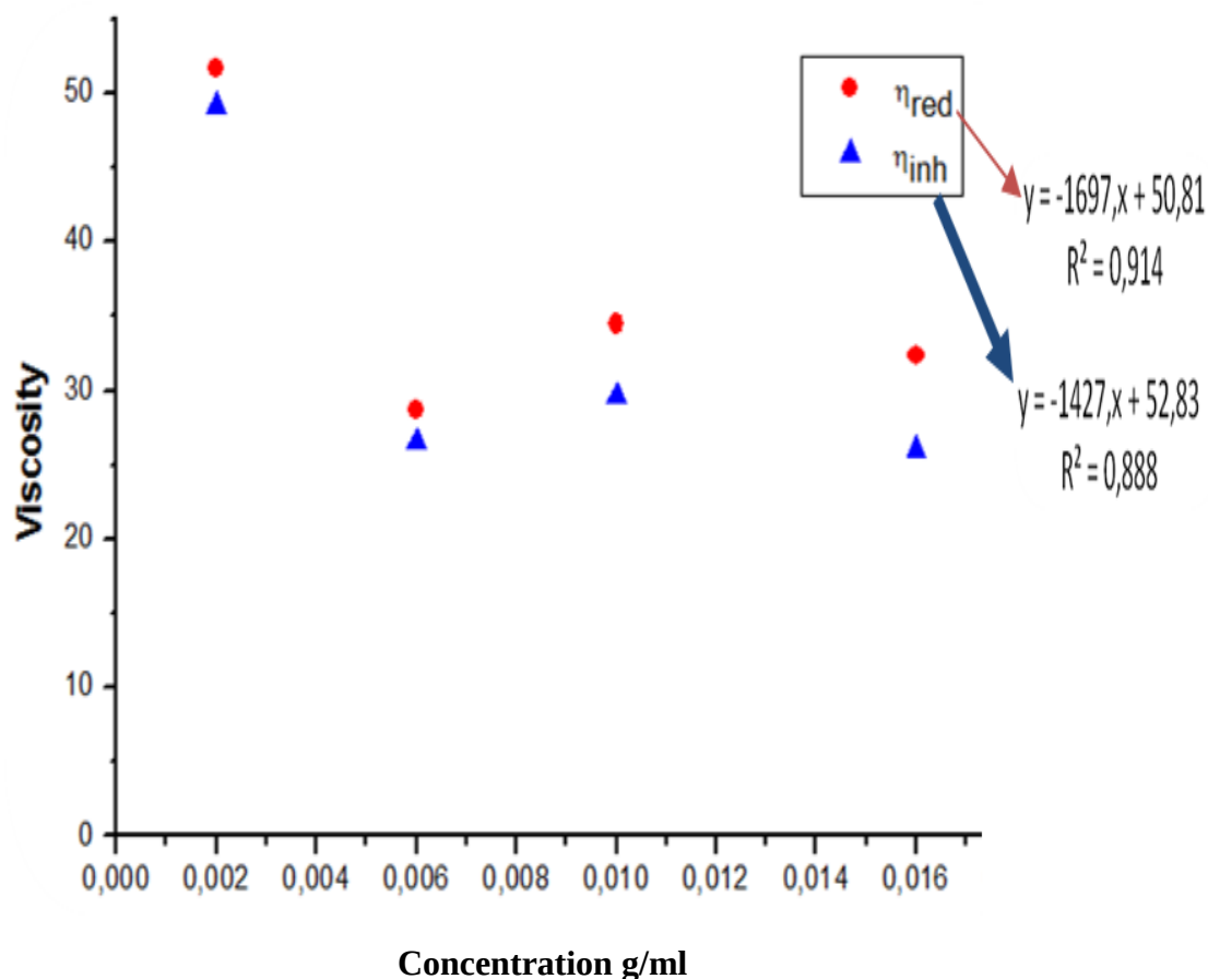
Figure 5.2: Intrinsic viscosity of base PMMA.
