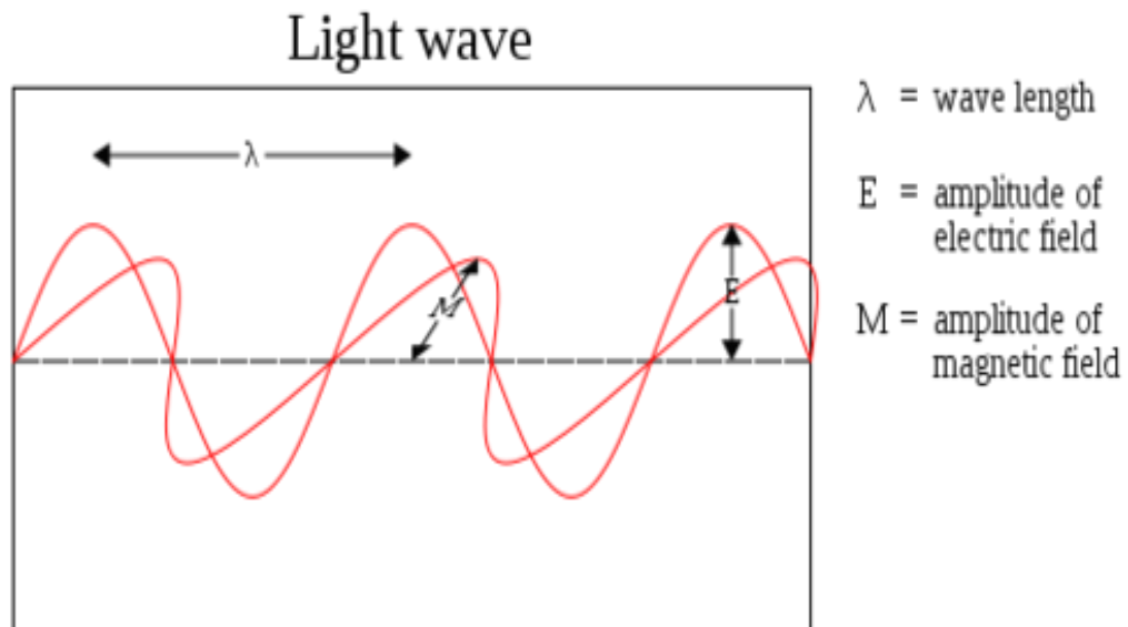
Figure 2.31. E, M and distance of electromagnetic wave [100].
