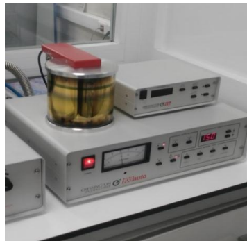
Figure 4.15: The process of coating the surfaces of samples with gold and then vacuuming of PMMA's.
