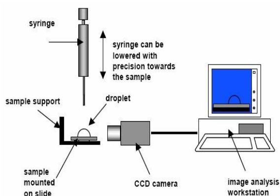
Figure 3.12: Components of the device of static contact angle measurement [163].
