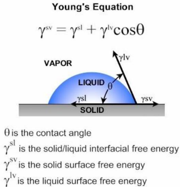
Figure 3.9: Young-Dupre Equation [155].
