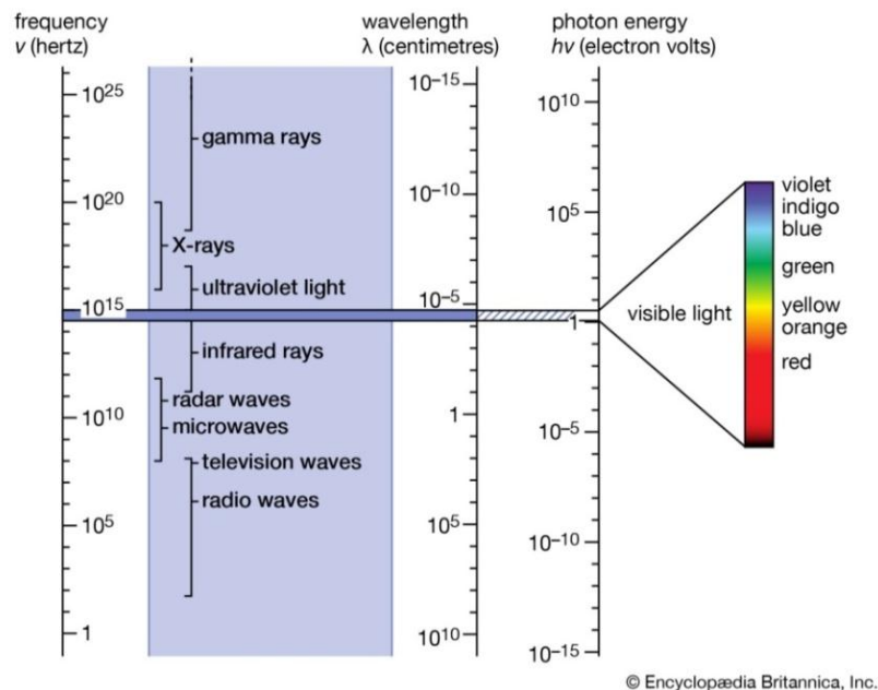
Figure 2.32: Schematic representation of the electromagnetic spectrum with frequency and wavelength [101].
