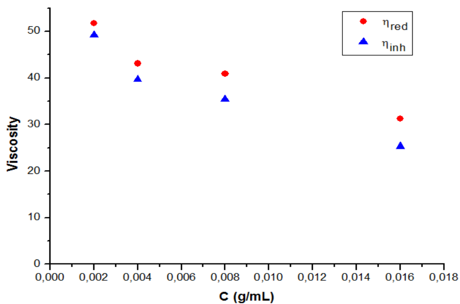
Figure 5.3: Intrinsic viscosity of PMMA 5 wt.% borax.
