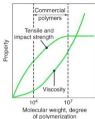
Figure 3.4: Relationship between viscosity and mechanical properties [141].
