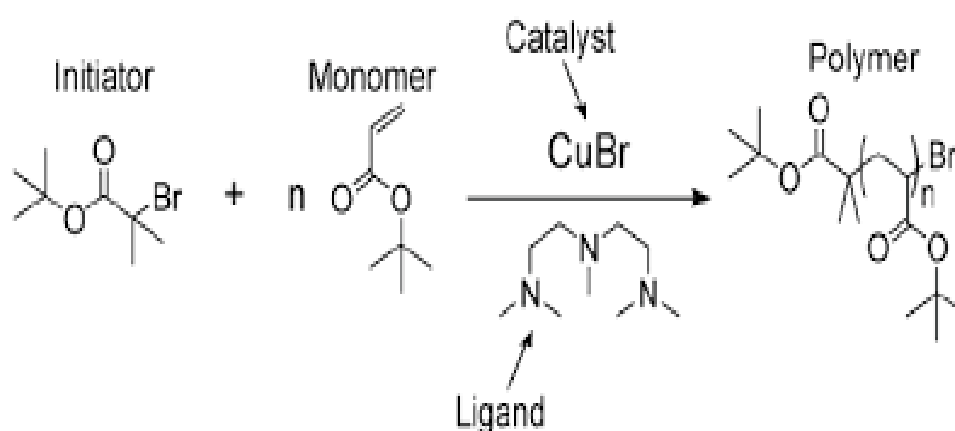
Figure 2.17: Components of ATRP [69].
