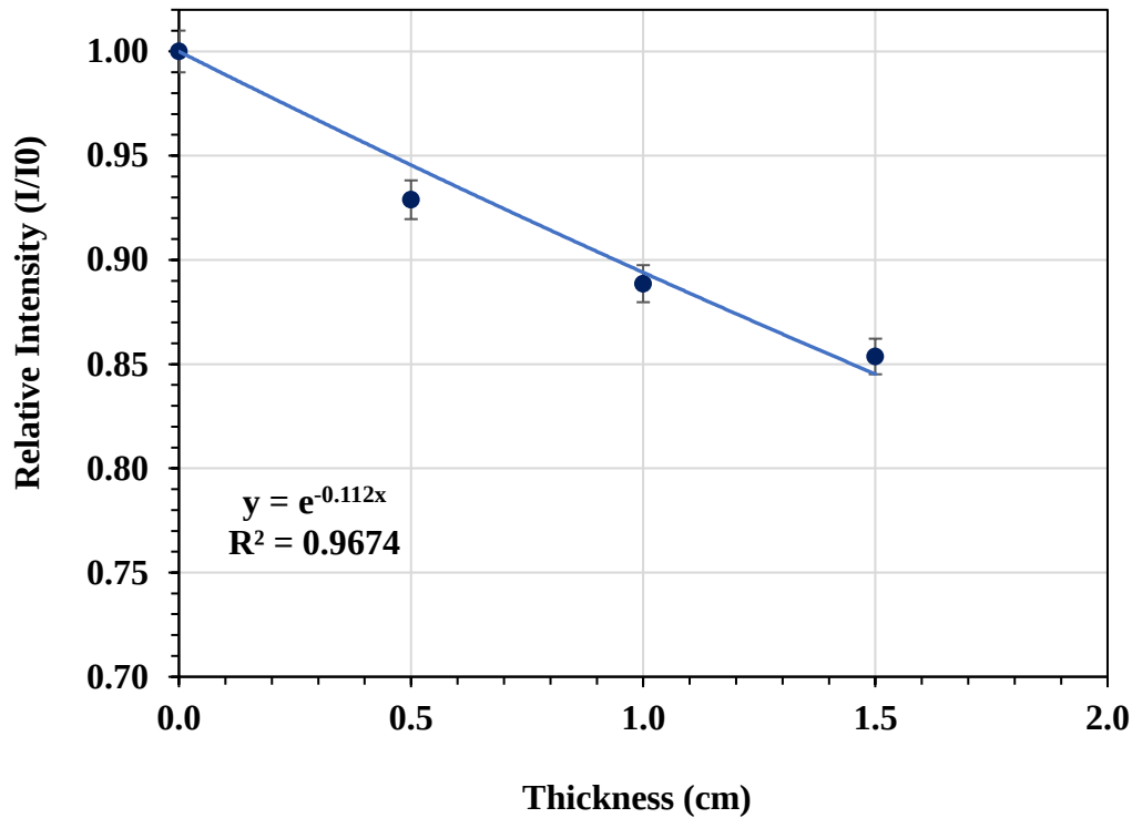
Figure 4.1 : Graph of relative intensity-thickness for pure PMMA using gamma source (Cs-137).
