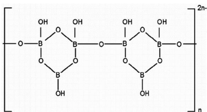
Figure 1.4 : Chemical structure of colemanite.
