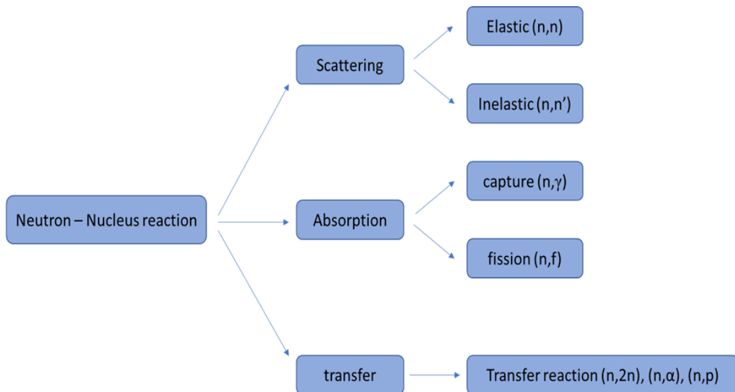
Figure 2.10 : Neutron-Nucleus interactions.
