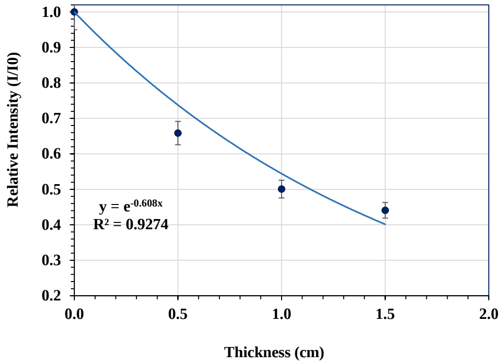
Figure 4.20 : Graph of relative intensity-thickness for PMMA/Colemanite 40 % samples using Pu-Be neutron source.
