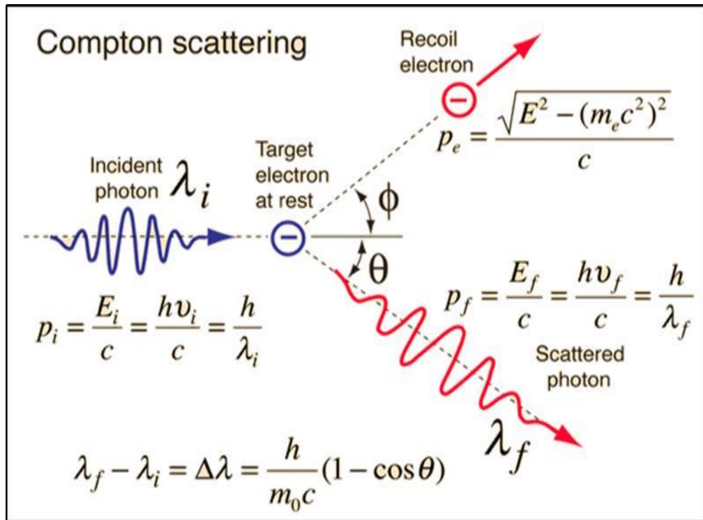
Figure 2.8 : Compton scattering.
