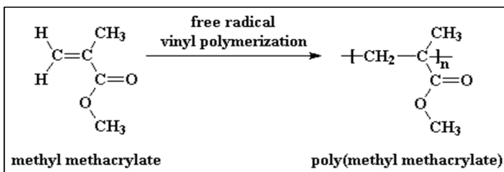
Figure 1.3 : Synthesis of PMMA via radical polymerization.
