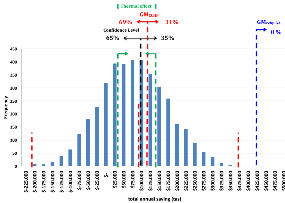
Figure 3.17 : Distribution function of tas.
