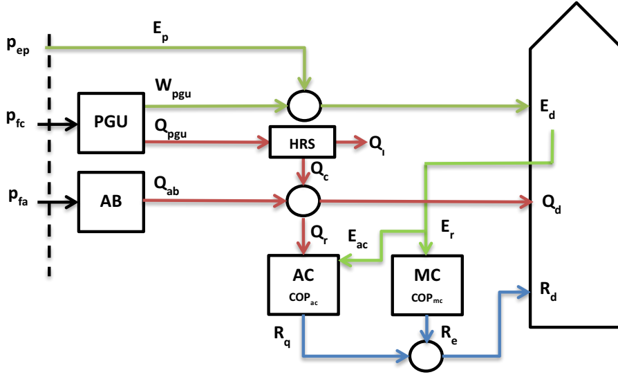
Figure 2.1 : CCHP System.
