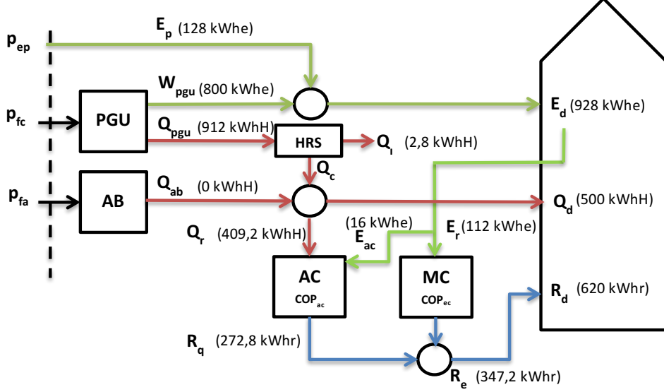
Figure 3.7 : CCHP with Optimum Load Distribution.
