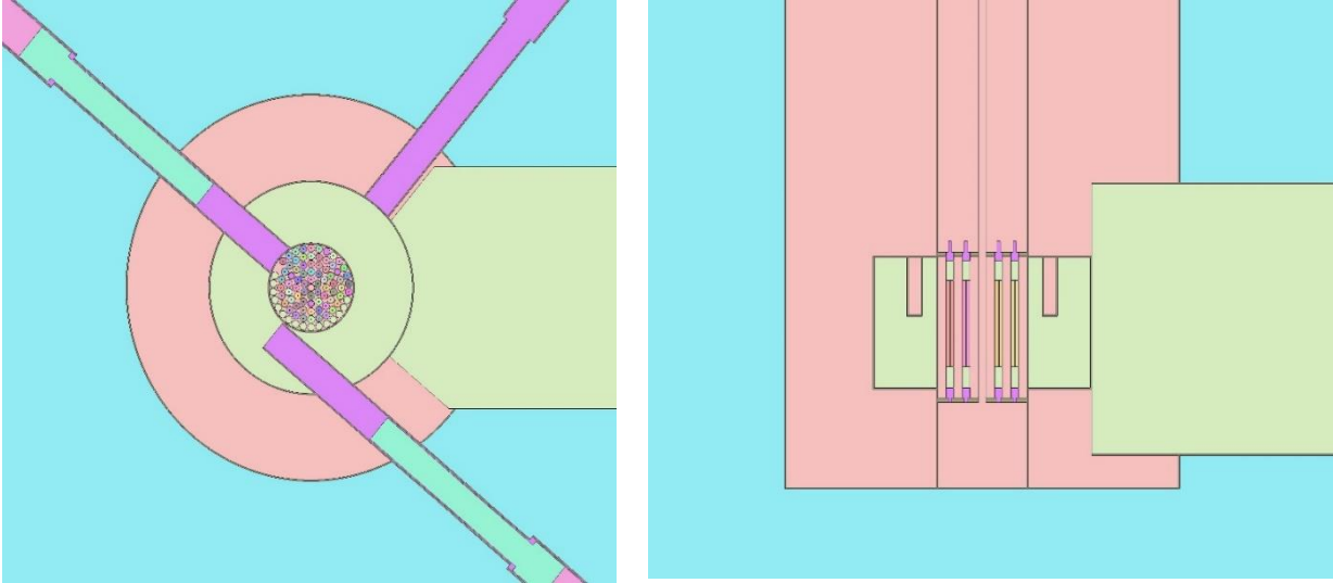
Figure 3.1 : Cross-sectional views radial (left) and axial (right) of the neutronic model for fresh fuel configuration.
