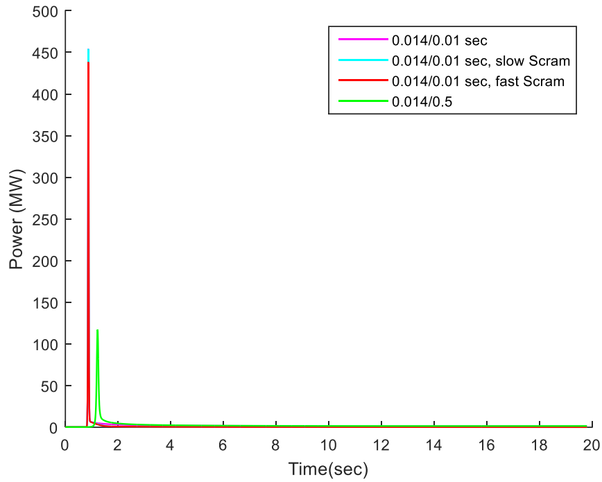
Figure 4.6 : Power vs time.
