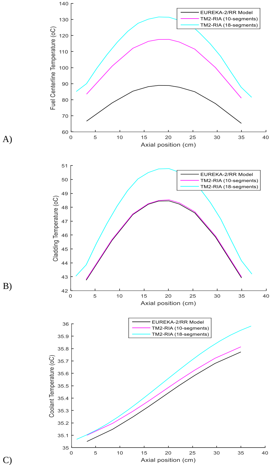
Figure 4.12 : Axial temperature profiles; A) fuel centerline, B) cladding surface, and C) coolant in hot channel. At steady-state (0.25 MW) based on the code, size and number of control volumes applied.
