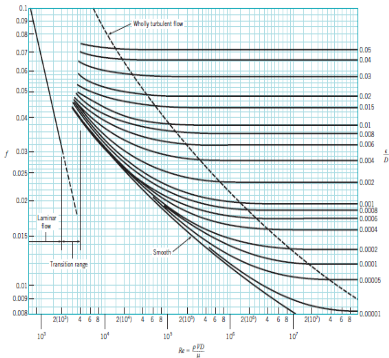
Figure C.1 : Friction factor as a function of Reynolds number and relative roughness for round pipes [55].
