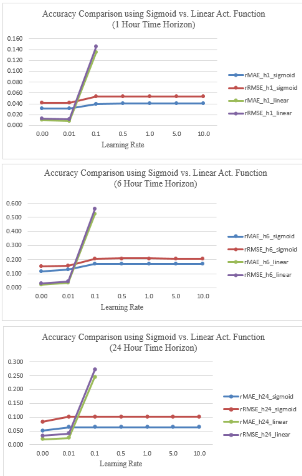
Figure 5.7: Sigmoid vs. Linear Activation Function Comparison.
