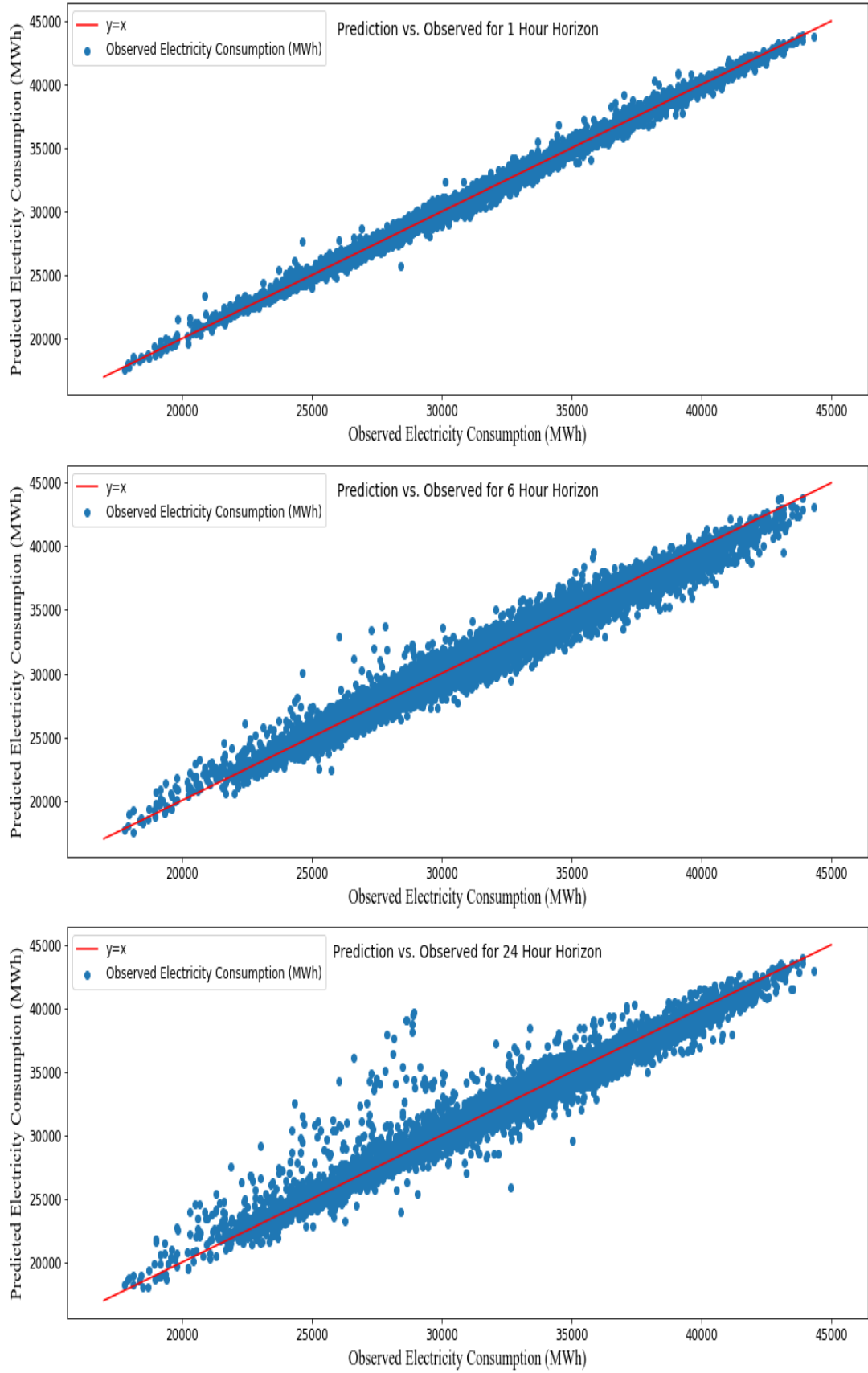
Figure 5.6: Predicted vs. Observed Electricity Load (MWh) for [220,165,220] with revised parameters.
