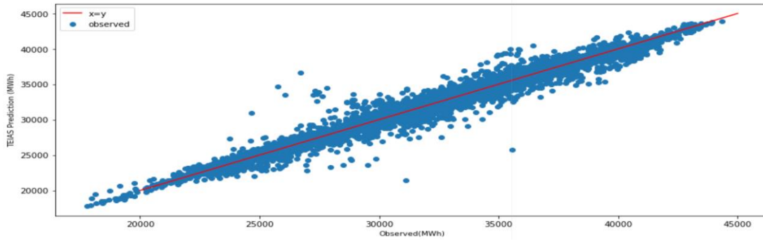
Figure 5.9: TEIAS Prediction vs Observed Electricity Load.
