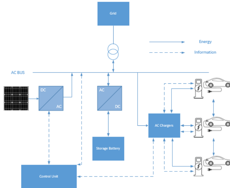
Figure 2.2 : General overview of Vehicle-to-Grid system.
