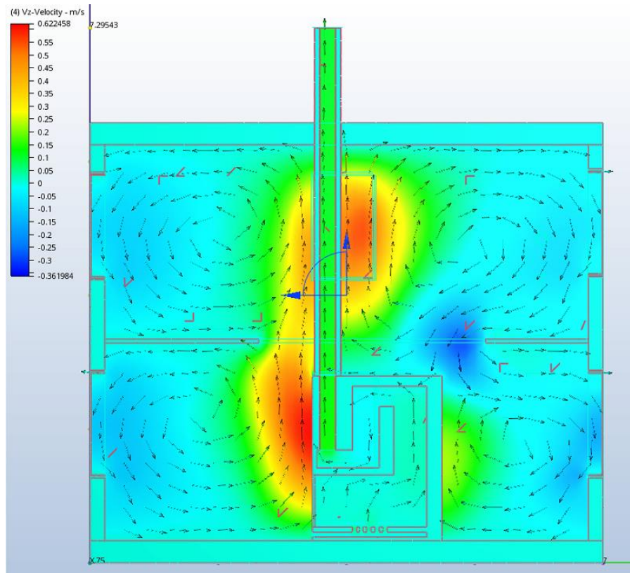
Figure 4.14 : Z direction air velocity circulation by a section view for Russian stove.
