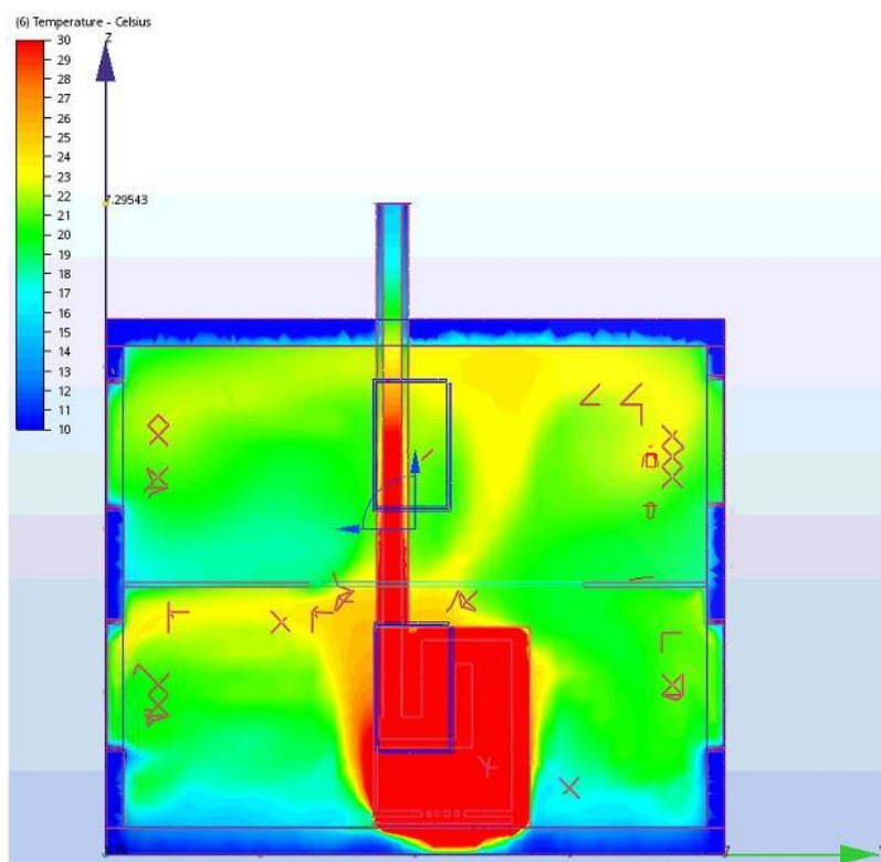
Figure 4.3 : Temperature gradient after heating period.
