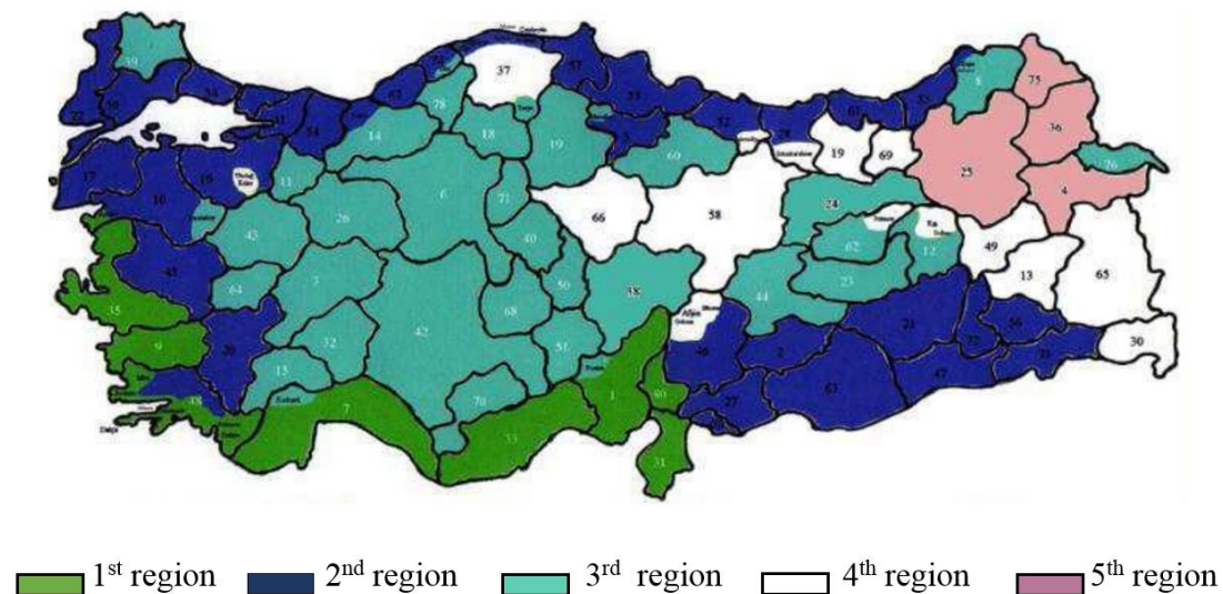
Figure 2.4 : The regional classification of Turkey (Turkish Standardization Institute, 2013).
