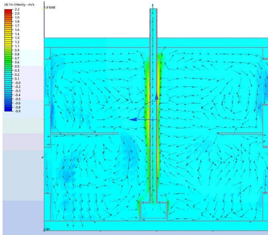
Figure 4.16 : Z direction air velocity circulation by a section view steel casting stove case.
