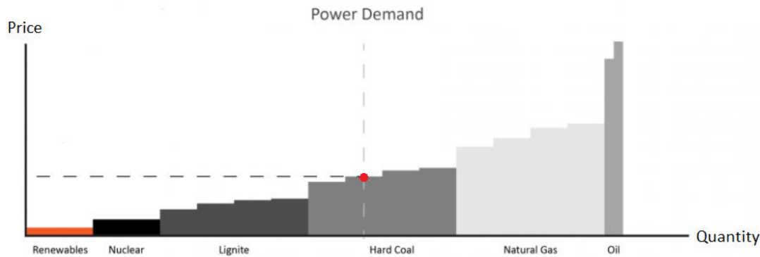
Figure 2.4 : Typical merit-order curve [13].
