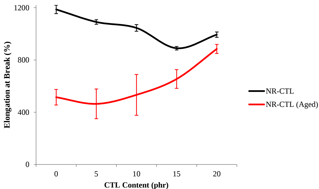
Figure 4.23: Before and after aging elongation values of NR-CTL composites
