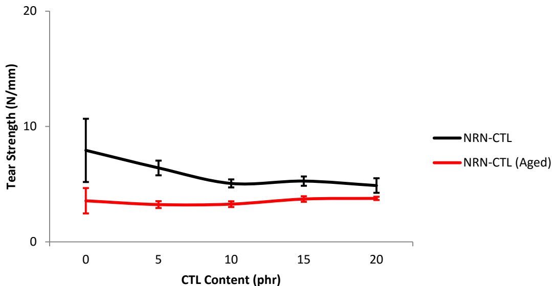
Figure 4.36 (continued): Before and after aging tear strength values a) NR-CTL and b) NRN-CTL composites
