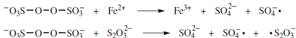
Figure 2.8 : Redox initiation by inorganic reductants and oxidants
