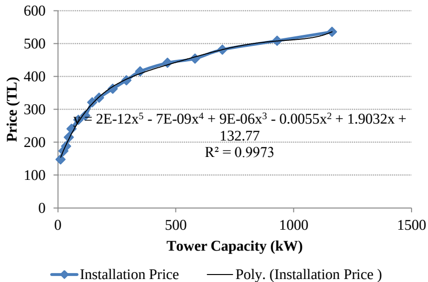
Figure 5.16 : Cooling tower installation price curve.
