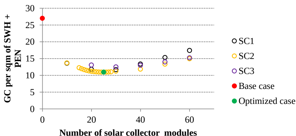
Figure 5.58 : Optimization results with each solar collector type within feasible region obtained with Antalya case.
