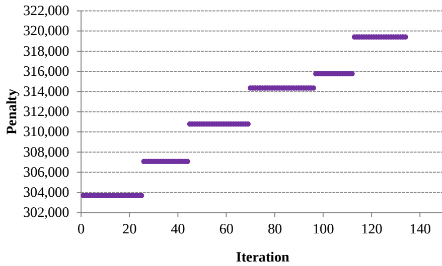
Figure D.21: Penalty function values of the payback period for Istanbul case.
