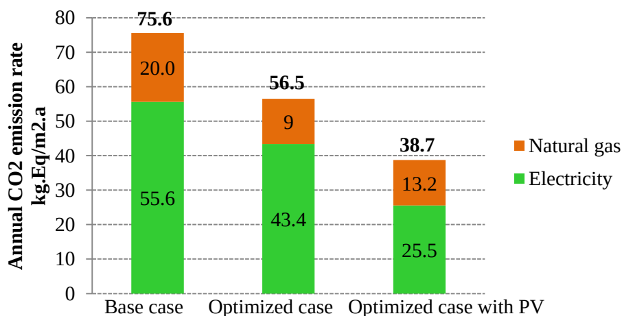
Figure 5.42 : Comparison of annual CO 2 emission rate after PV integration obtained with Ankara case.
