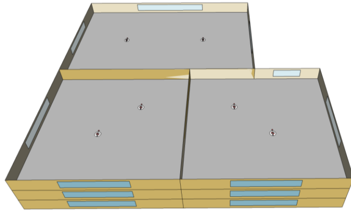
Figure 5.8 : Location of daylighting reference points.
