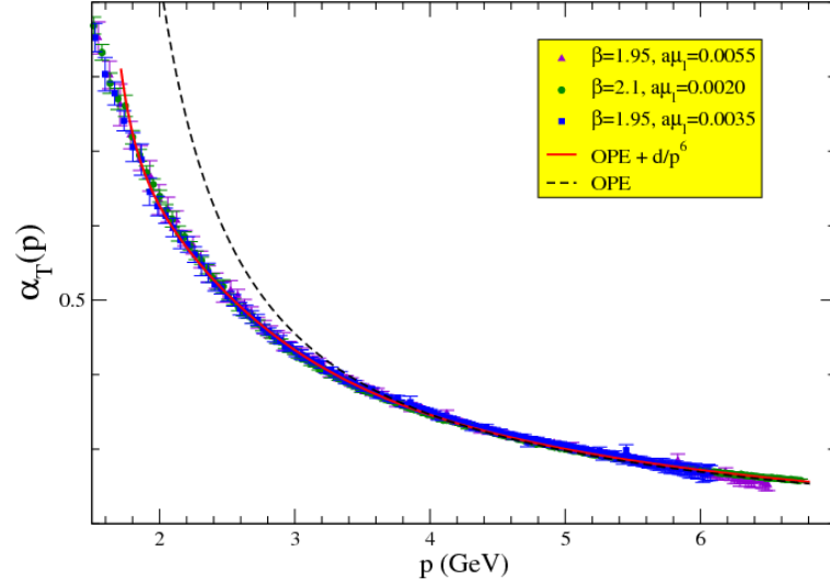
Figure 1.3 : Significant Lattice QCD results of the running coupling constant [4].
