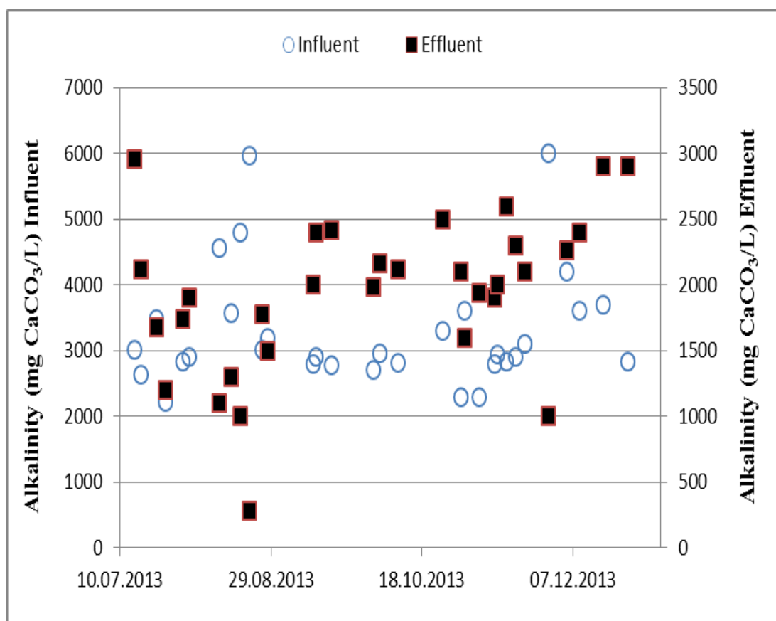
Figure 4.16 : Alkalinity changes in the effluent in the ASB reactor treating Slurry-II.
