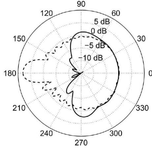
Figure 3.11 : Normalized magnitude of the interior field ( |E|/|E^i| ) on the surface of Eaton lens (solid line), and Luneburg lens (dashed line), induced by a plane wave travelling in the negative z-direction.
