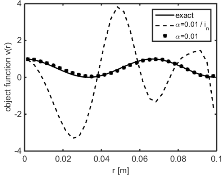
Figure 2.29 : Exact and reconstructed values of the object function for a sphere described by b(r)/b_0 = 1.5 + 0.5\cos(3\pi r/a) with \alpha = 0.01/i_n and \alpha = 0.01 .
