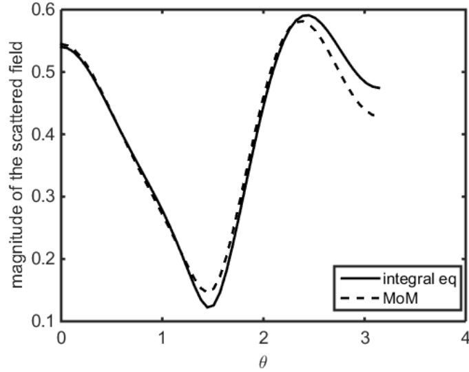
Figure 2.13 : The field scattered by the sphere described by b(r)/b_0 = 5 + 5(r/a) in the case of plane wave excitation, calculated by the integral equations and MoM. Measurement region: r_{obs} = 0.2m , \theta_{obs} \in [0, \pi] , \phi_{obs} = 0 ; ( k_0 = 8\pi ).
