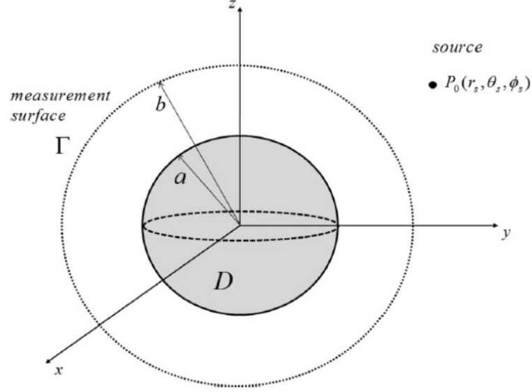
Figure 2.16 : The geometry of the inverse scattering problem.
