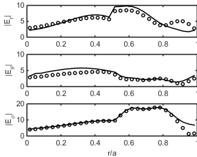
Figure 3.3 : Magnitude of the total field inside the two-layered sphere, solid line corresponds to the solution with integral equations, and circles to the dyadic Green's function ( k_0 a = 20 , N_{\max} = 25 ).
