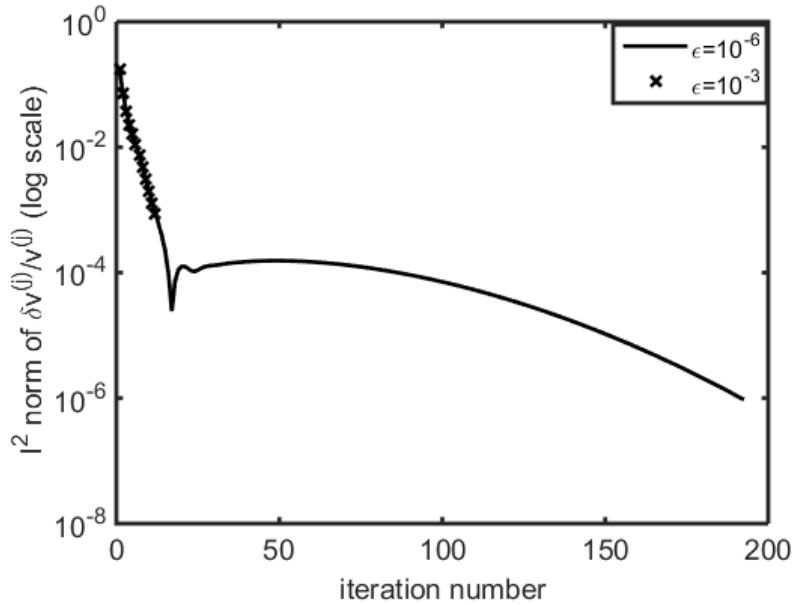
Figure 2.31 : The convergence history graph of the \ell^2 norm of \delta v^{(j)}/v^{(j)} (in logarithmic scale) for the Luneburg lens with \varepsilon = 10^{-3} and \varepsilon = 10^{-6} .
