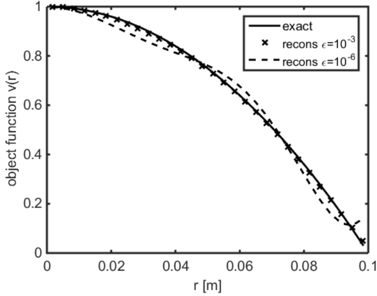
Figure 2.30 : Exact and reconstructed values of the object function for the Luneburg lens with \varepsilon = 10^{-3} and \varepsilon = 10^{-6} .
