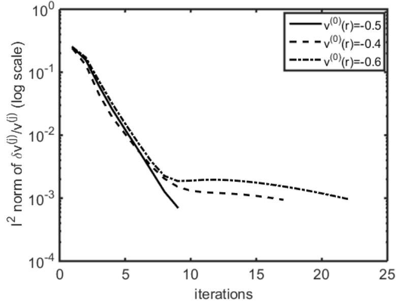
Figure 2.22 : The convergence history graph of the \ell^2 norm of \delta v^{(j)} / v^{(j)} (in log scale) for three different initial guesses v^{(0)}(r) . The sphere has a linearly varying profile described by b(r)/b_0 = 0.5 + 0.5(r/a) .
