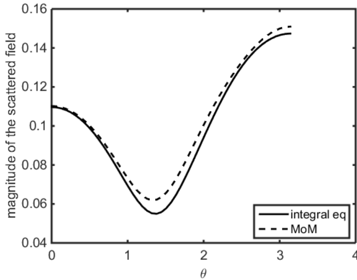
Figure 2.12 : The field scattered by the sphere described by b(r)/b_0 = 5 + 5(r/a) in the case of point source excitation, calculated by the integral equations and MoM.
