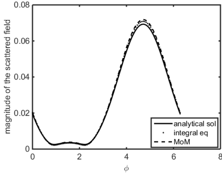
Figure 2.8 : The magnitude of field scattered by a two layered sphere, calculated by three methods. Measurement region: r_{\text{obs}} = 0.2 \text{ m} , \theta_{\text{obs}} = \pi/2 , \phi_{\text{obs}} \in [0, 2\pi] ; k_0 = 8\pi .
