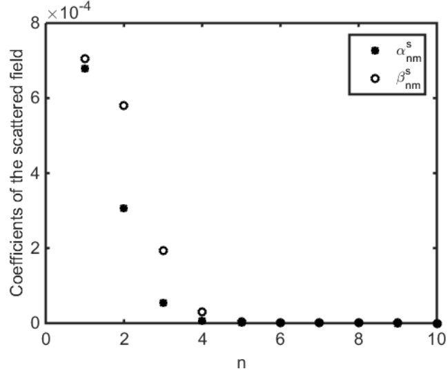
Figure 3.6 : The magnitude of the coefficients \alpha_{n1}^s(r = 300) and \beta_{n1}^s(r = 300) of the field scattered by a sphere with linearly varying profile.
