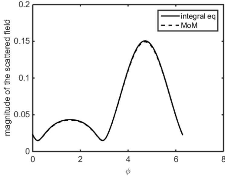
Figure 2.15 : The field scattered from the sphere of b(r)/b_0 = 1.5 + 0.5\cos(3\pi r/a) , calculated by the integral equations and MoM. Measurement region: r_{obs} = 0.2 m , \theta_{obs} = \pi/2 , \phi_{obs} \in [0, 2\pi] ; ( k_0 = 8\pi ).
